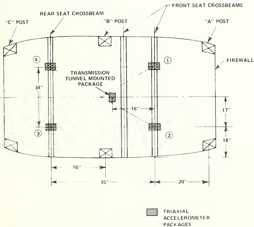
Figure A-2. Schematic Of Passenger Compartment Showing Accelerometer Locations
