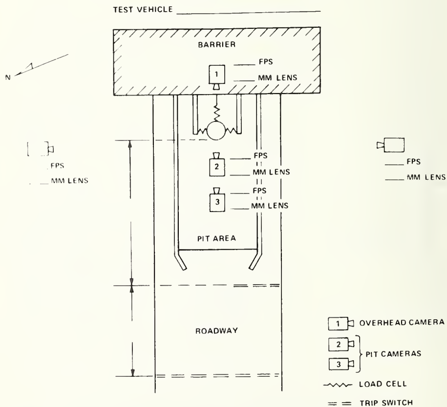
Figure A-5. Test Site Location Of Sensors And Cameras
