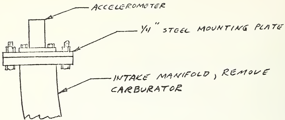
Figure A-8. Engine Accelerometer Location
