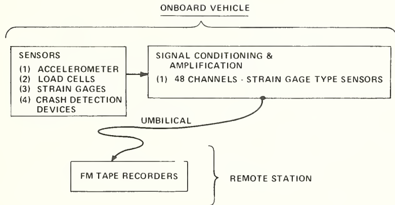
Figure A-1. Block Diagram Of Basic Data Recording System
