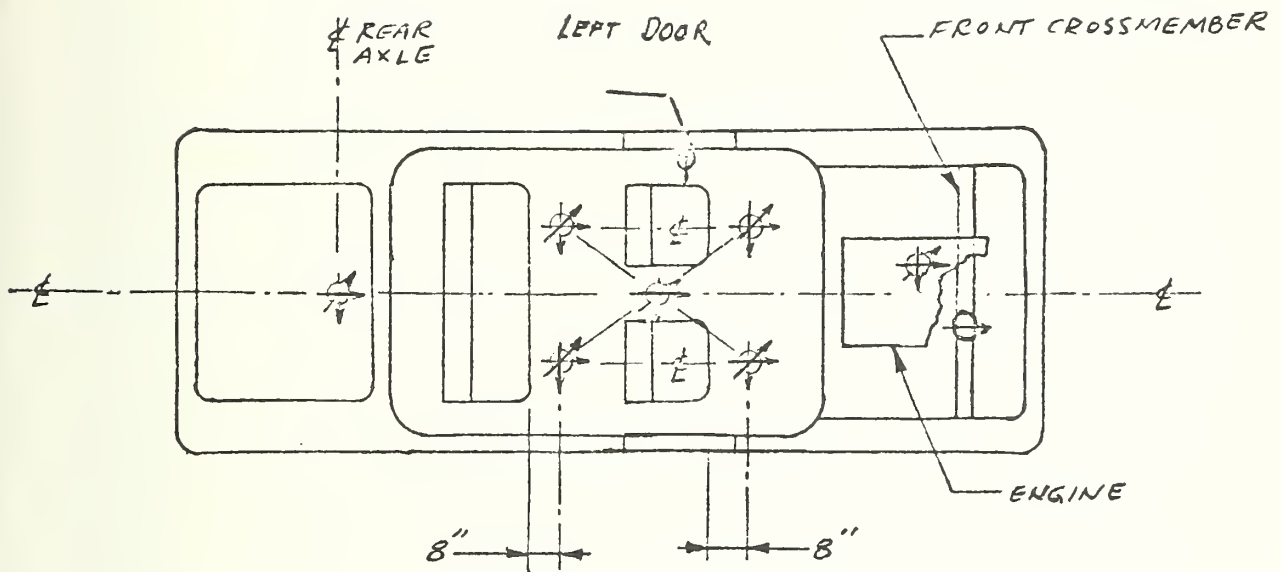
Figure A-6. Compact Car Floor Plan, Typical Accelerometer Locations
