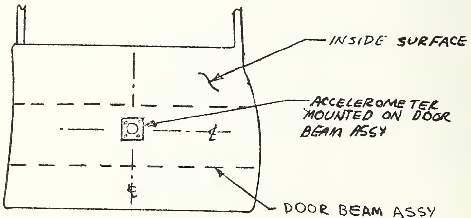
Figure A-10. Door Accelerometer Location
