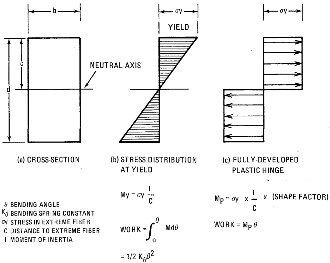
Figure 9-3. Definition of Plastic Hinges
