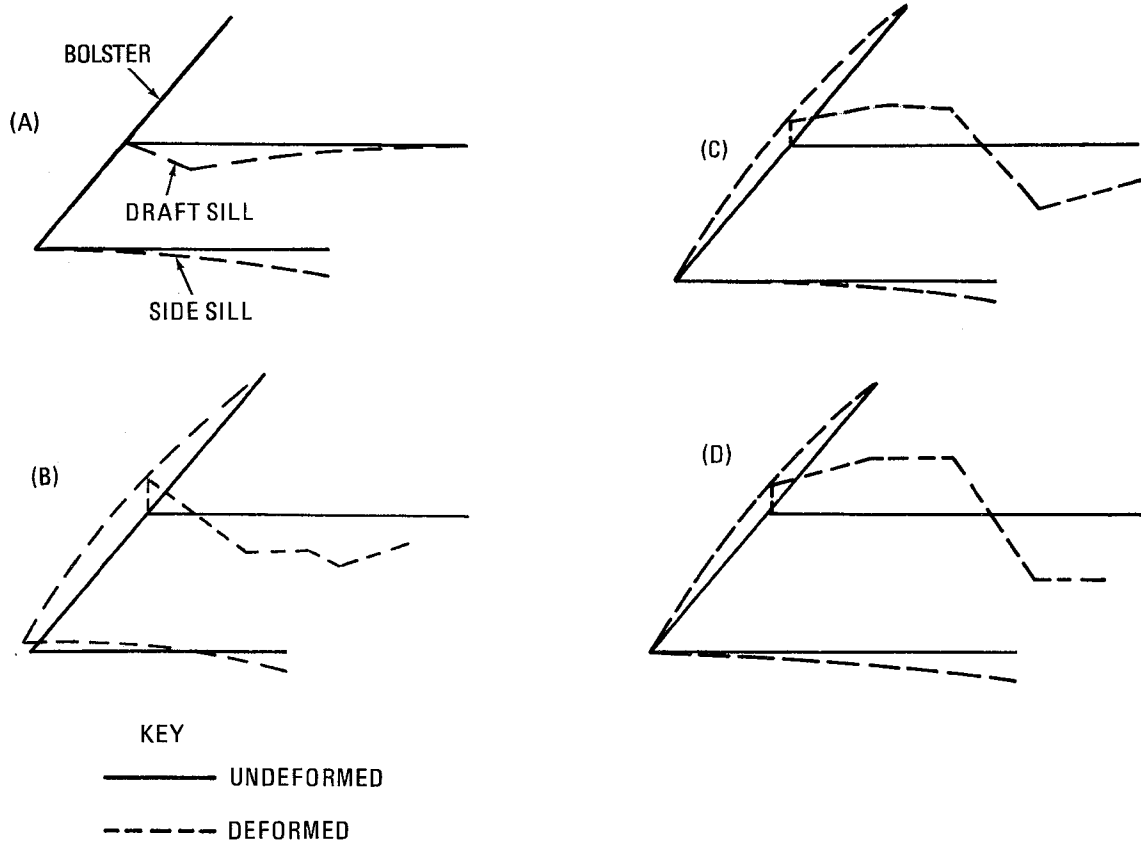
Figure 9-6. Characteristic Car End Deformations
