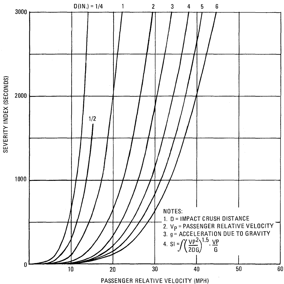
Figure 6—8. Severity Index Versus Passenger Relative Velocity for Constant Cushion Crush Distances
