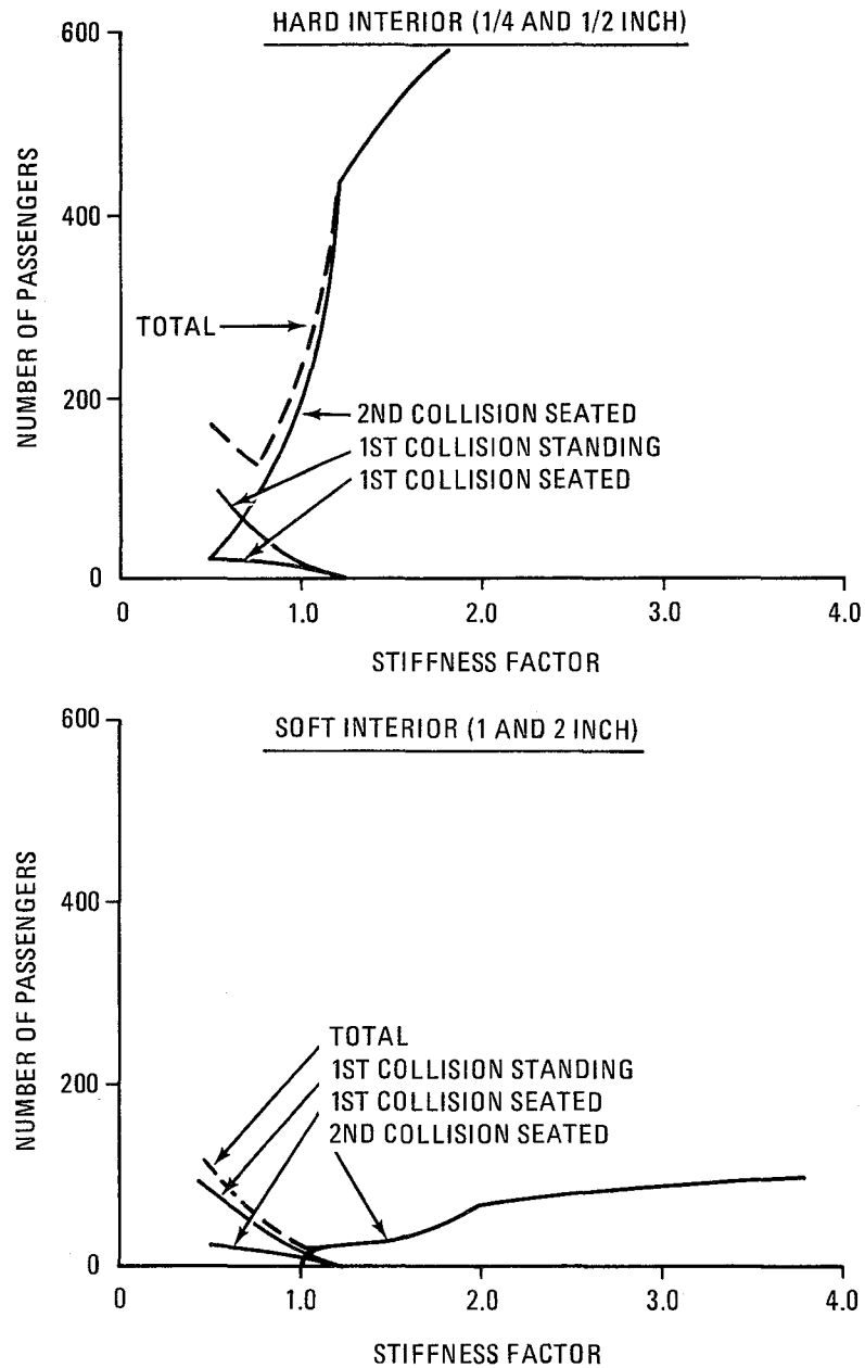
Figure 7-5. Passenger Fatality Cause for Hard and Soft Car Interiors
