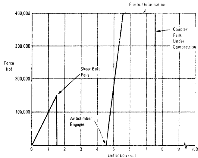
Figure 2-3. Coupler Force Deflection Characteristics
