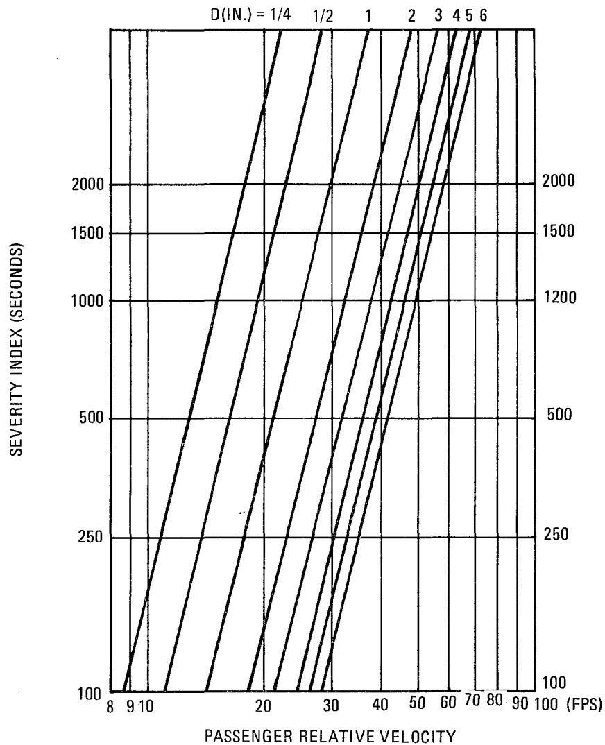
Figure 6-7. Severity Index Versus Passenger Relative Velocity for Constant Cushion Crush Distances
