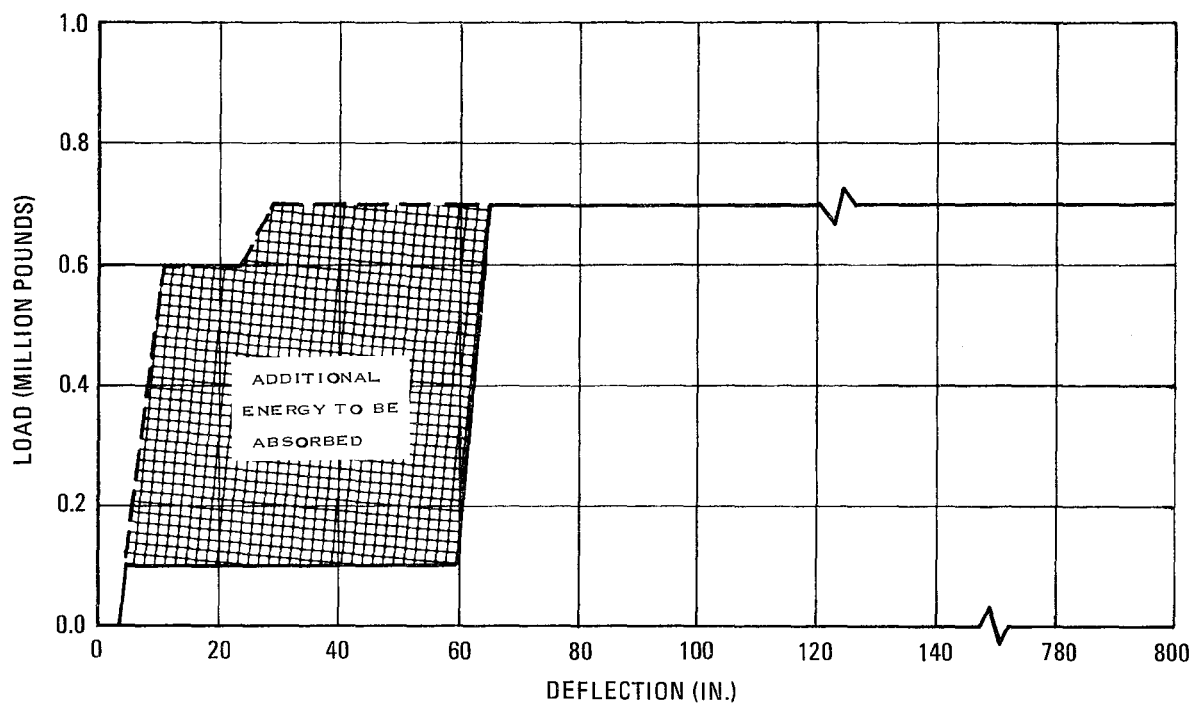
Figure 9-1. Crush Force Versus Deflection to Provide Buff Required Strength
