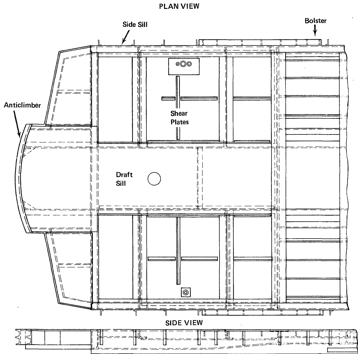
Figure 2-2. SOAC Underframe at Car End
