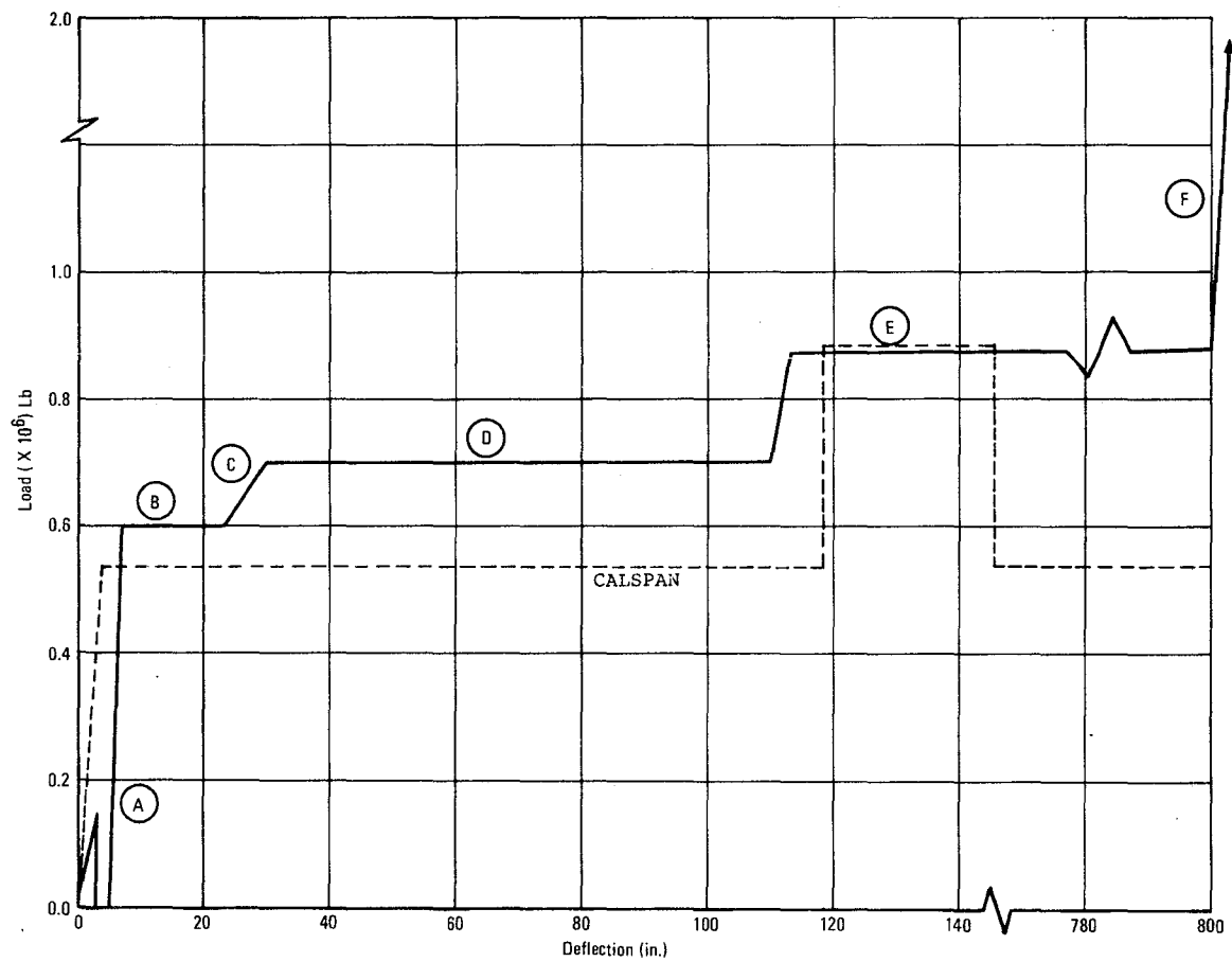
Figure 4-1. Crush Force Versus Deflection for Car Squeeze with No Overriding
