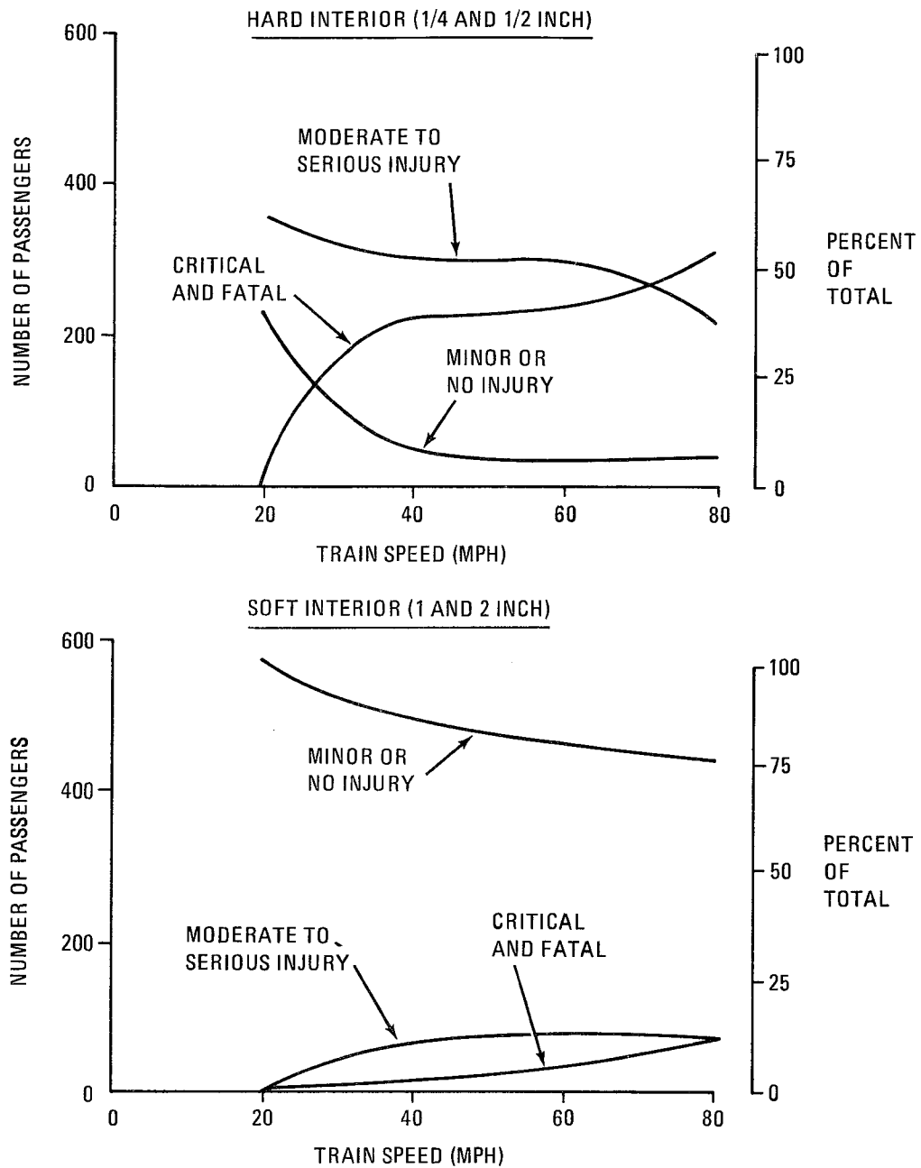
Figure 7-3. Casualties for Hard and Soft Car Interiors as a Function of Closing Velocity
