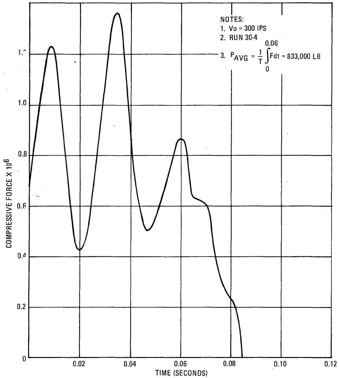
Figure 2-9. Anticlimber Contact: Axial Load in Element 4-5
