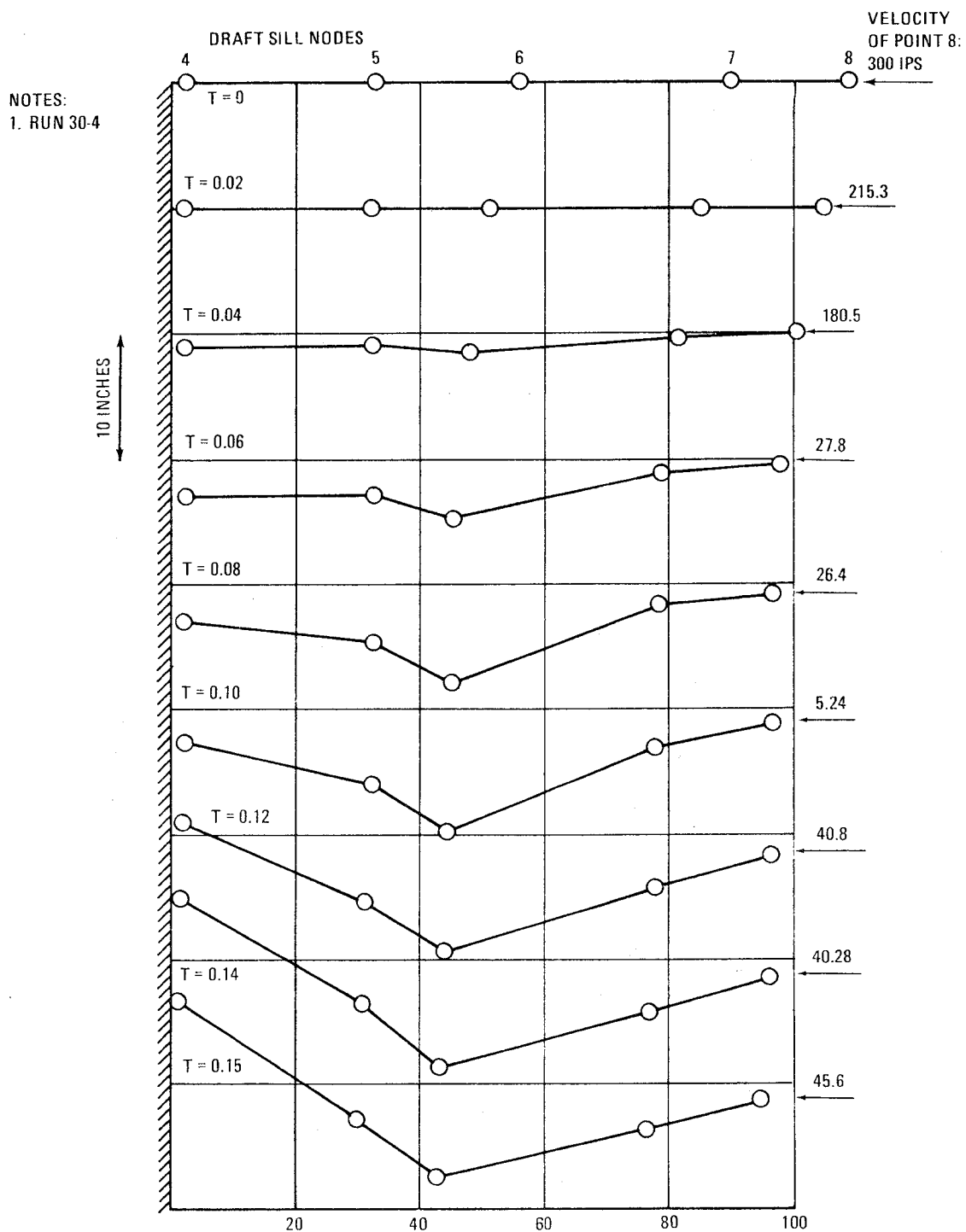
Figure 2-11. Draft Sill Deflections Versus Time
