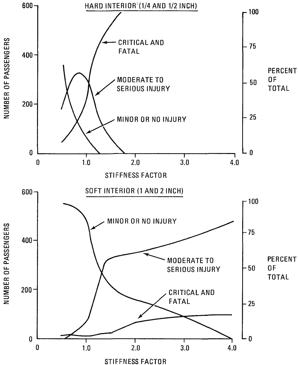
Figure 7-4. Casualties Versus Stiffness Factor for Hard and Soft Car Interiors
