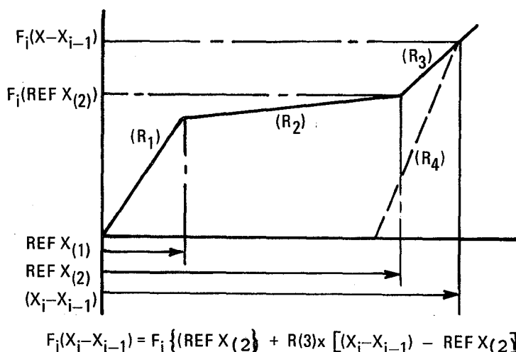
Figure 5-2. Force Value Computation
