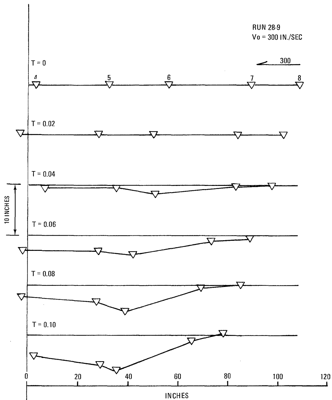
Figure 2-6. Draft Sill Deflection Coupler/Anticlimber Impact
