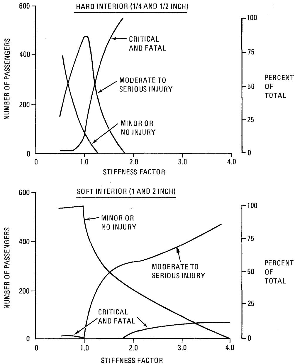
Figure 7-7. Casualties Versus Stiffness for Hard and Soft Car Interiors
