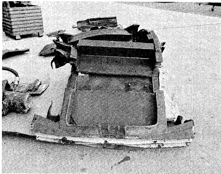
Figure 3-5. Draft Sill Anchor Plate and Plastic Hinge
