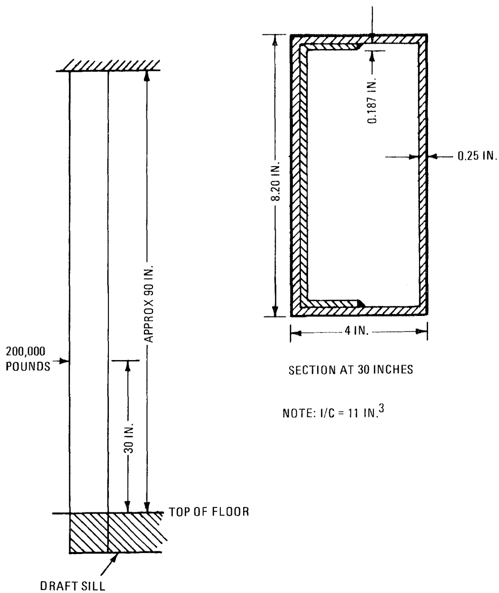
Figure 9-4. General Collision Post Arrangement
