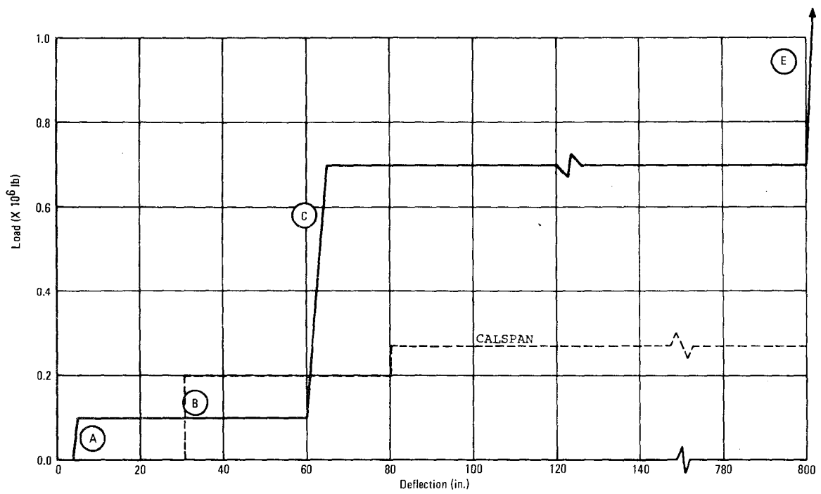
Figure 4-2. Crush Force Versus Deflection with Overriding
