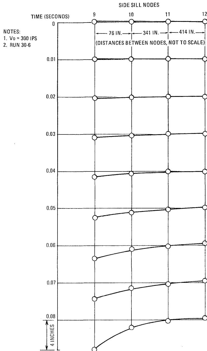
Figure 2-13. Side Sill Vertical Deflection for Coupler Impact Versus Time
