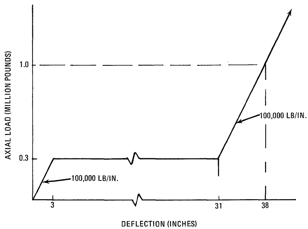
Figure 5-5. Accident Simulation Force Deflection Curve for Element 2-4.
