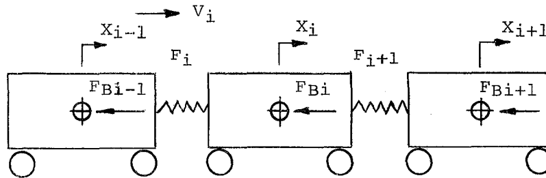
Figure 5-1. Multi-Car Consist Impact Model
