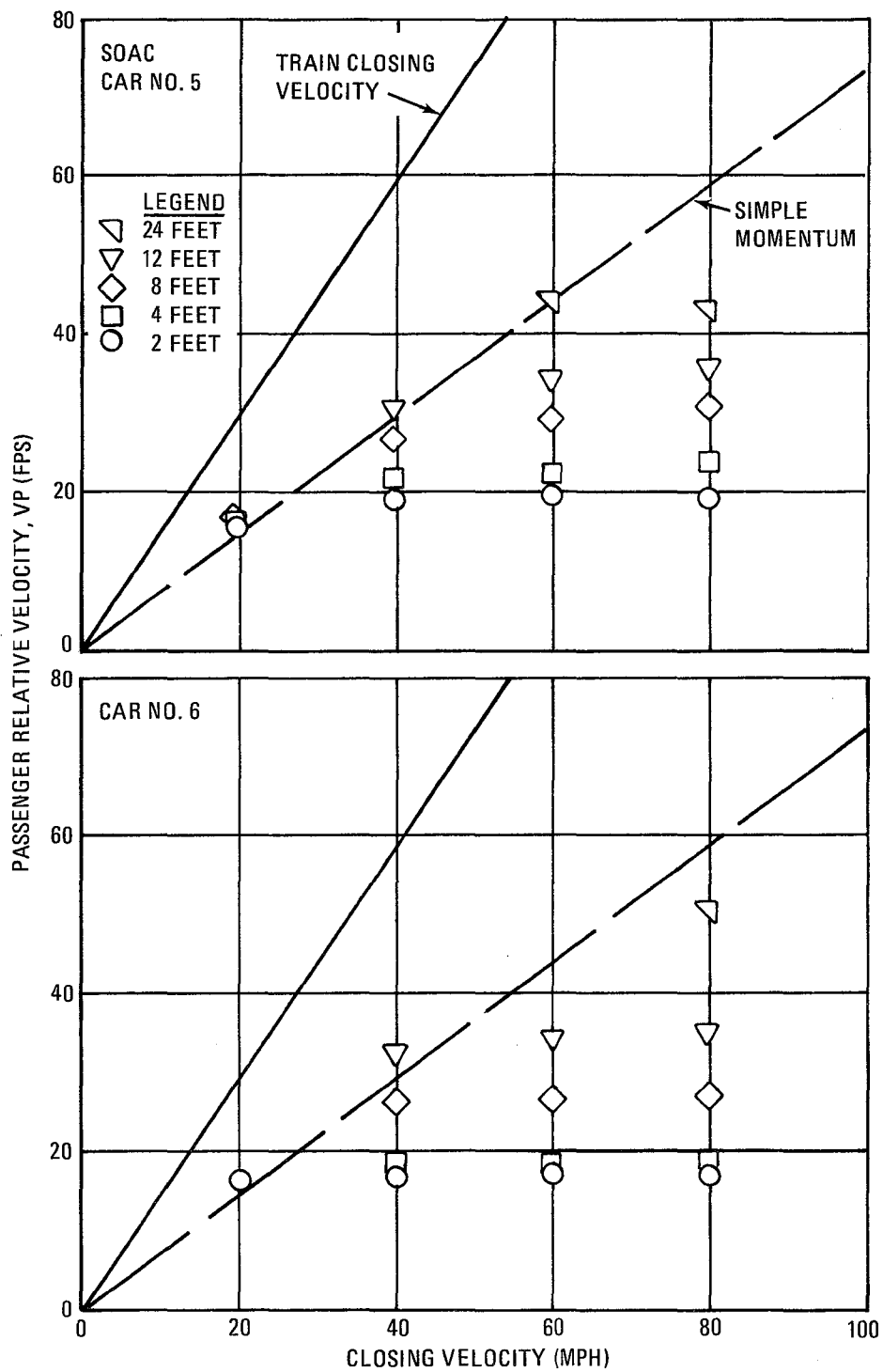
Figure 6-6. Passenger Relative Velocity Versus Train Closing Velocity (Sheet 1 of 2)
