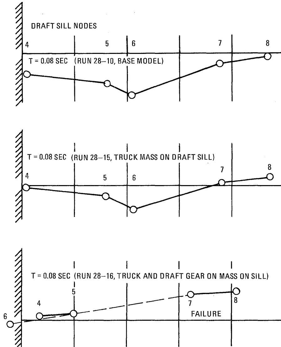
Figure 2-12. Anticlimber Hitting Barrier: Draft Sill Deflections for Different Mass Arrangements
