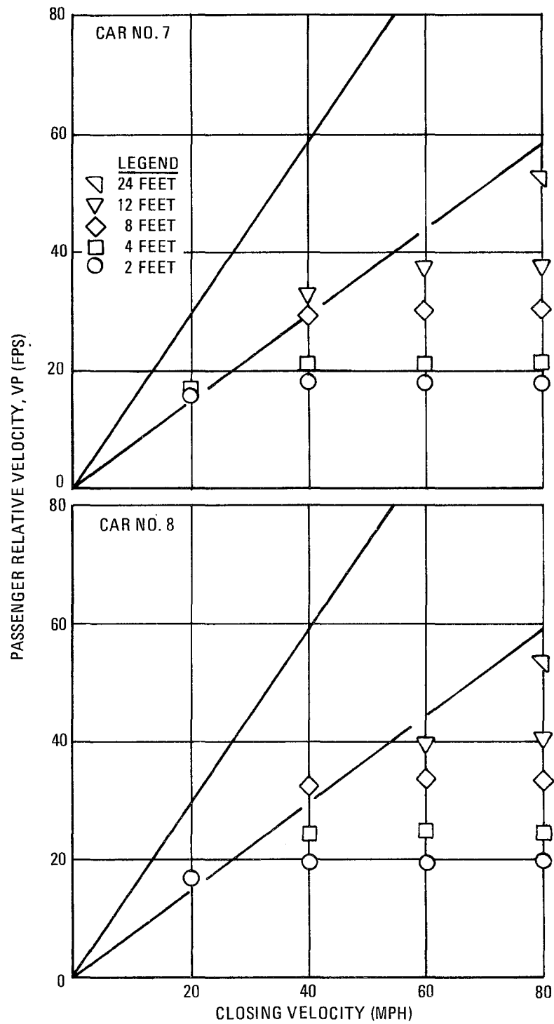
Figure 6-6. Passenger Relative Velocity Versus Train Closing Velocity (Sheet 2 of 2)
