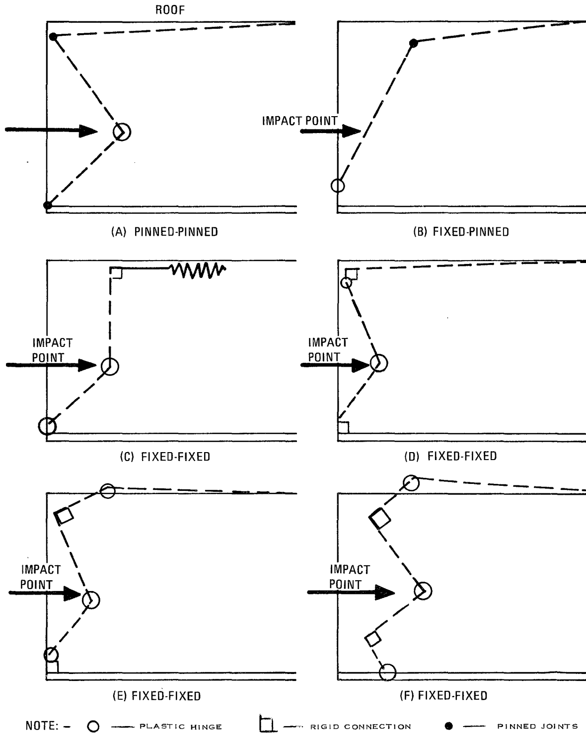
Figure 9-2. Collision Post Energy Absorbing Modes
