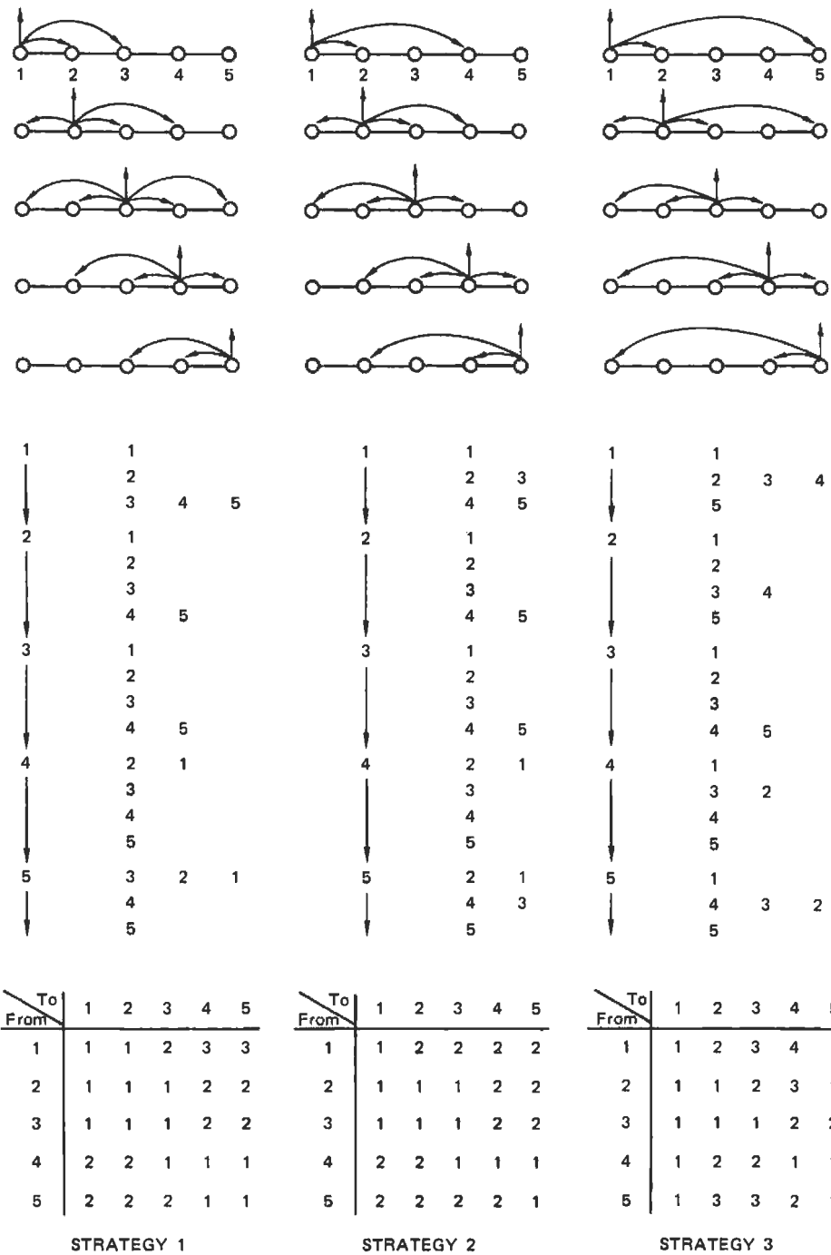
FIGURE 64 THREE BLOCKING STRATEGIES WITH CONSTRAINTS ON BLOCK MAKING CAPACITIES AND THE ASSOCIATED SWITCHING MATRICES
