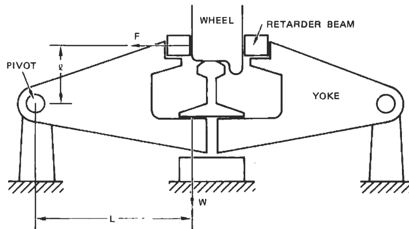
FIGURE 25 PRINCIPLE OF WEIGHT-RESPONSIVE RETARDER
