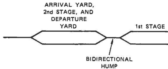
FIGURE 54 TWO-STAGE HUMPH YARD (CONFIGURATION 3)
