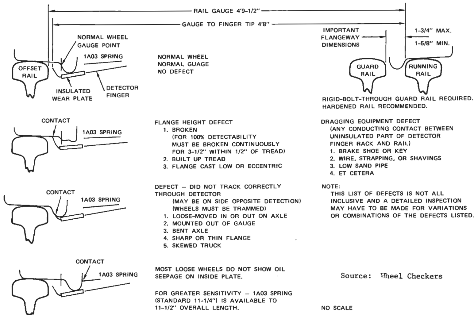
FIGURE 23 BROKEN-FLANGE AND LOOSE-WHEEL DETECTOR
