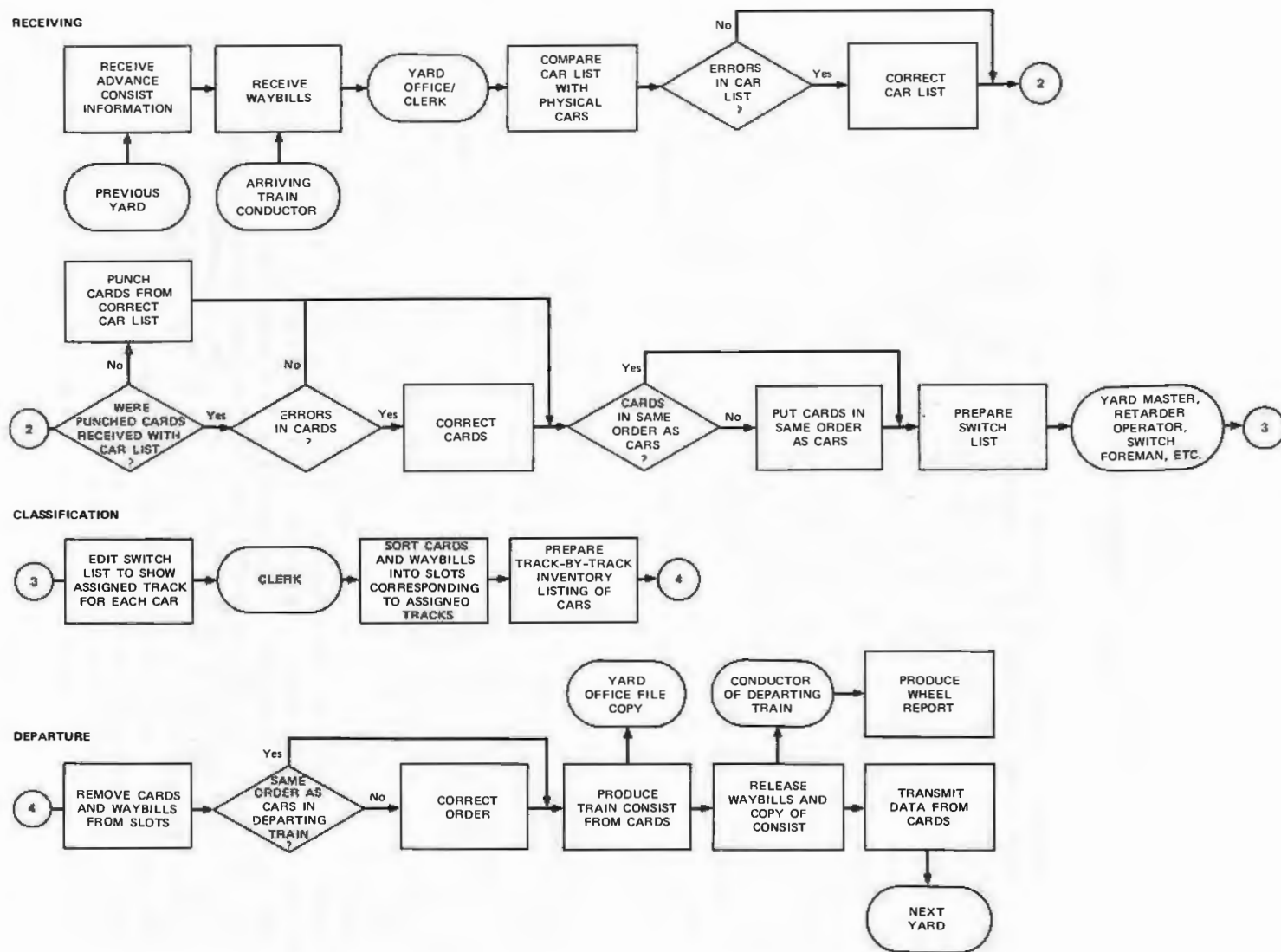
FIGURE A-1 INFORMATION FLOW IN MECHANIZED YARDS
