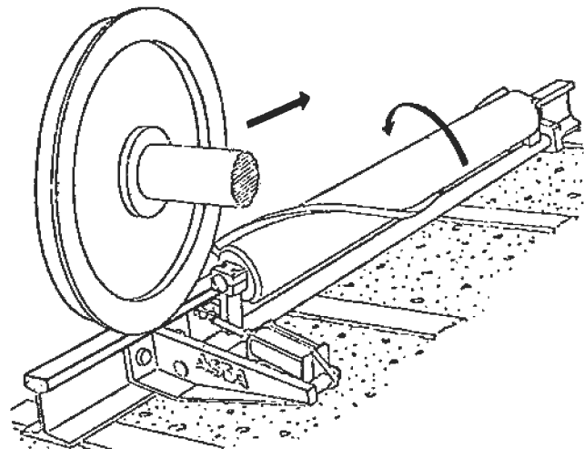
FIGURE 27 HYDRAULIC RETARDER
