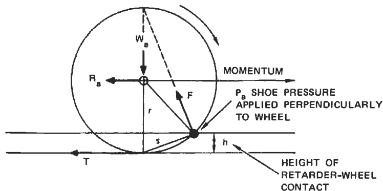
FIGURE 24 PRINCIPLE OF RETARDATION
