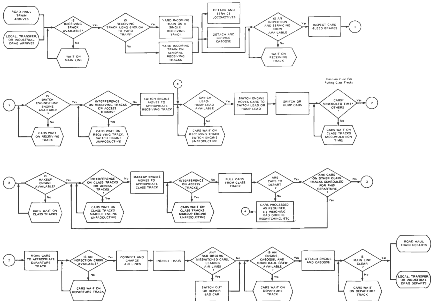
FIGURE 7 CAR HANDLING PROCESSES IN CLASSIFICATION YARDS
