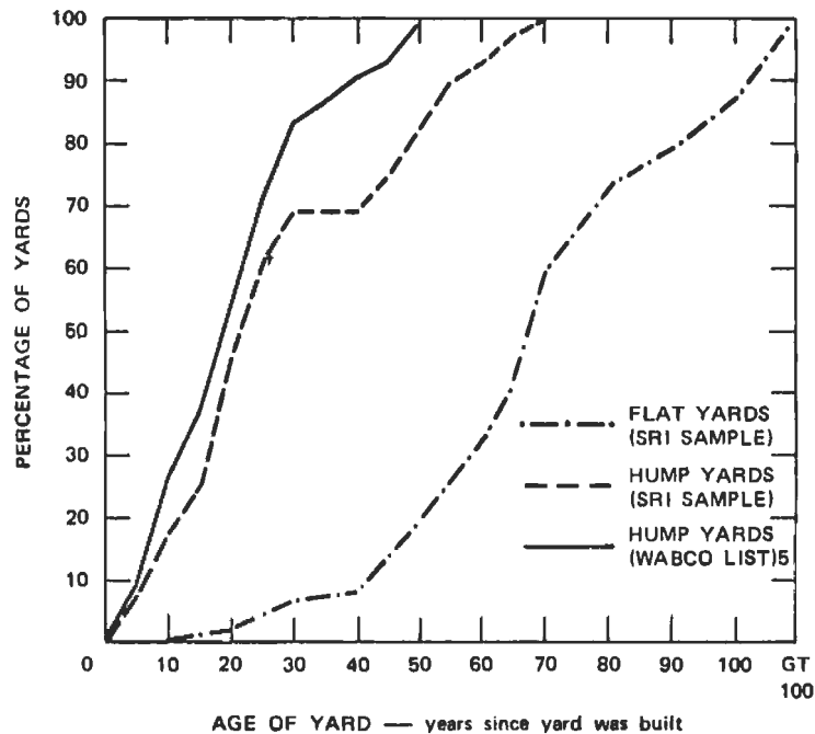
FIGURE 13 AGE DISTRIBUTION OF CLASSIFICATION YARDS
