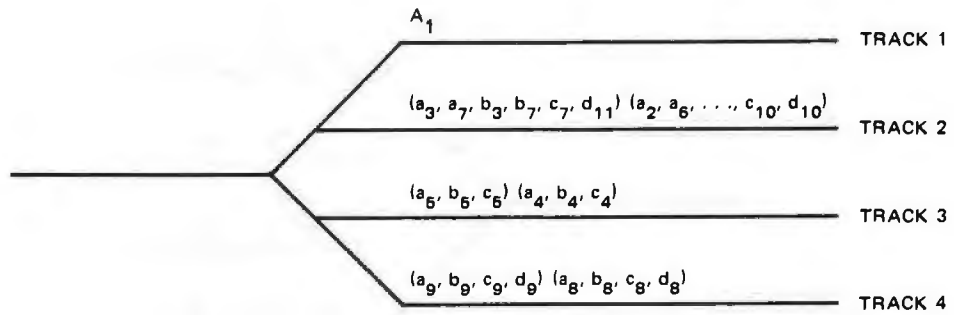
FIGURE 45 STRATEGY 4: CAR GROUPING AFTER RESWITCHING TRACK 1
