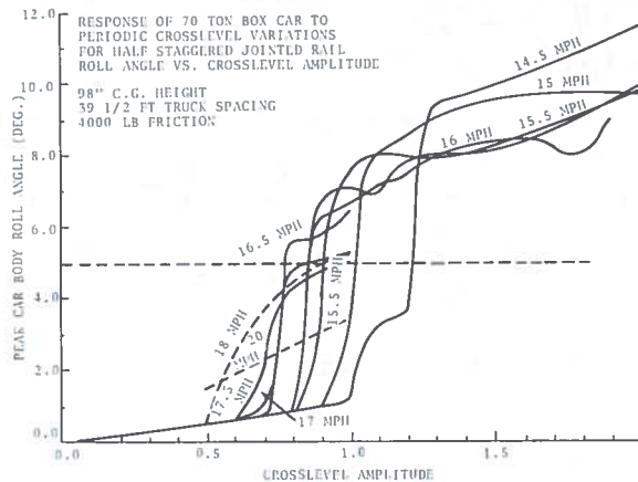
FIGURE 10. CROSSLEVEL AMPLITUDE
