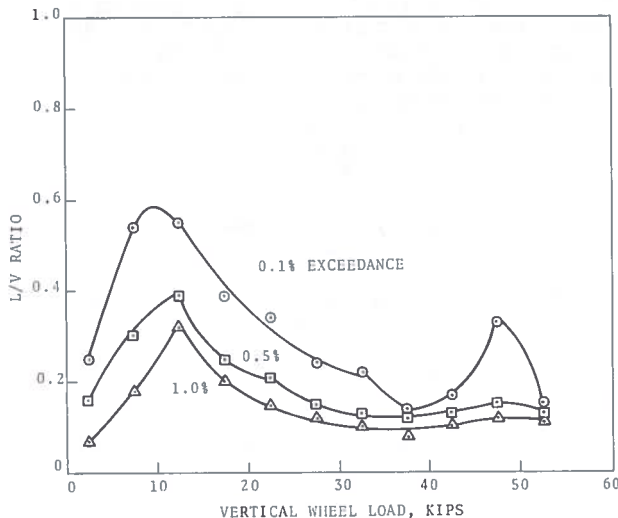
FIGURE 5. FREQUENCY OF EXCEEDANCE CURVES FOR L/V RATIO VERSUS VERTICAL WHEEL LOAD, TANGENT BJR TRACK, ALL TRAFFIC, ALL SPEEDS, ALL MEASUREMENT SITES IN TEST SECTION
