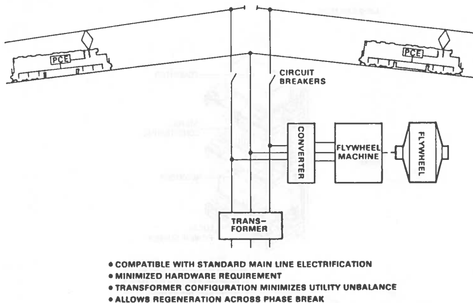
FIGURE 1. OPTIMUM WESS DESIGN
