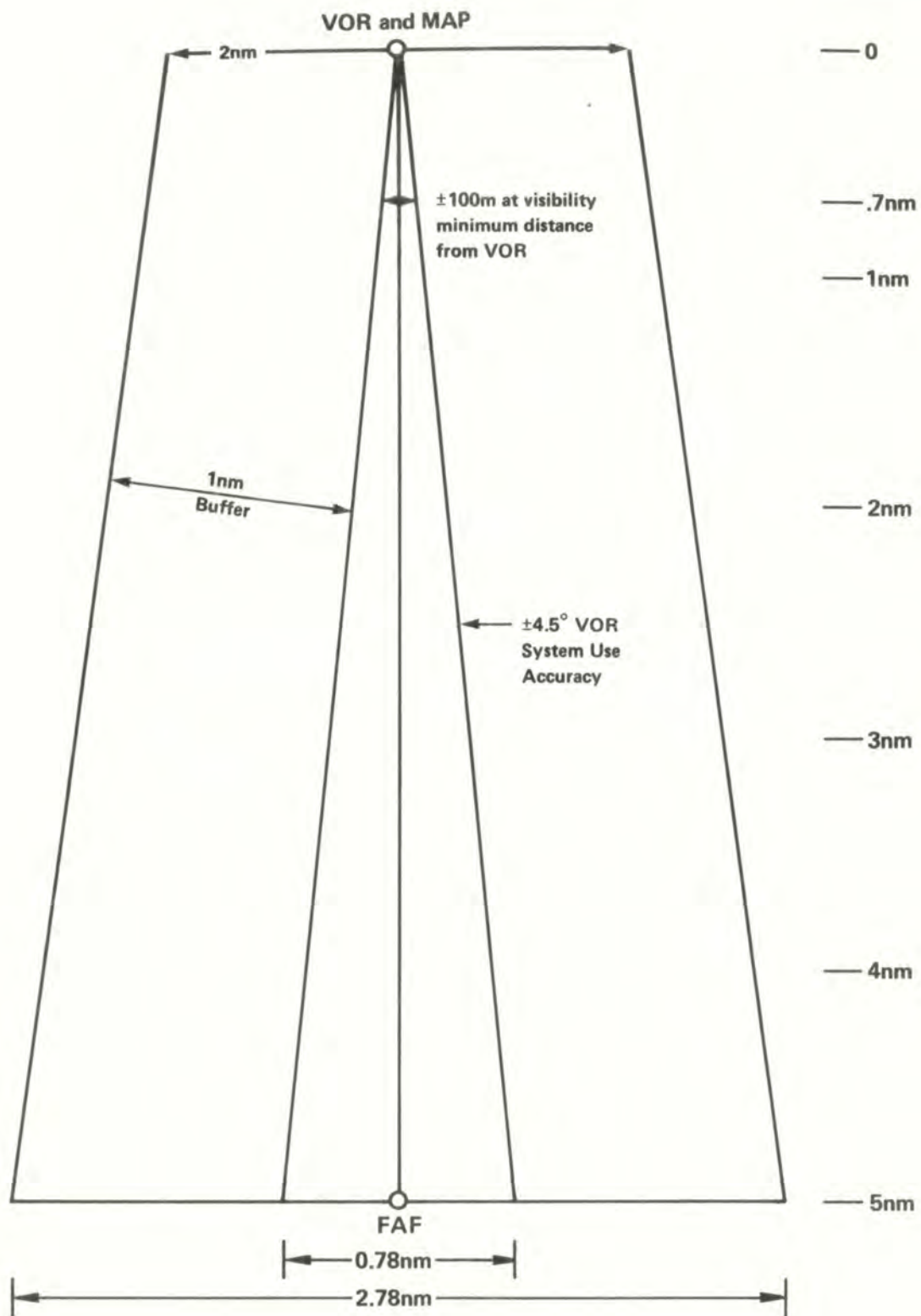
FIGURE II-2.1 Non-Precision Approach Obstacle Clearance Area for Current VOR with MAP at VOR facility
