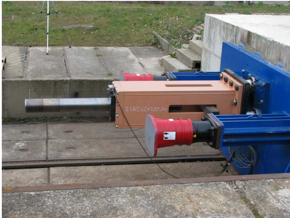
Figure 52. An example test setup with residual energy absorption crash buffers
