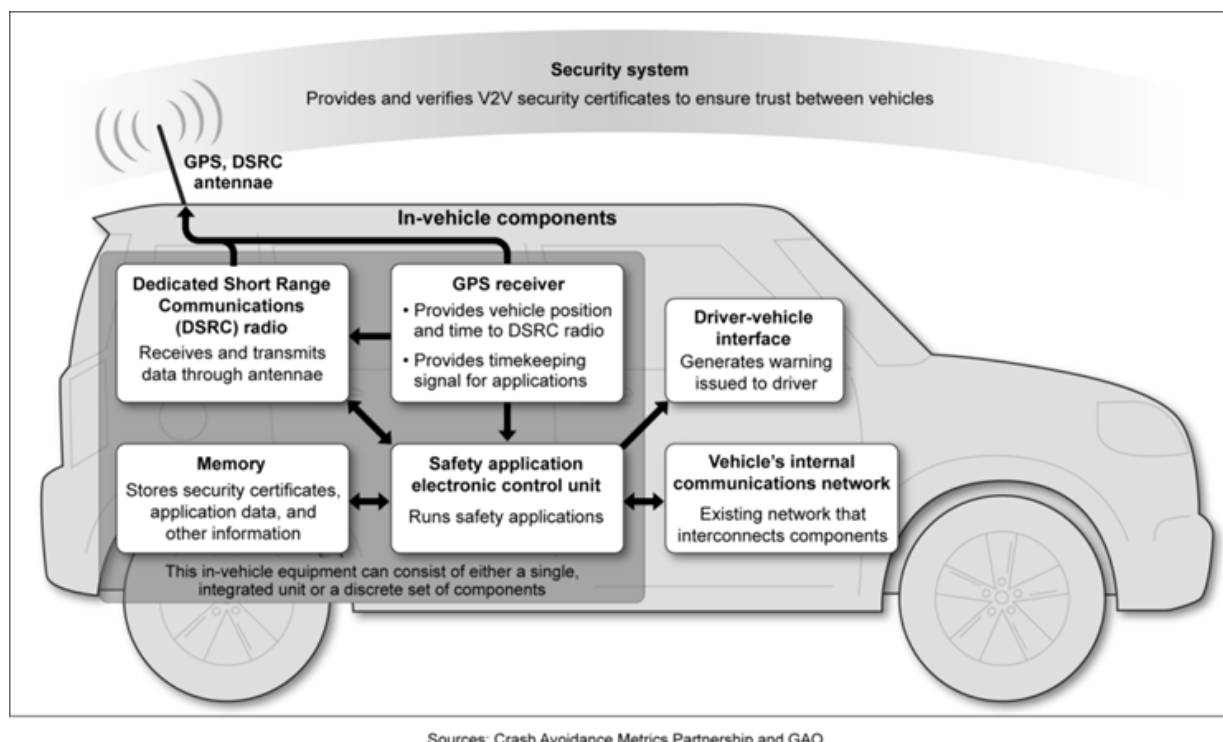
Figure E-1. Illustration of DSRC Vehicle-Based Technologies
