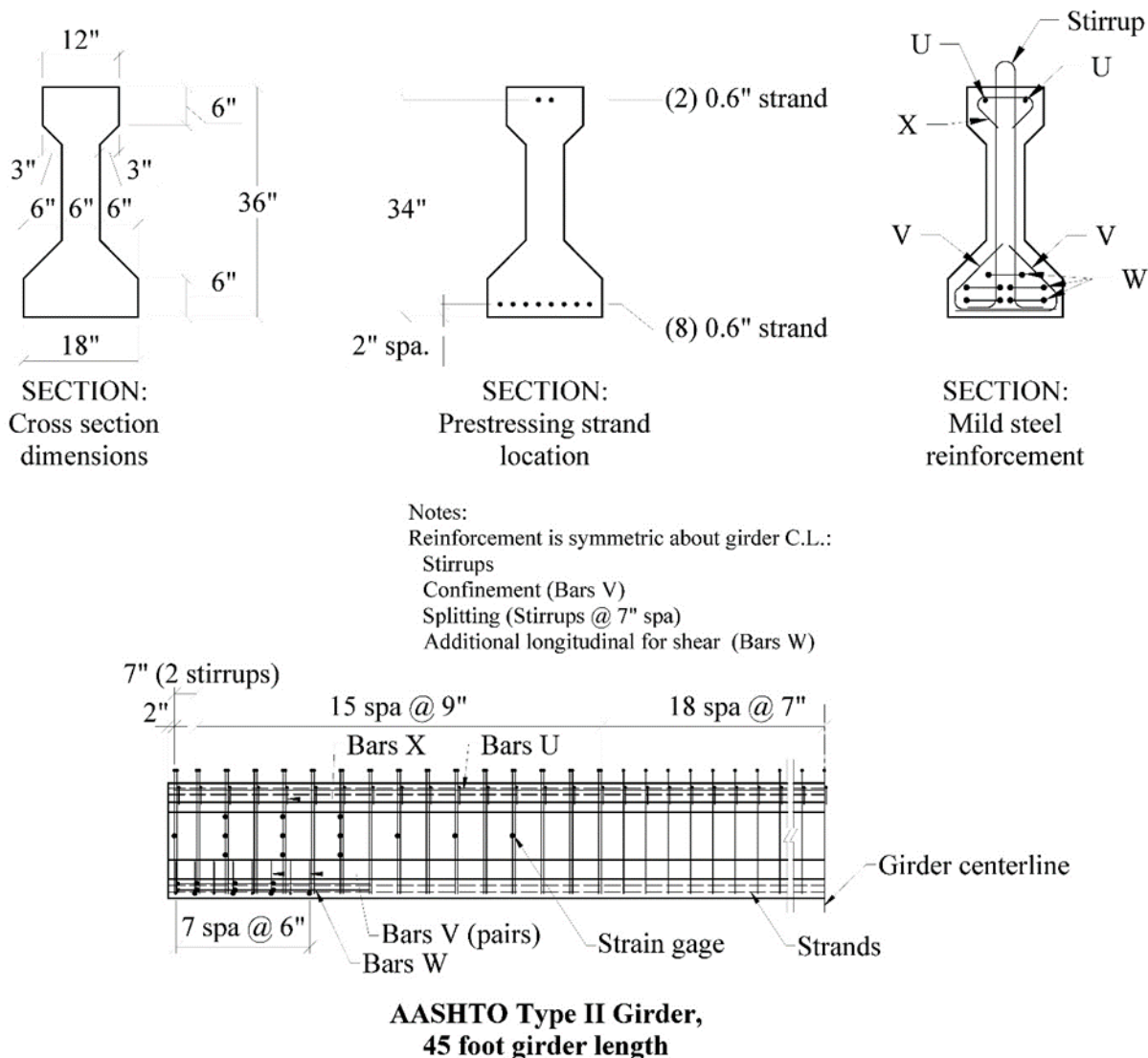
Figure 4. Illustration. Beam Design 4.
