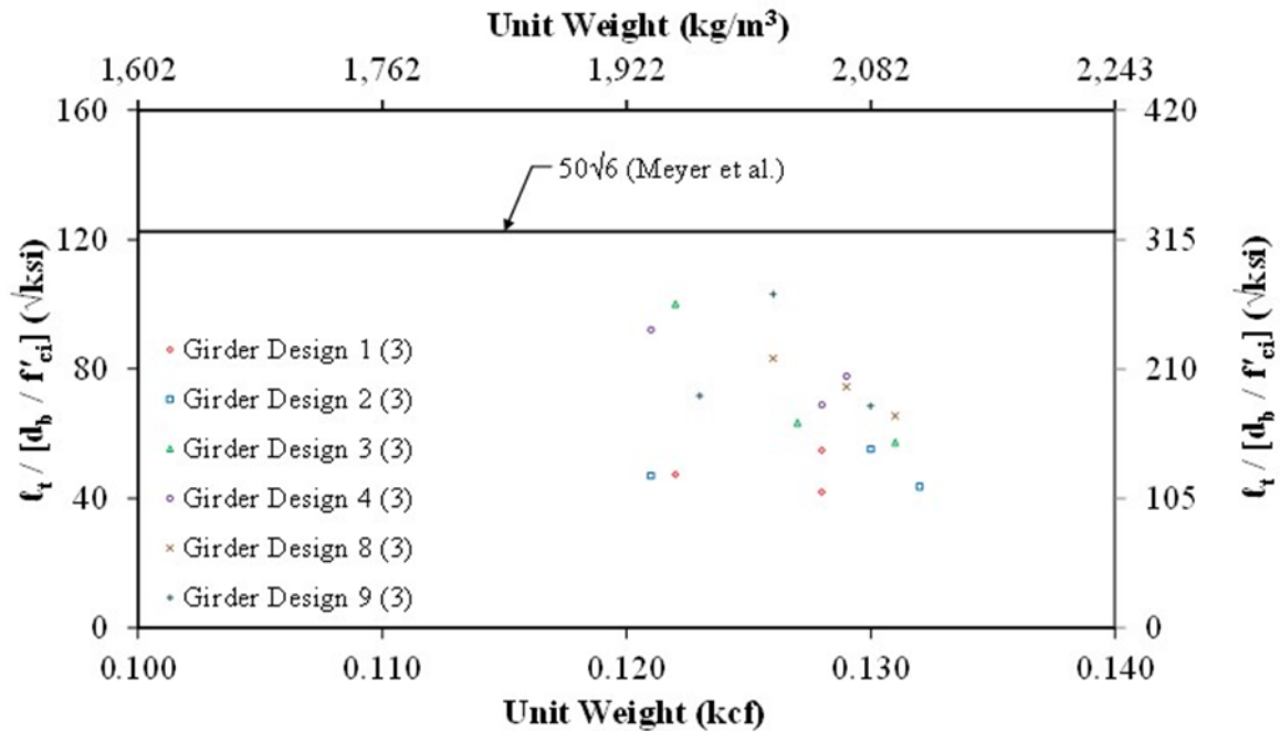
Figure 25. Graph. Normalized Transfer Length ( l_t/[d_b/\sqrt{f'_{ci}}] ) Compared to Unit Weight by Girder Design.
