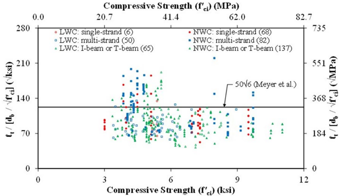
Figure 72. Graph. Normalized Transfer Length ( l_t/[d_b/\sqrt{f'_{ci}}] ) Compared to Compressive Strength ( f'_{ci} ) by Specimen Type in the TFHRC Database.
