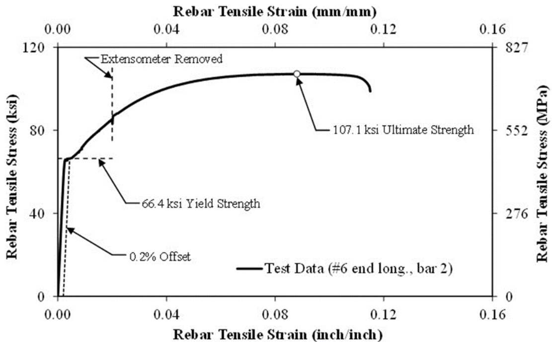
Figure 106. Graph. Measured Stress-Strain Relationship for #6 End Longitudinal Reinforcing Bar for Girder Design 1-4 – Coupon 2.
