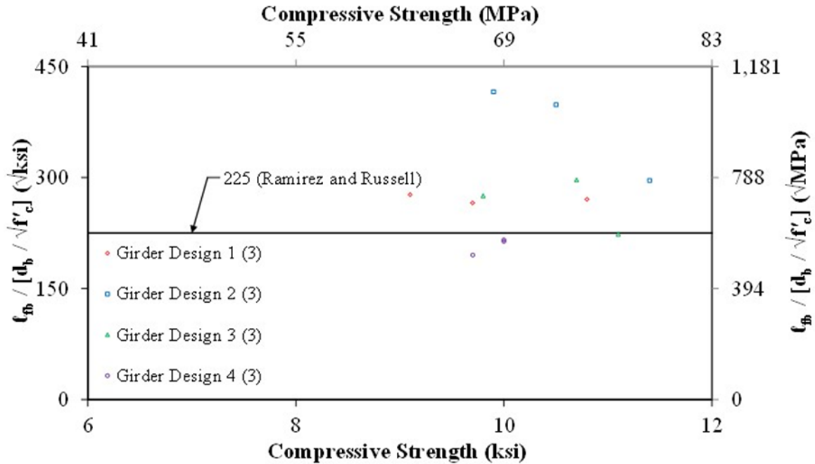
Figure 54. Graph. Normalized Flexural Bond Length ( \ell_b / [d_b / \sqrt{f'_{ci}}] ) Compared to Compressive Strength by Girder Design.
