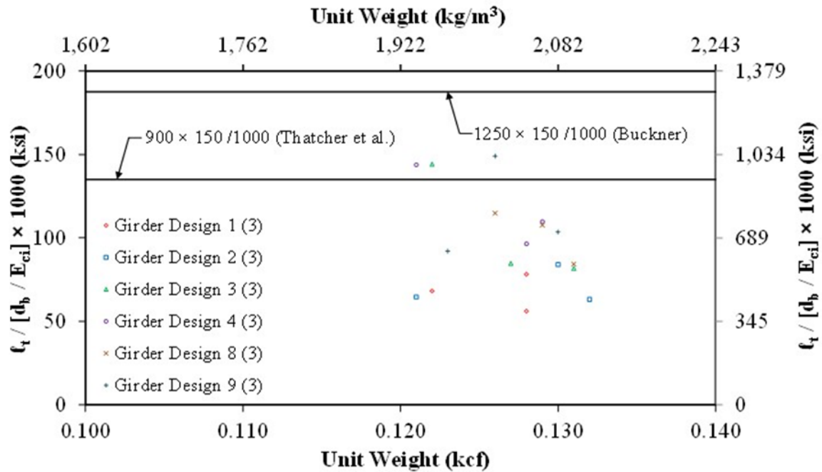
Figure 29. Graph. Normalized Transfer Length ( \ell_t/[d_b/E_{ci}] ) Compared to Unit Weight by Girder Design.
