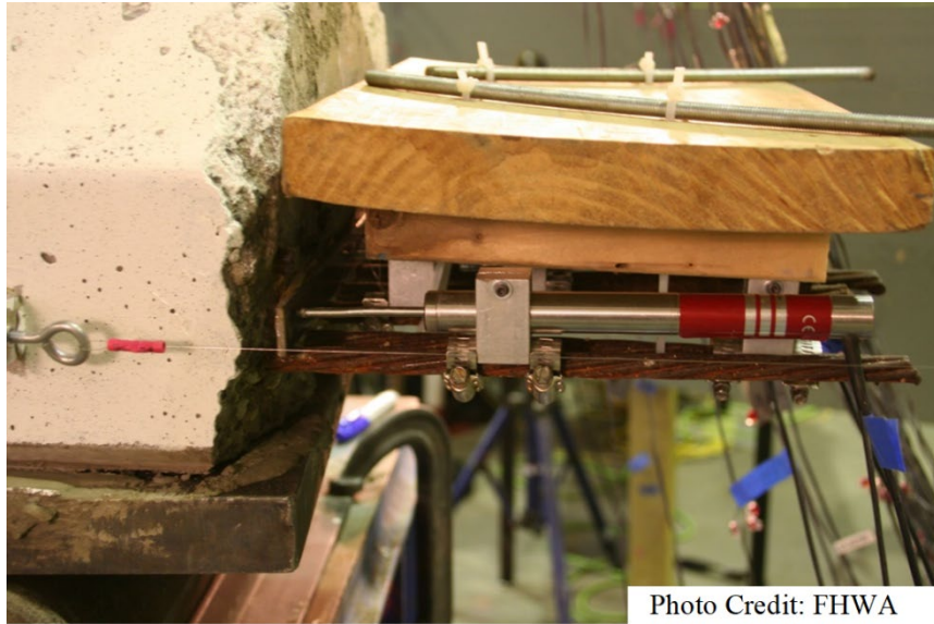
Figure 39. Photo. LVDTs used to Measure Strand Slip.
