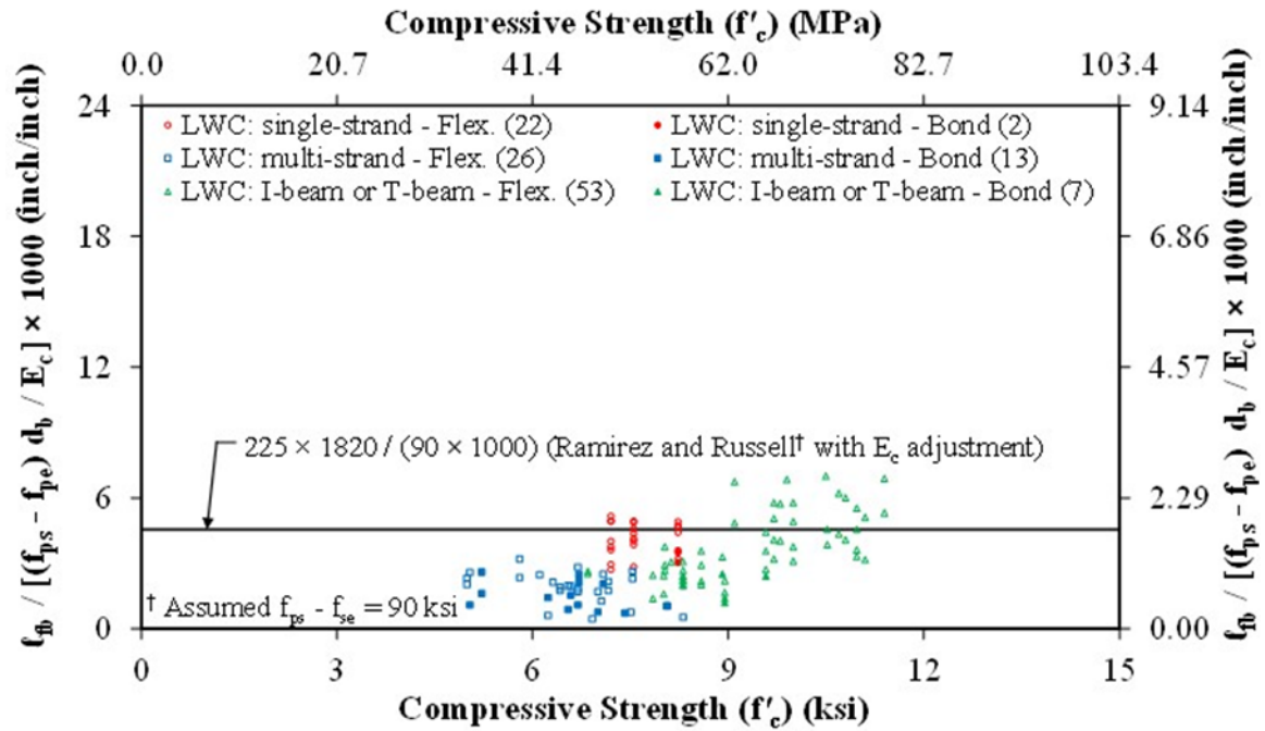
Figure 88. Graph. Normalized Flexural Bond Length ( \ell_{fb}/[(f_{ps}-f_{pe})d_b/E_c] ) Compared to Compressive Strength ( f'_c ) by Specimen Type for LWC in the TFHRC Database.
