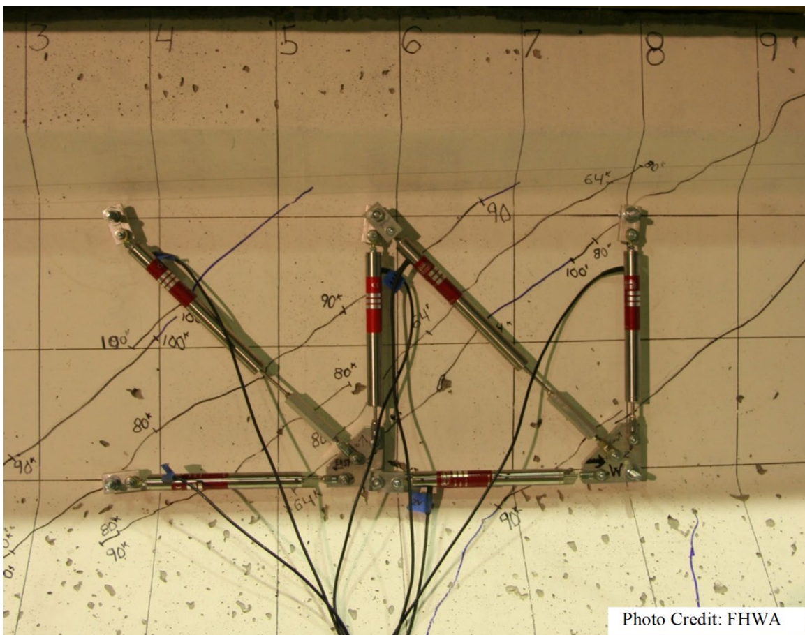
Figure 40. Photo. LVDTs used to Measure Average Concrete Strain in a “Rosette.”
