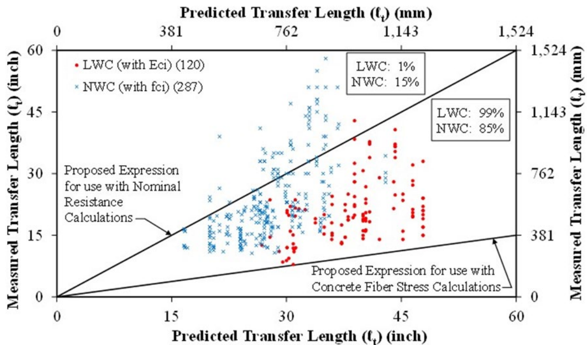
Figure 93. Graph. Measured Transfer Length ( l_t ) Compared to Transfer Length Predicted by Proposed Expressions for Specimens in the TFHRC Database.
