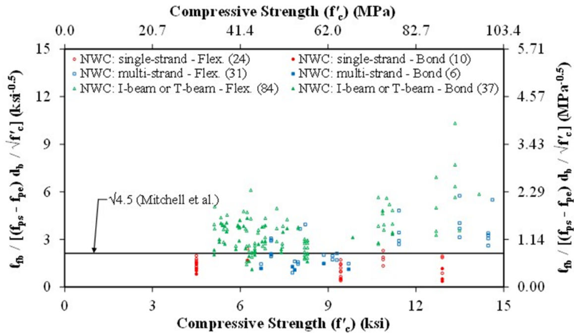
Figure 85. Graph. Normalized Flexural Bond Length ( \ell_{fb}/[(f_{ps}-f_{pe})d_b/\sqrt{f'_c}] ) Compared to Compressive Strength ( f'_c ) by Specimen Type for NWC in the TFHRC Database.
