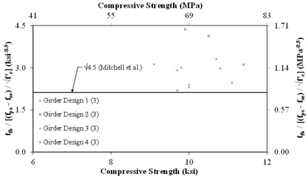
Figure 56. Graph. Normalized Flexural Bond Length ( \ell_{fb} / [(f_{ps} - f_{se})d_b / \sqrt{f'_c}] ) Compared to Compressive Strength by Girder Design.
