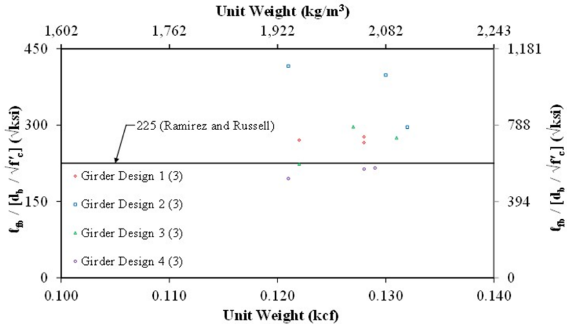
Figure 55. Graph. Normalized Flexural Bond Length ( \ell_b / [d_b / \sqrt{f'_{ci}}] ) Compared to Unit Weight by Girder Design.
