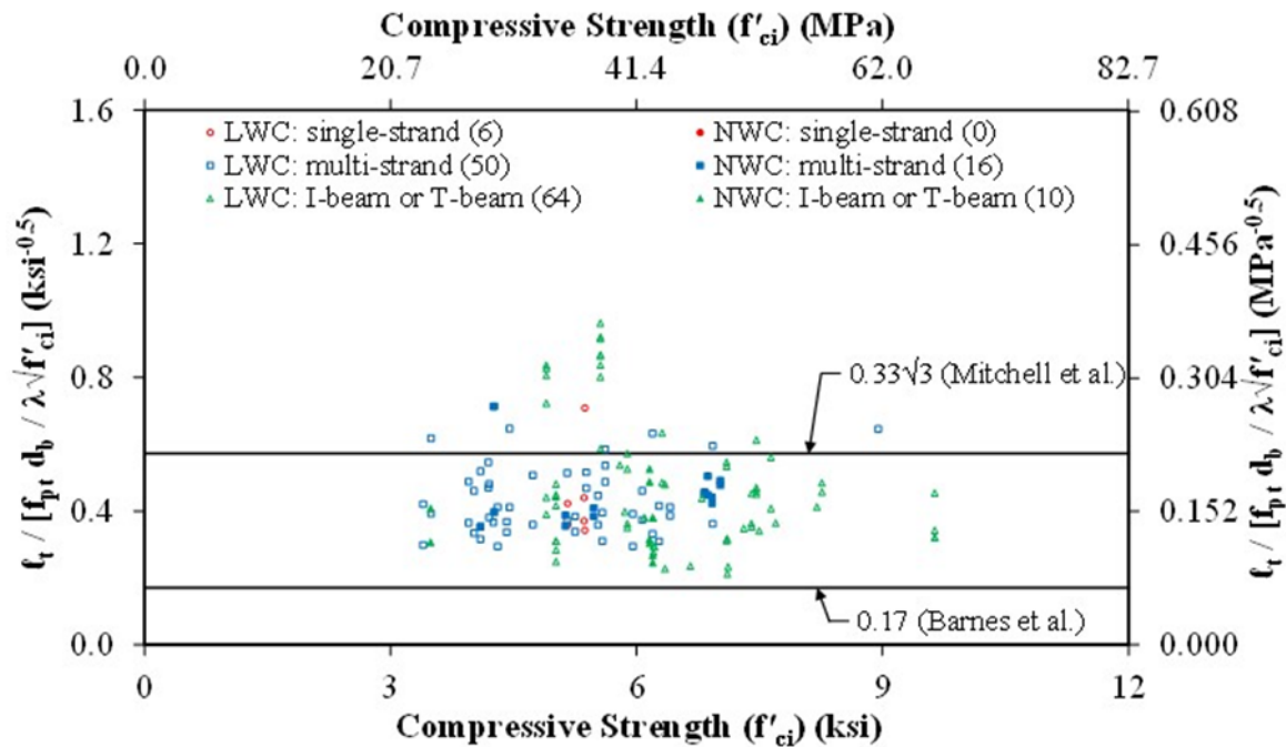
Figure 79. Graph. Normalized Transfer Length ( t_t / [f_{pt} d_b / \lambda \sqrt{f'_{ci}}] ) Compared to Compressive Strength ( f'_{ci} ) by Specimen Type in the TFHRC Database.
