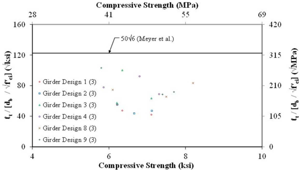
Figure 24. Graph. Normalized Transfer Length ( l_t/[d_b/\sqrt{f'_{ci}}] ) Compared to Compressive Strength by Girder Design.
