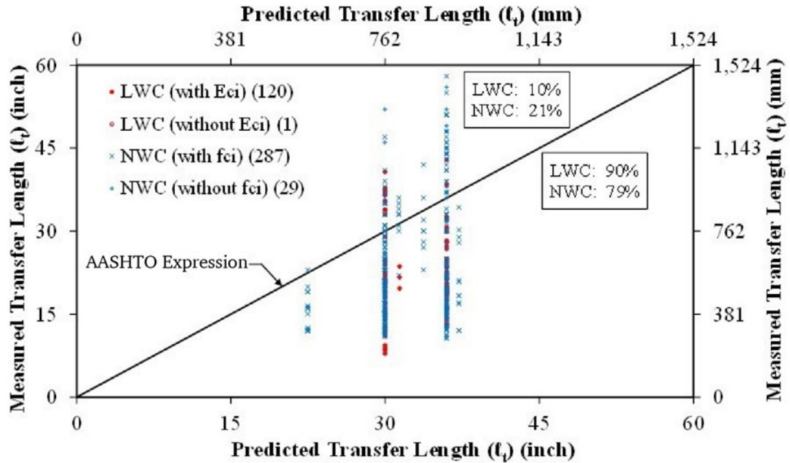
Figure 92. Graph. Measured Transfer Length ( l_t ) Compared to Transfer Length Predicted by AASHTO Expression for Specimens in the TFHRC Database.
