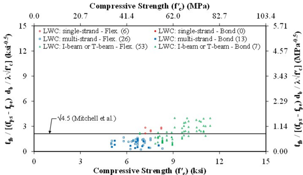
Figure 91. Graph. Normalized Flexural Bond Length ( \ell_{fb}/[(f_{ps}-f_{pe})d_b/\lambda\sqrt{f'_c}] ) Compared to Compressive Strength ( f'_c ) by Specimen Type for LWC in the TFHRC Database.
