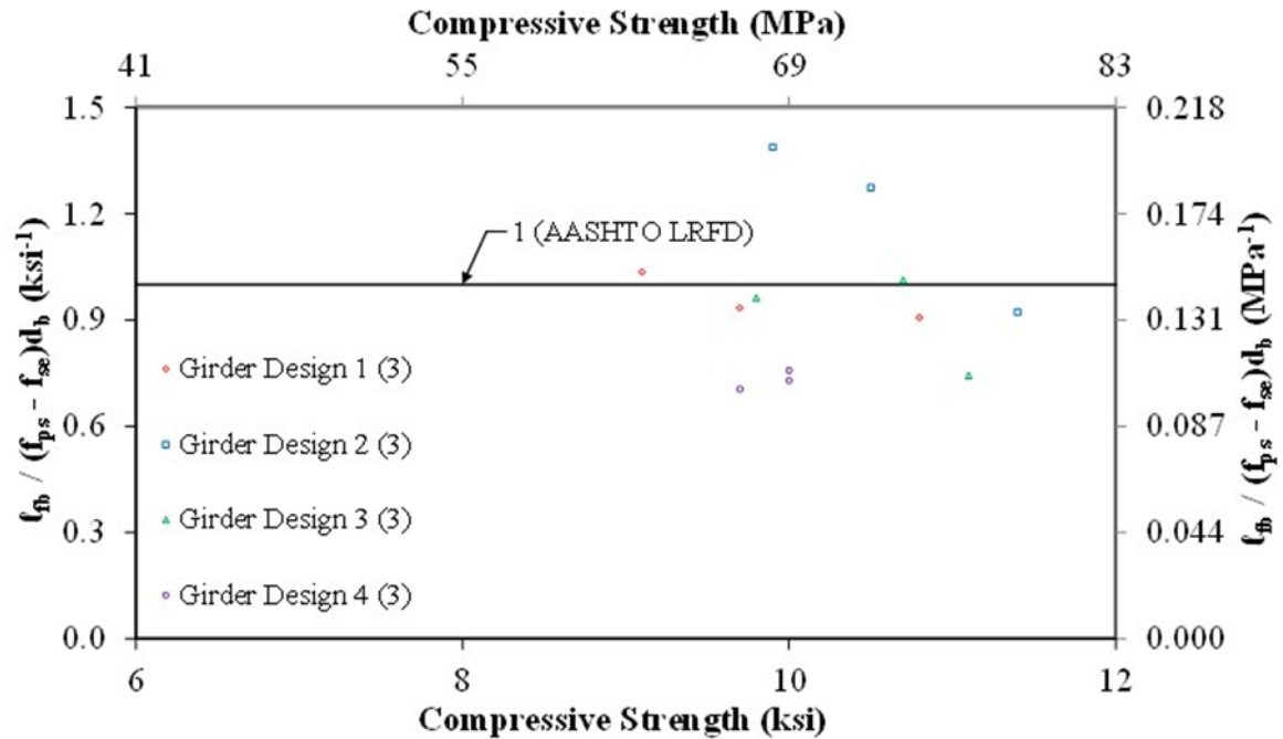
Figure 52. Graph. Normalized Flexural Bond Length ( \ell_{fb} / (f_{ps} - f_{se})d_b ) Compared to Compressive Strength by Girder Design.
