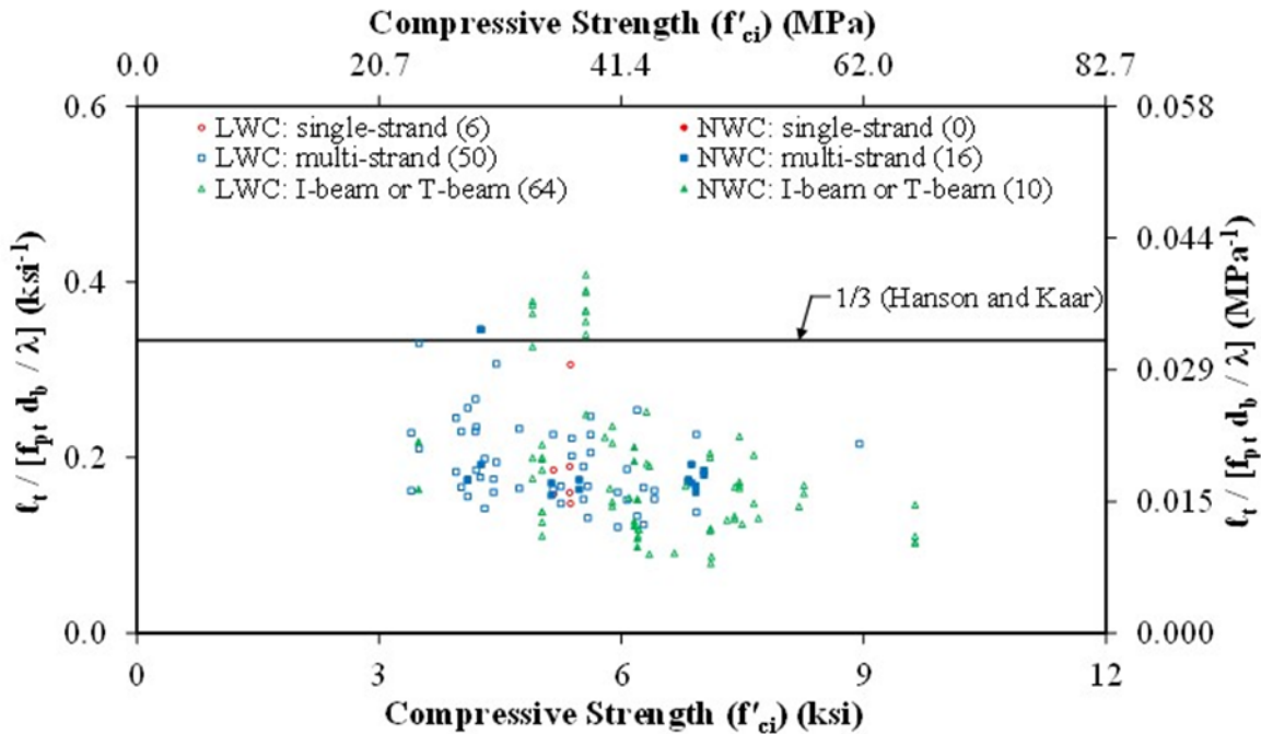
Figure 77. Graph. Normalized Transfer Length ( l_t/[f_{pt}d_b/\lambda] ) Compared to Compressive Strength ( f'_{ci} ) by Specimen Type in the TFHRC Database.
