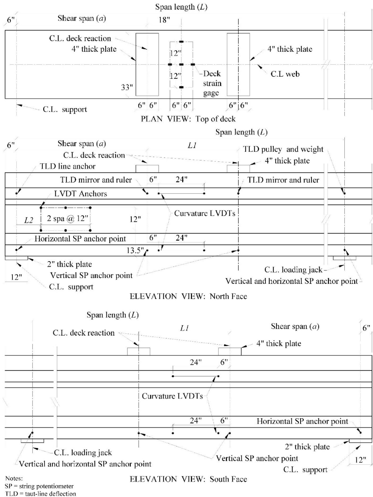
Figure 37. Illustration. External Instrumentation for AASHTO Type II Girders.
