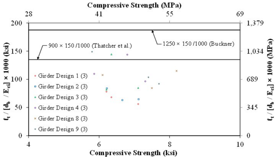
Figure 28. Graph. Normalized Transfer Length ( \ell_t/[d_b/E_{ci}] ) Compared to Compressive Strength by Girder Design.
