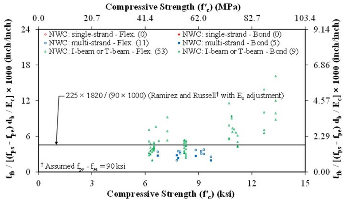
Figure 89. Graph. Normalized Flexural Bond Length ( \ell_{fb}/[(f_{ps}-f_{pe})d_b/E_c] ) Compared to Compressive Strength ( f'_c ) by Specimen Type for NWC in the TFHRC Database.
