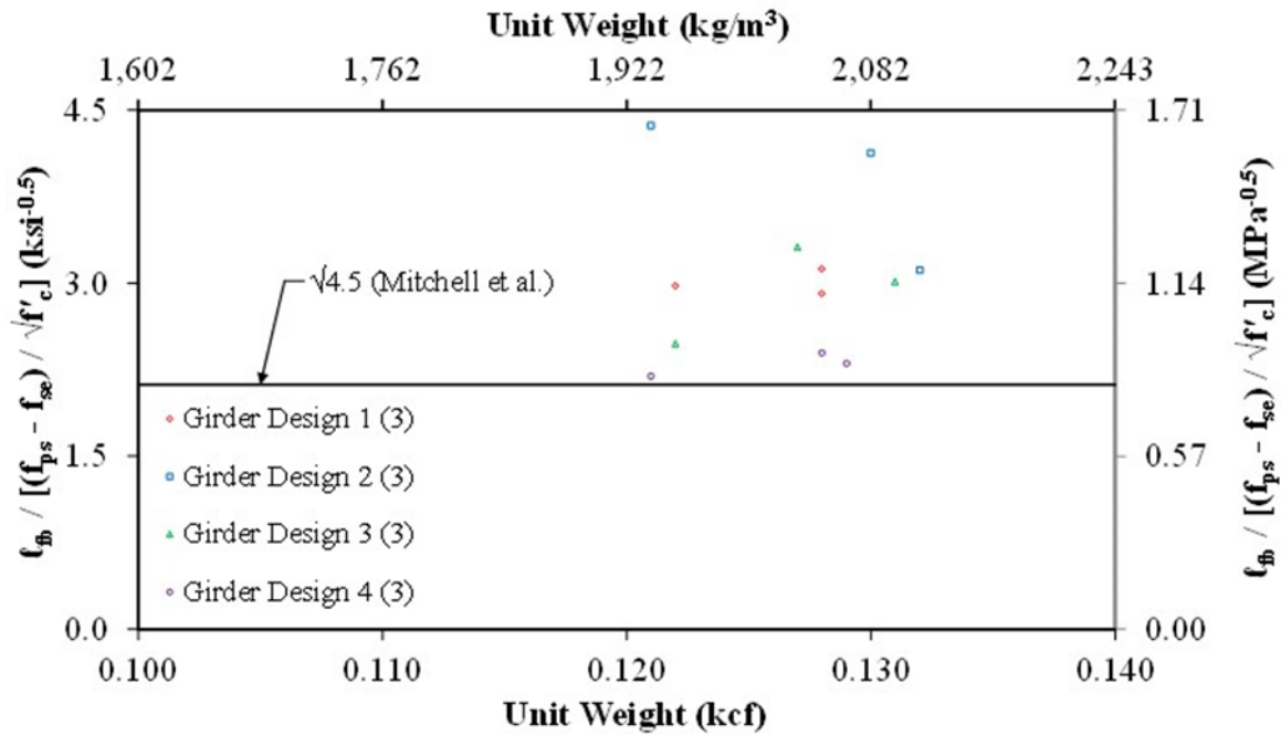
Figure 57. Graph. Normalized Flexural Bond Length ( \ell_{fb} / [(f_{ps} - f_{se})d_b / \sqrt{f'_c}] ) Compared to Unit Weight by Girder Design.
