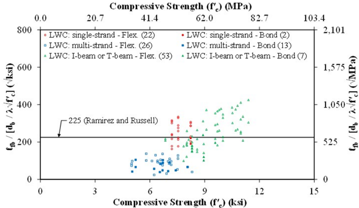
Figure 90. Graph. Normalized Flexural Bond Length ( \ell_{fb}/[d_b/\lambda\sqrt{f'_c}] ) Compared to Compressive Strength ( f'_c ) by Specimen Type for LWC in the TFHRC Database.
