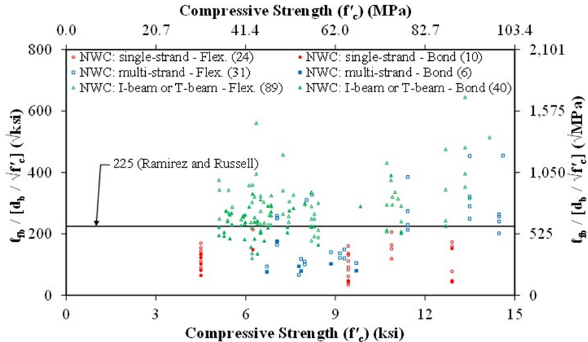
Figure 83. Graph. Normalized Flexural Bond Length ( \ell_{fb}/[d_b/\sqrt{f'_c}] ) Compared to Compressive Strength ( f'_c ) by Specimen Type for NWC in the TFHRC Database.
