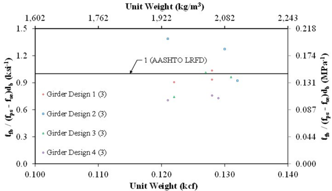
Figure 53. Graph. Normalized Flexural Bond Length ( \ell_{fb} / (f_{ps} - f_{se})d_b ) Compared to Unit Weight by Girder Design.
