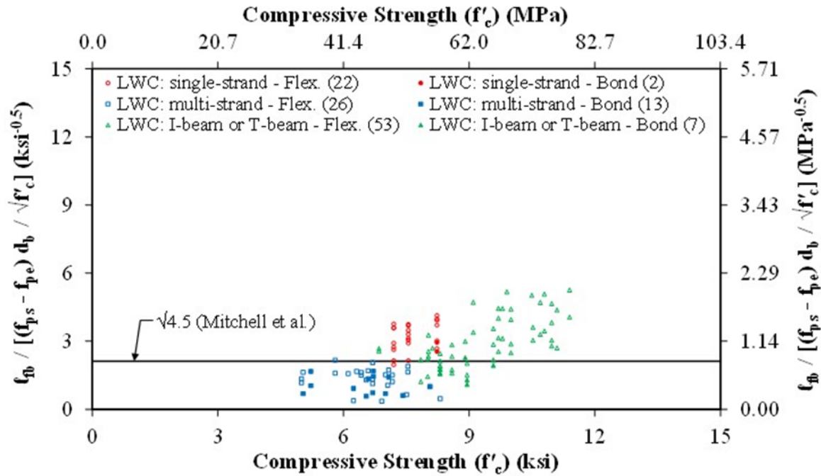
Figure 84. Graph. Normalized Flexural Bond Length ( \ell_{fb}/[(f_{ps}-f_{pe})d_b/\sqrt{f'_c}] ) Compared to Compressive Strength ( f'_c ) by Specimen Type for LWC in the TFHRC Database.
