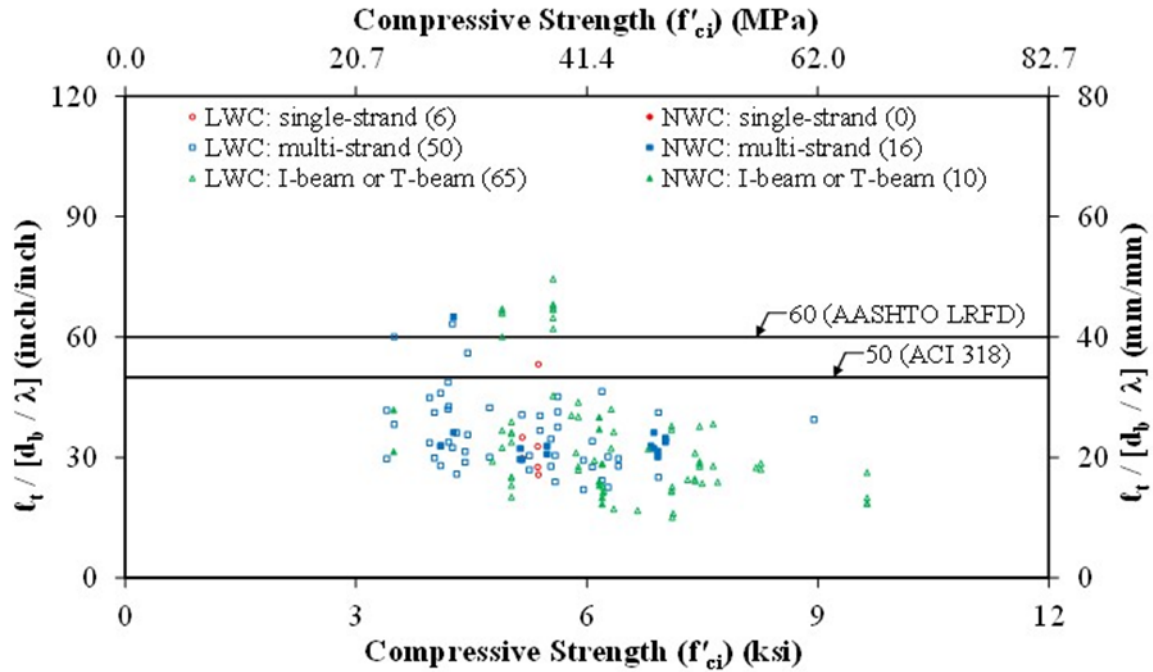
Figure 76. Graph. Normalized Transfer Length ( l_t/[d_b/\lambda] ) Compared to Compressive Strength ( f'_{ci} ) by Specimen Type in the TFHRC Database.
