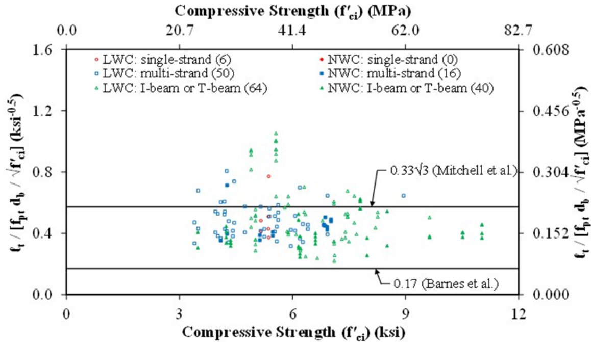
Figure 73. Graph. Normalized Transfer Length ( l_t/[f_{pt}d_b/\sqrt{f'_{ci}}] ) Compared to Compressive Strength ( f'_{ci} ) by Specimen Type in the TFHRC Database.
