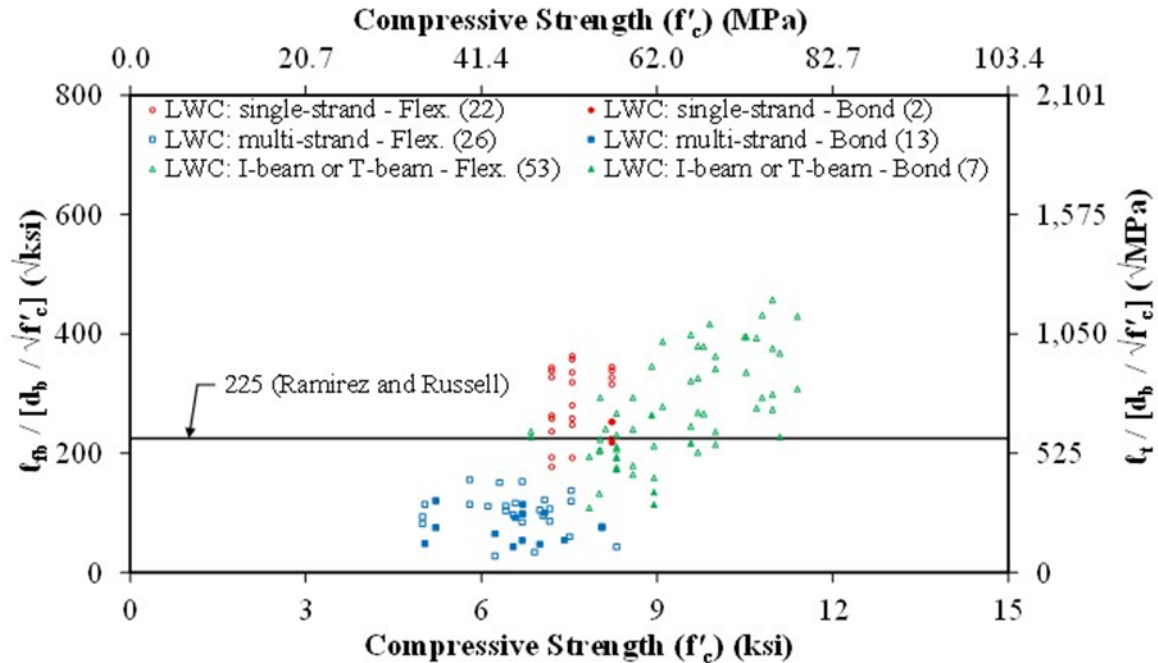
Figure 82. Graph. Normalized Flexural Bond Length ( \ell_{fb}/[d_b/\sqrt{f'_c}] ) Compared to Compressive Strength ( f'_c ) by Specimen Type for LWC in the TFHRC Database.
