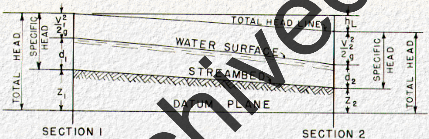
Figure 12. Water-Surface Profile of Channel with Nonuniform Flow
