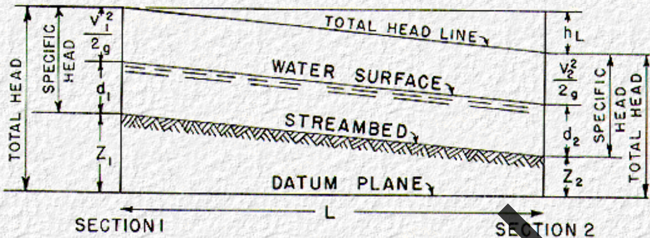
Figure 11. Water-Surface Profile of Channel with Uniform Flow
