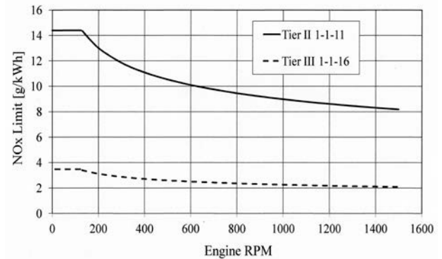
(a) ECA Marine Fuel Sulfur Content Limits in 2015 (b) ECA Tier III NOx Emissions Limits in 2016 Figure1: More stringent Emissions Control Area Requirements for the Great Lakes in 2015 and 2016
