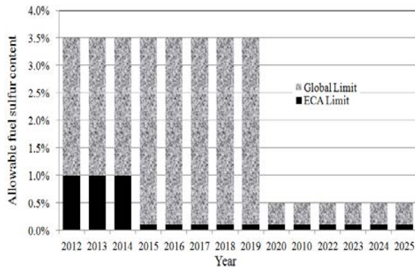
(a) ECA Marine Fuel Sulfur Content Limits in 2015 (b) ECA Tier III NOx Emissions Limits in 2016 Figure1: More stringent Emissions Control Area Requirements for the Great Lakes in 2015 and 2016
