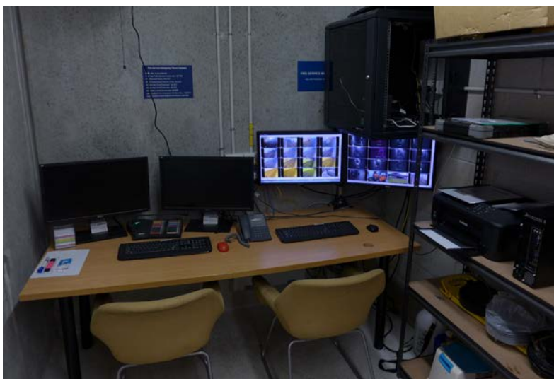
Figure 2-35: Victoria Park Tunnel backup control room
