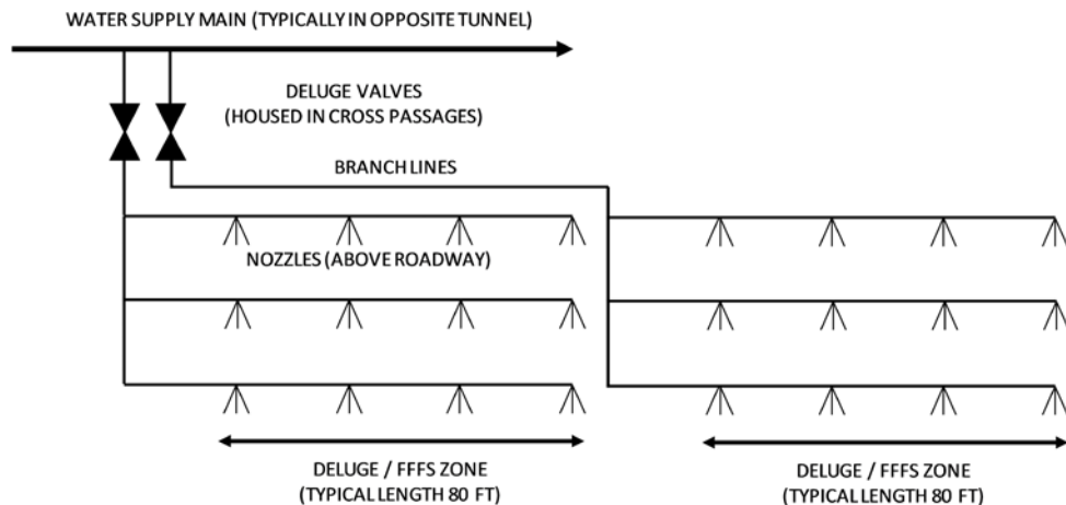
Figure 2-1: FFFS basic schematic. Source: FHWA
