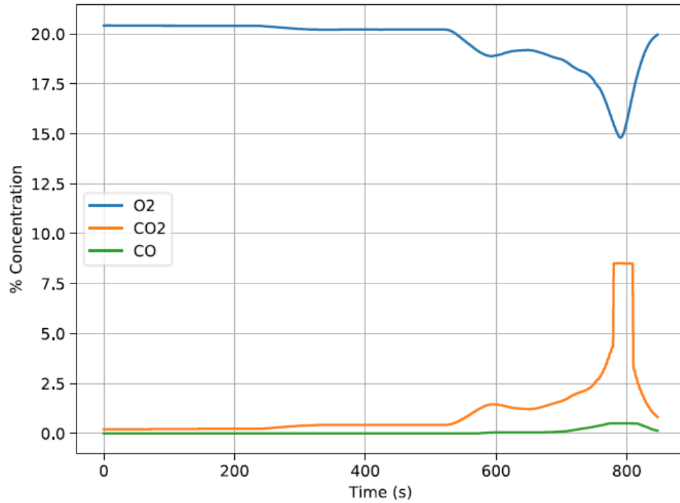
Figure C 16. Gas concentrations for Sample 2
