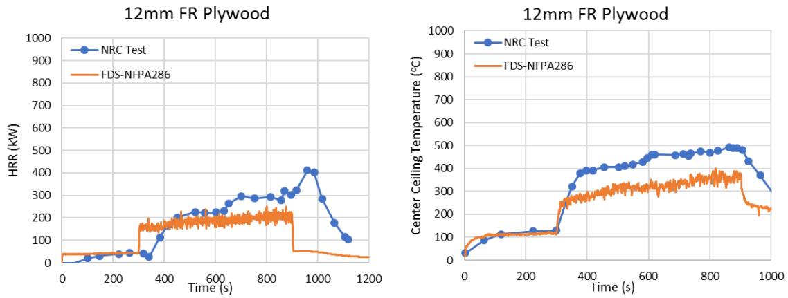
Figure D 4. Time history of HRR (left) and center ceiling temperature (right) of 12 mm fire retarded plywood tested in NFPA 286 room
