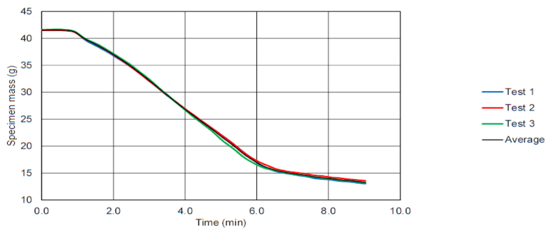
Specimen Mass
