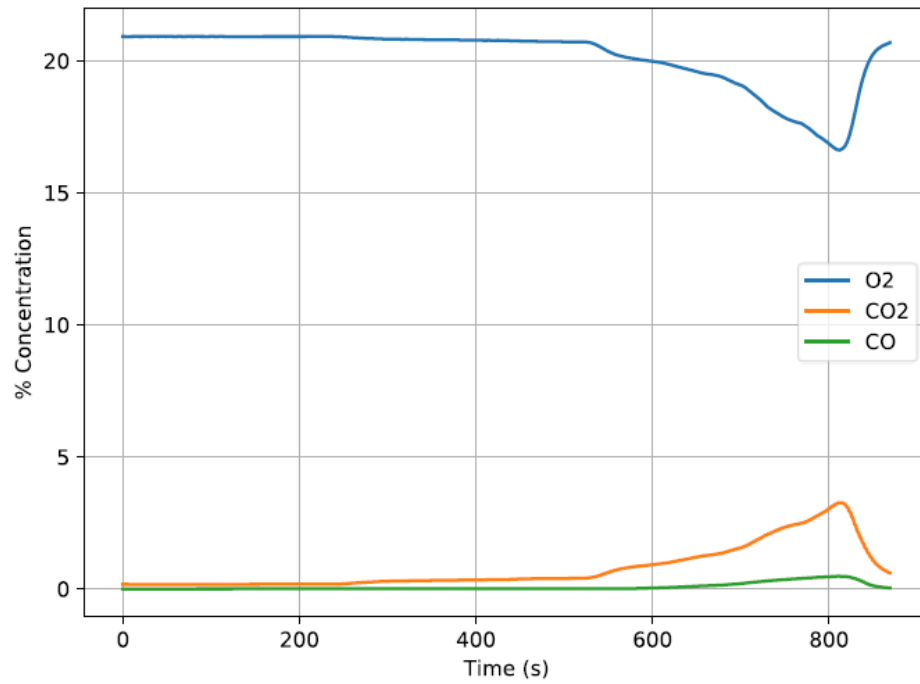
Figure C 10. Gas concentrations for Sample 6
