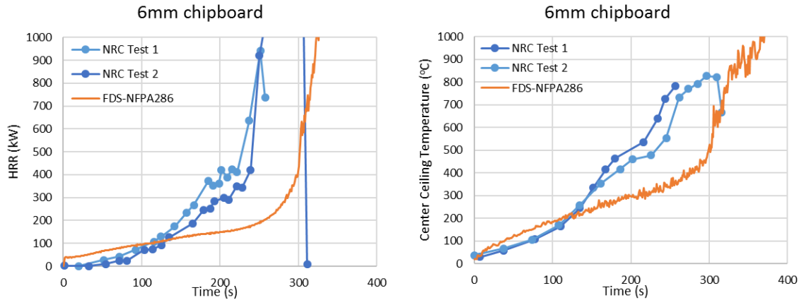
Figure D 2. Time history of HRR (left) and center ceiling temperature (right) of 6 mm chipboard tested in NFPA 286 room and FDS
