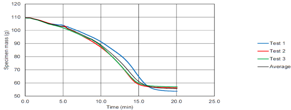
Specimen Mass
