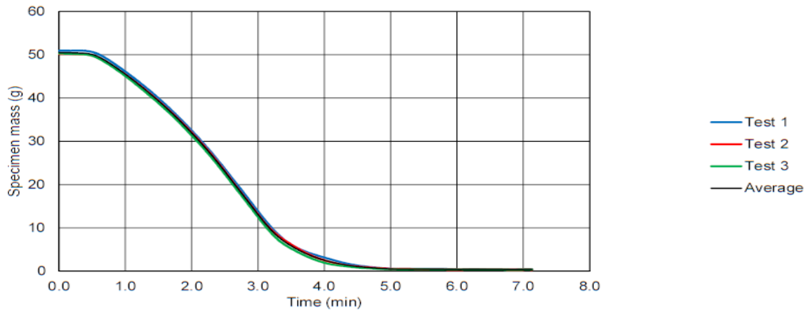
Specimen Mass
