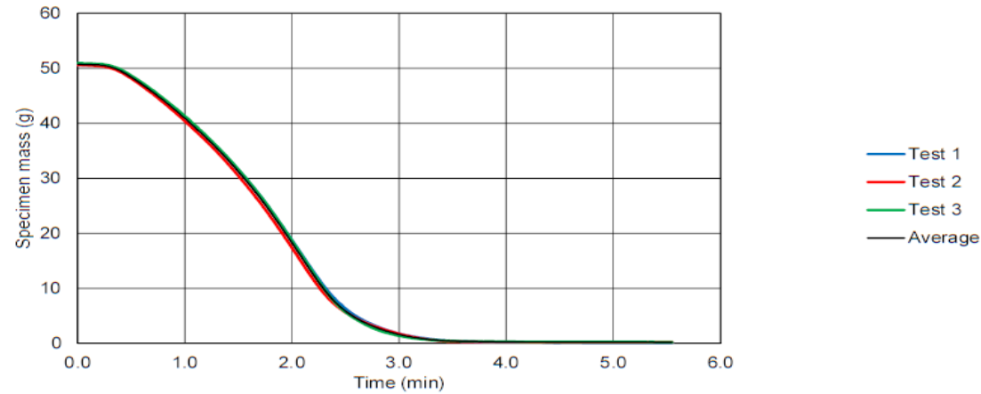
Specimen Mass
