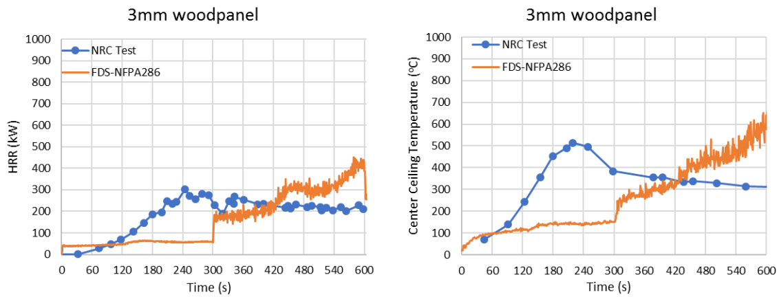
Figure D 5. Time history of HRR (left) and center ceiling temperature (right) of 3 mm wood panel tested in NFPA 286 room
