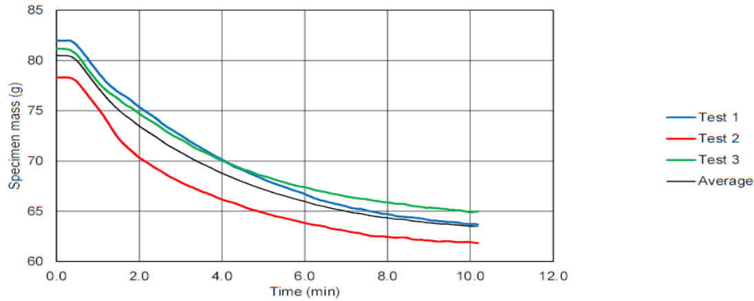
Specimen Mass
