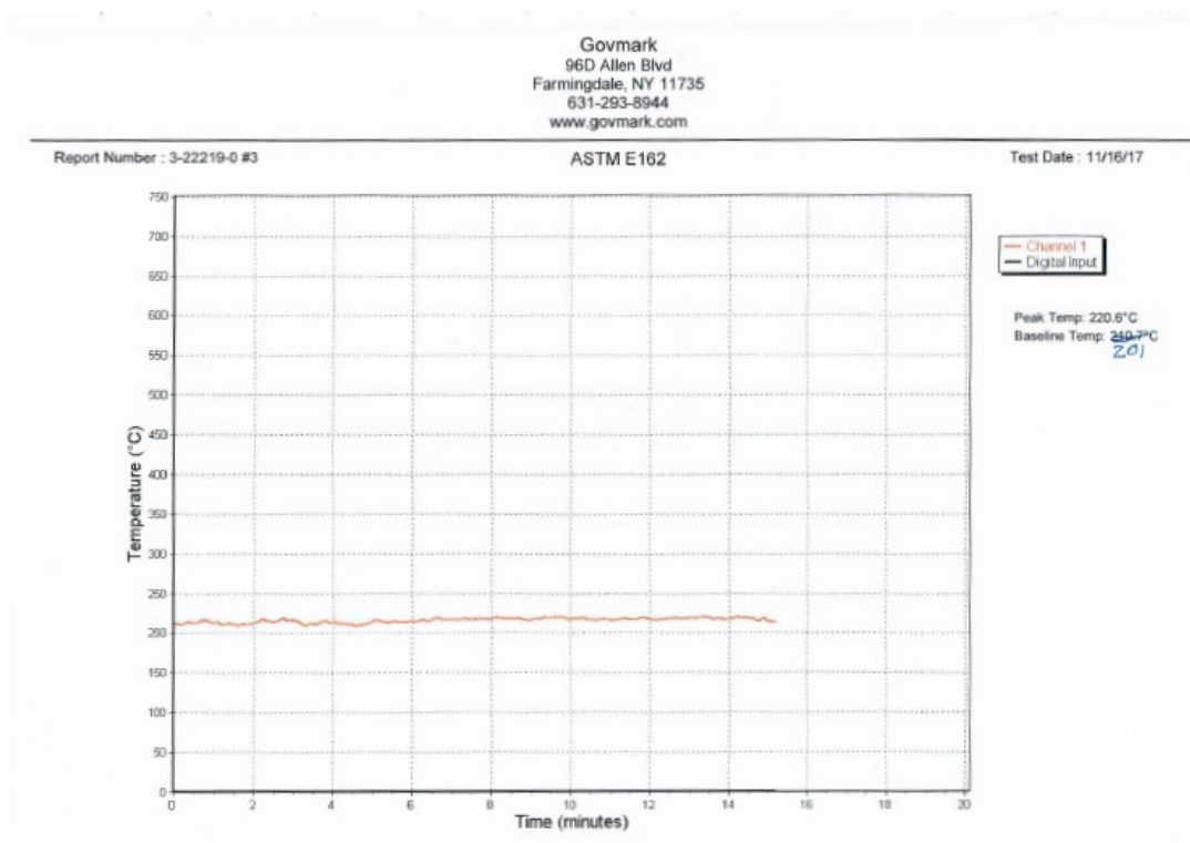
Figure B 2. All the radiant panel test results
