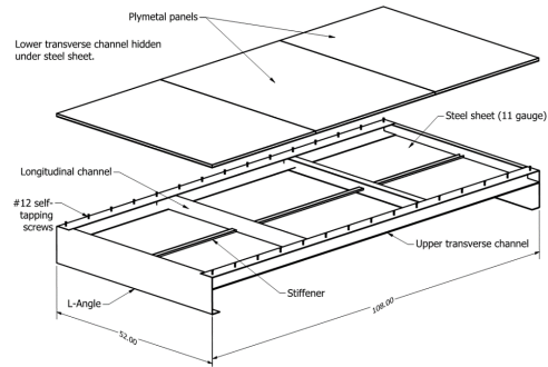
Figure 2: Reduced scale assembly Design 1, Test 3a
