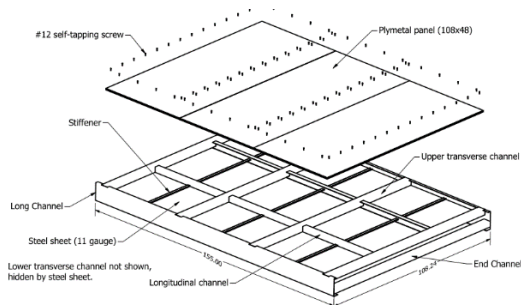
Figure 1: Full scale Assembly Design 1, Tests 1 and 2
