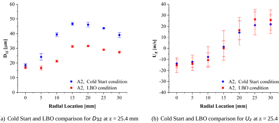
Figure 9: Comparisons of drop diameters and drop velocities for A-2 at Cold Start and LBO conditions. Cold Start : \Delta P/P = 3\% , T_{fuel}=T_{gas}=238\text{ K} . LBO : \Delta P/P = 3\% , T_{fuel}=322\text{ K} , and T_{gas}=394\text{ K}
