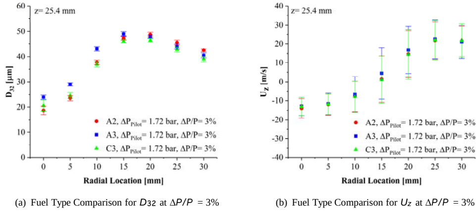
Figure 8: Comparisons of fuel type at \Delta P/P = 3\% , T_{fuel}=238\text{ K} , and T_{gas}=238\text{ K} on the 25.4 mm plane
