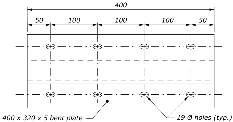
GUARDRAIL ANCHOR PLATE
