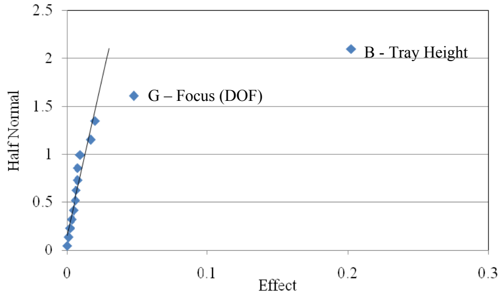
Figure 2.38. Half-normal plot of the aggregate height of the dark 9.5 mm (0.375 in) coarse aggregate used in Experiment 9.
