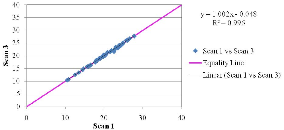
Figure 2.42. 25.0 mm (1.0 in) aggregate height measurement for Replicate Scan 1 vs. Scan 3.
