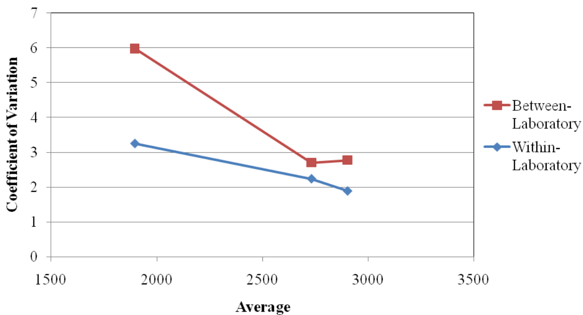
Figure 3.4. Coefficient of variation versus average angularity of 25.0 mm (1 in).
