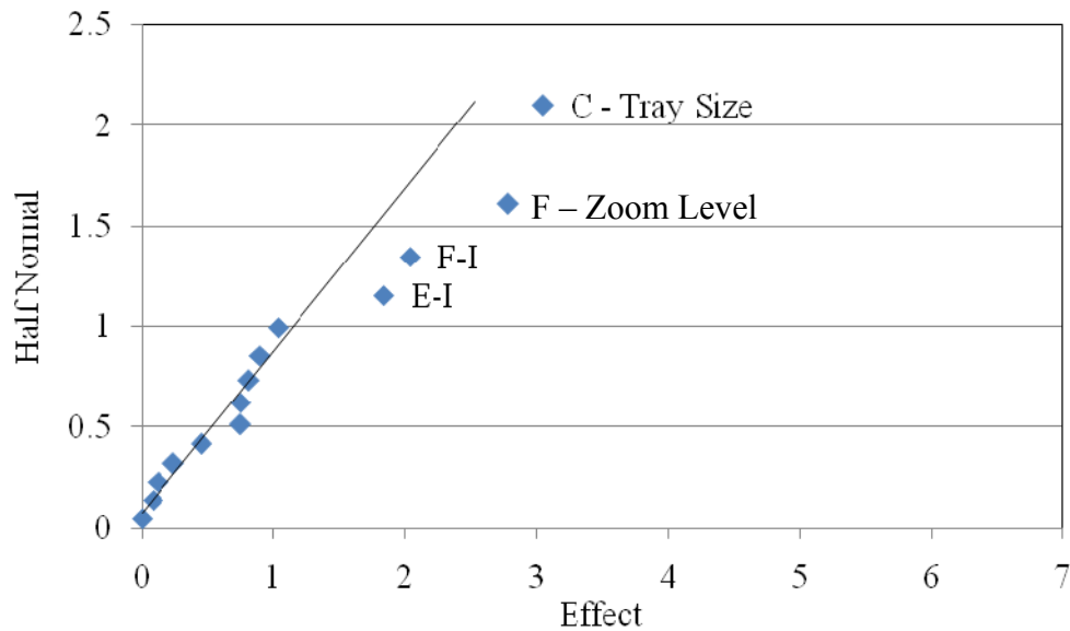
Figure 2.13. Half-normal plot of the texture of the light 4.75 mm (ASTM #4 sieve) coarse aggregate used in Experiment 5.
