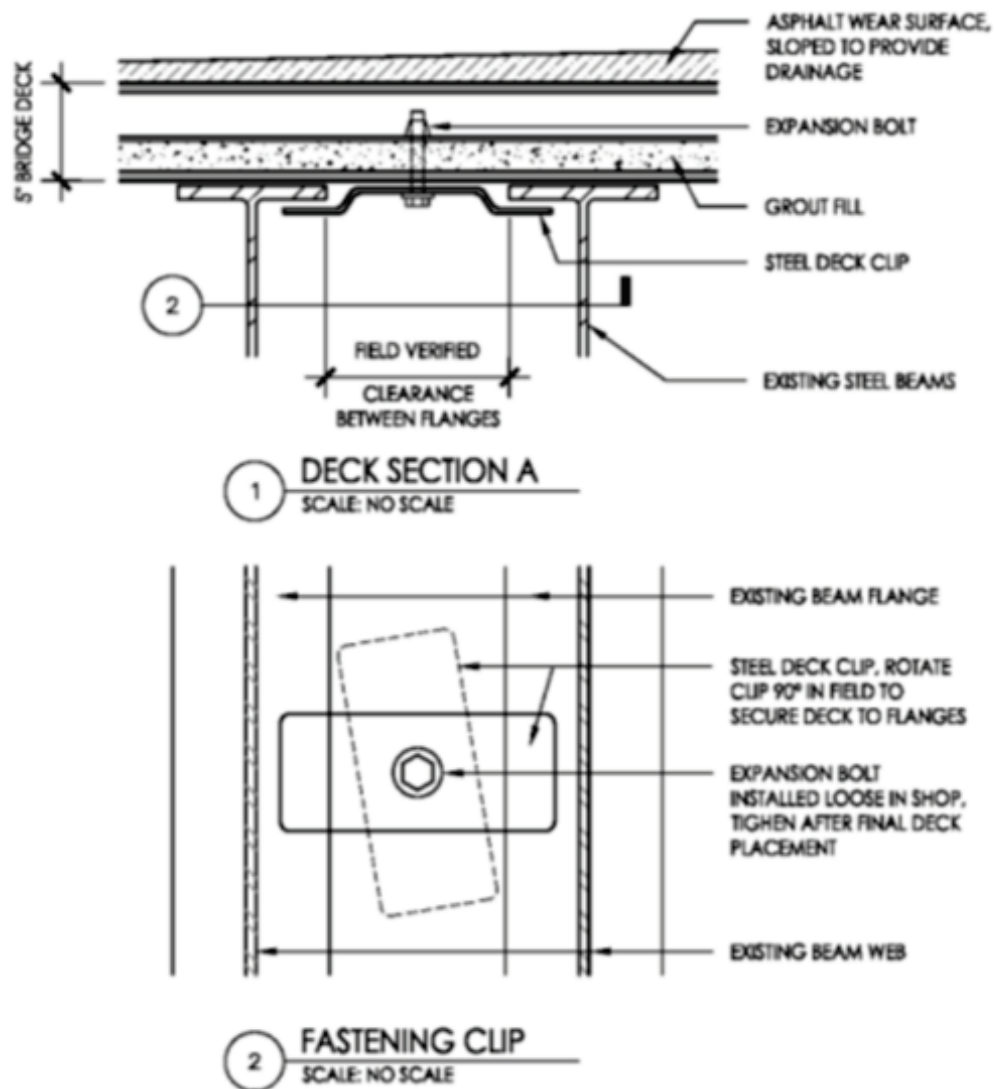
Figure 20. Diagram. Proposed connection detail.
