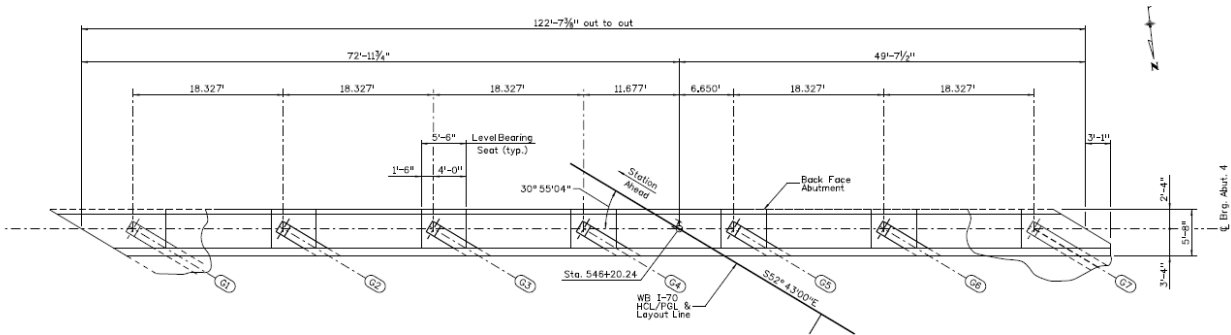
Figure 8. Diagram. GRS abutment plan view of abutment 4, E-17-AEK.
