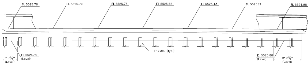
Figure 9. Diagram. GRS abutment elevation view of abutment 4, E-17-AEK.
