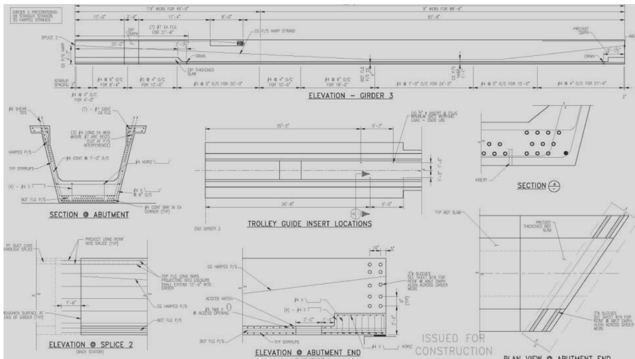
Figure 17. Drawing. U72 girders used on project (courtesy: Colorado DOT).
