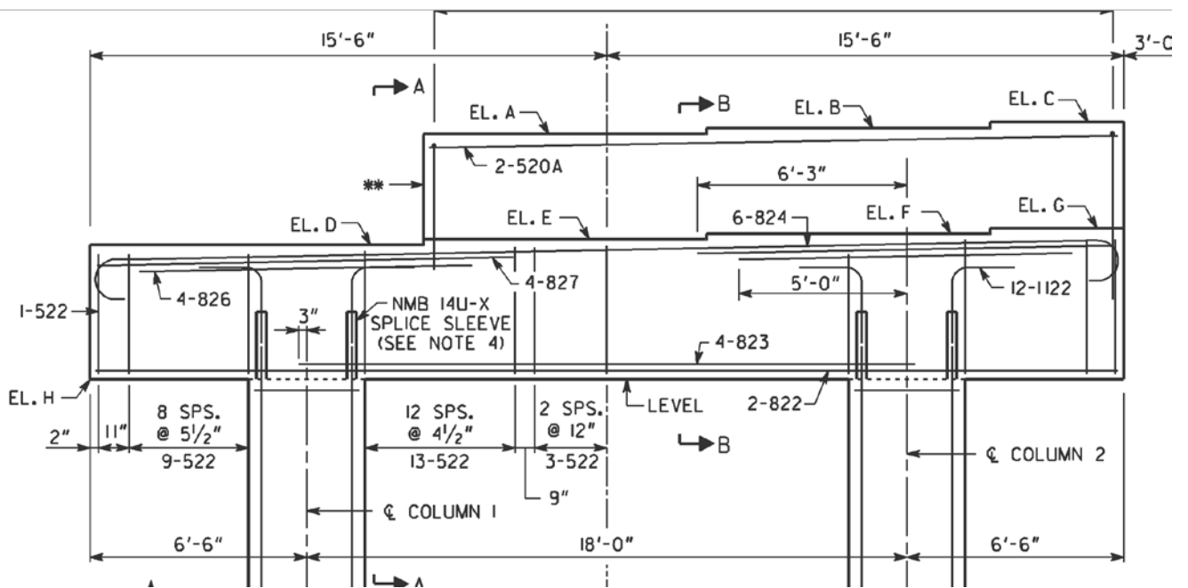
Figure 6. Typical intermediate bent detail.
