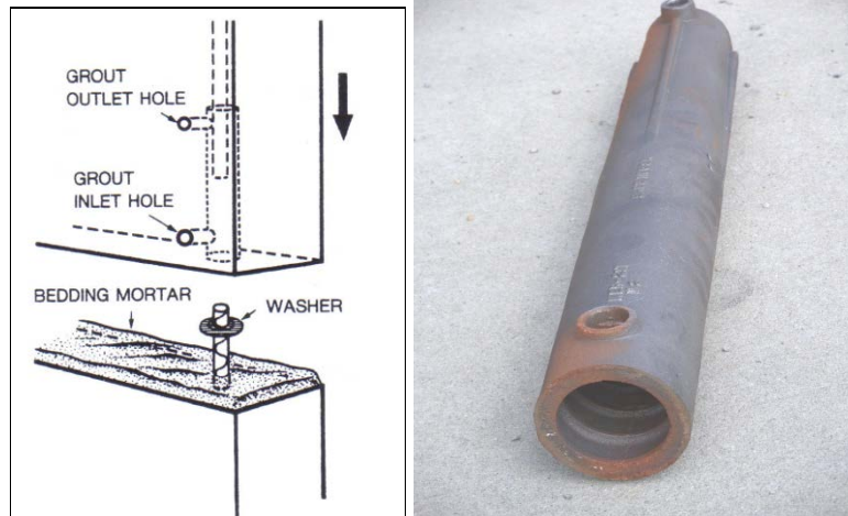
Figure 4. Coupler used to splice rebar to connect the footings, columns, and pier caps.
