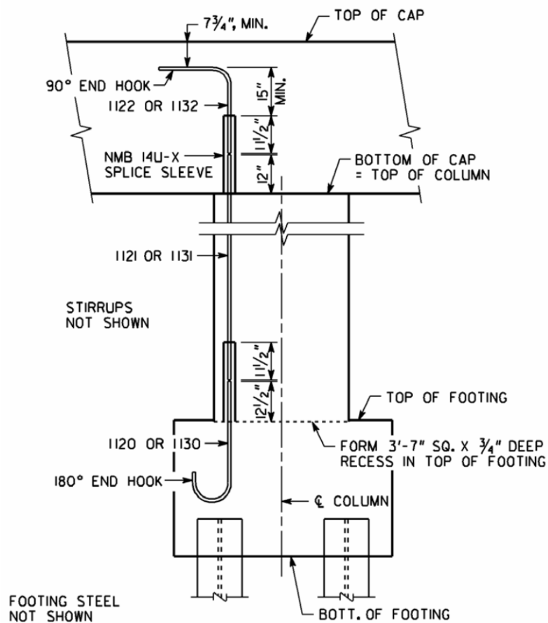
Figure 4. Coupler used to splice rebar to connect the footings, columns, and pier caps.
