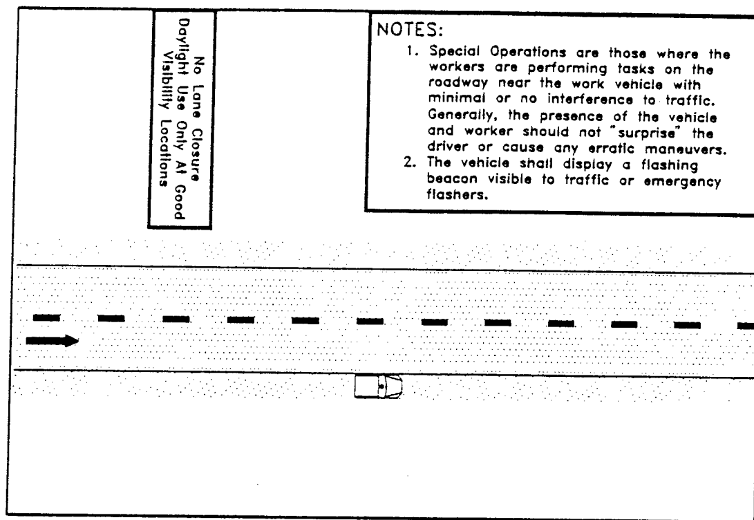
Figure 6 - Special Traffic Control Zone with Work Vehicle Off the Traveled Roadway High-Speed Street or Highway
