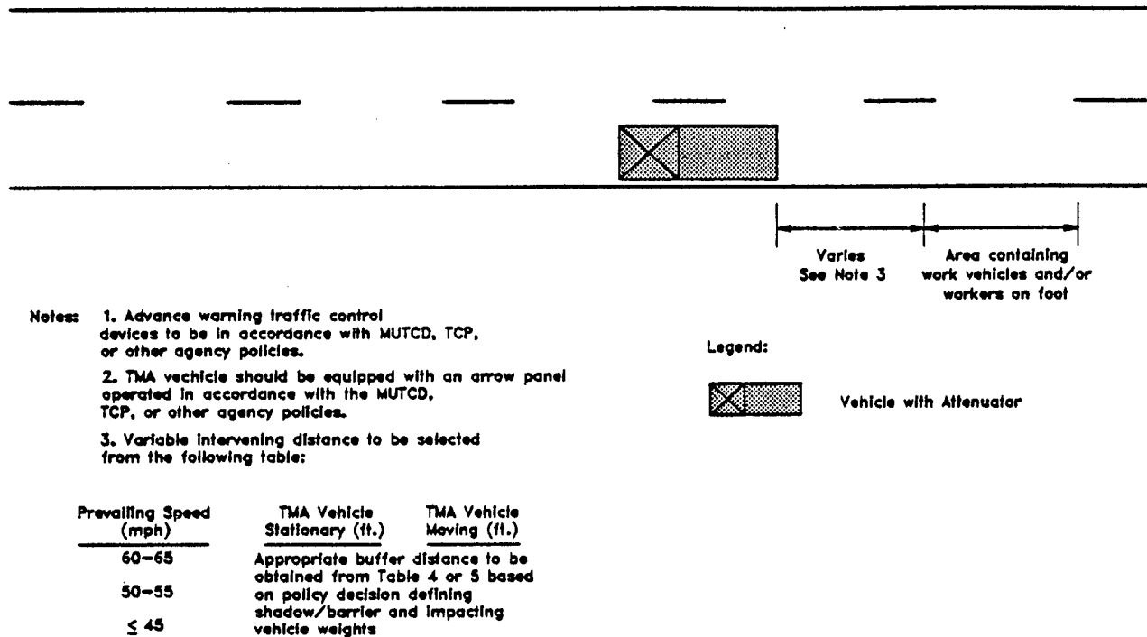
Figure 1 - Work area outside formal lane closure. (One-way or two-way)
