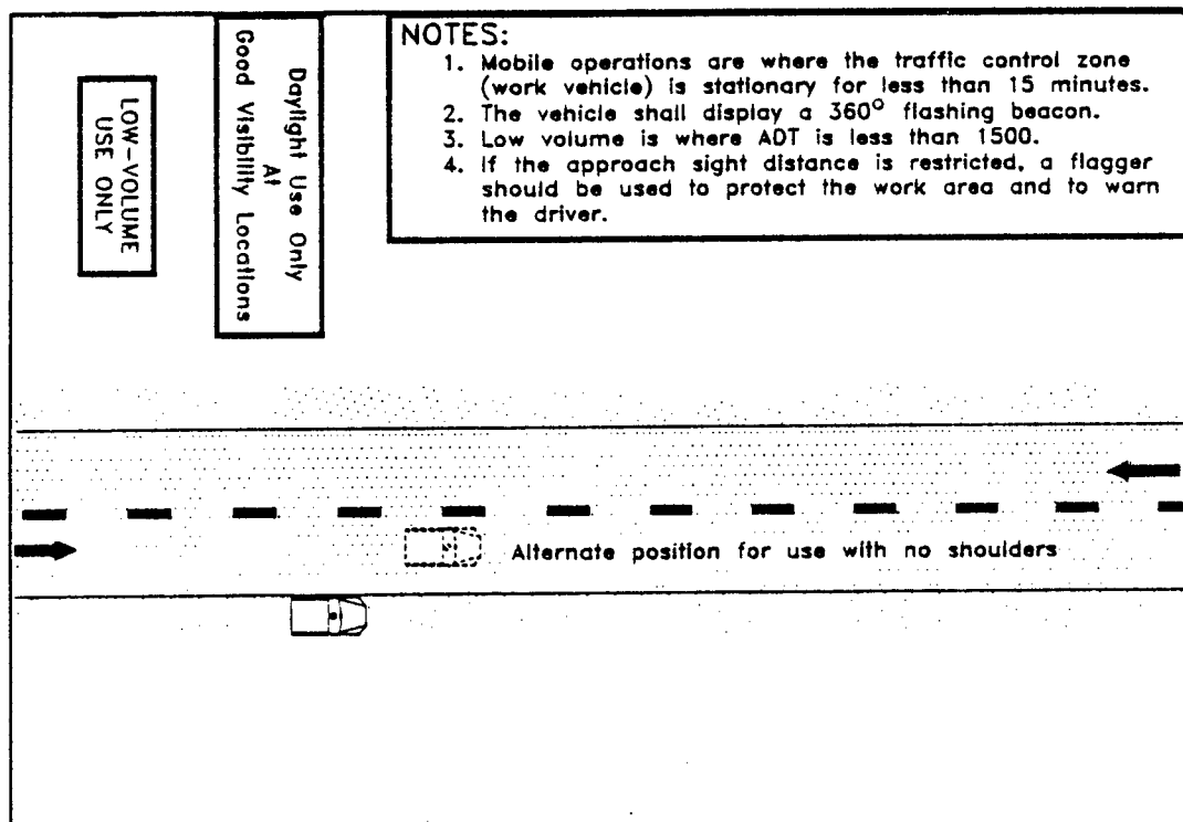
Figure 4 - Lane Closure for Mobile Traffic Control Zones High-Speed Two-Lane Two-Way Low-Volume Street or Highway
