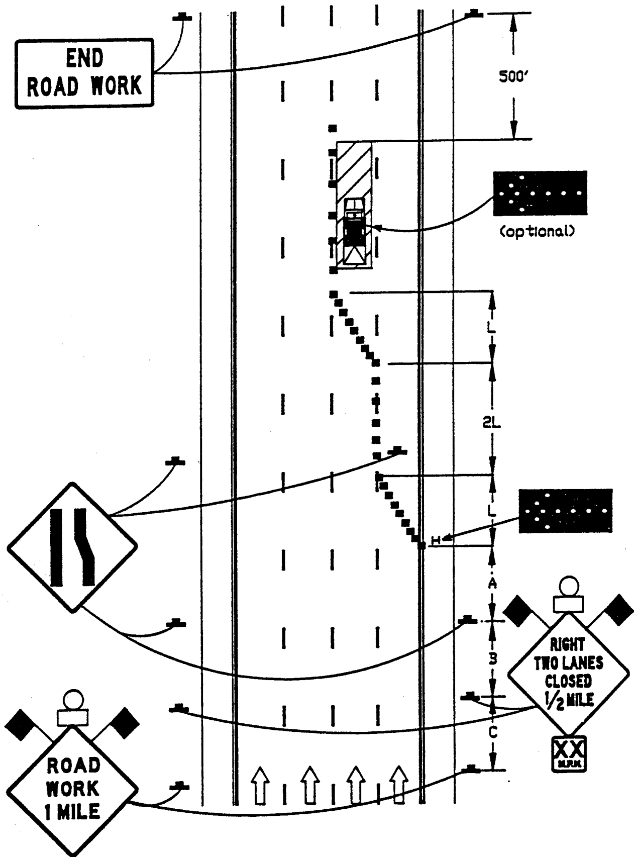
Figure 4 - Multiple lane closure.
