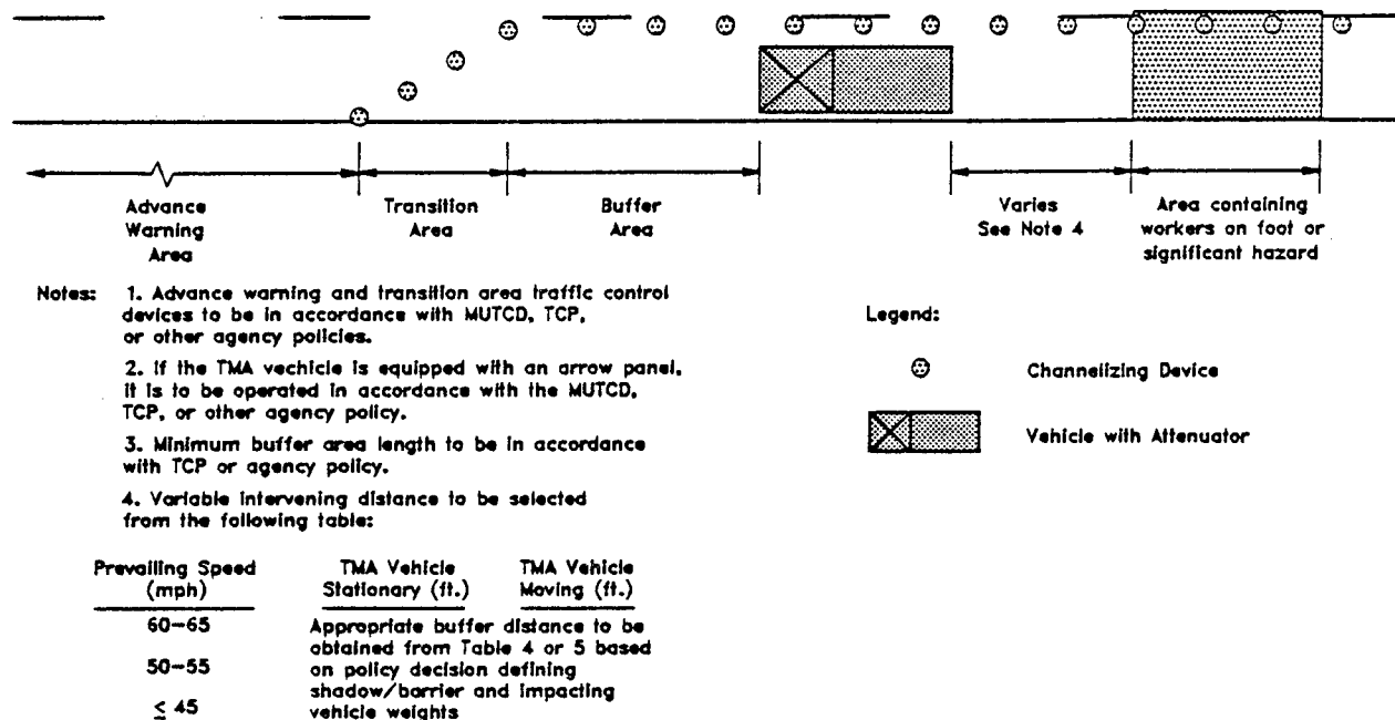
Figure 3 - Workers on foot or significant hazard within formal lane closure. (One-way or two-way)
