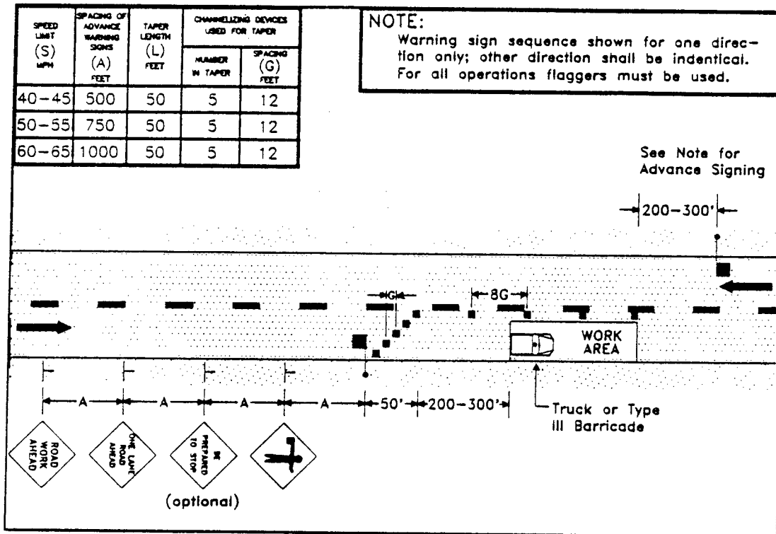
Figure 1 - Lane Closure High-Speed Two-Lane Two-Way Low-Volume Street or Highway
