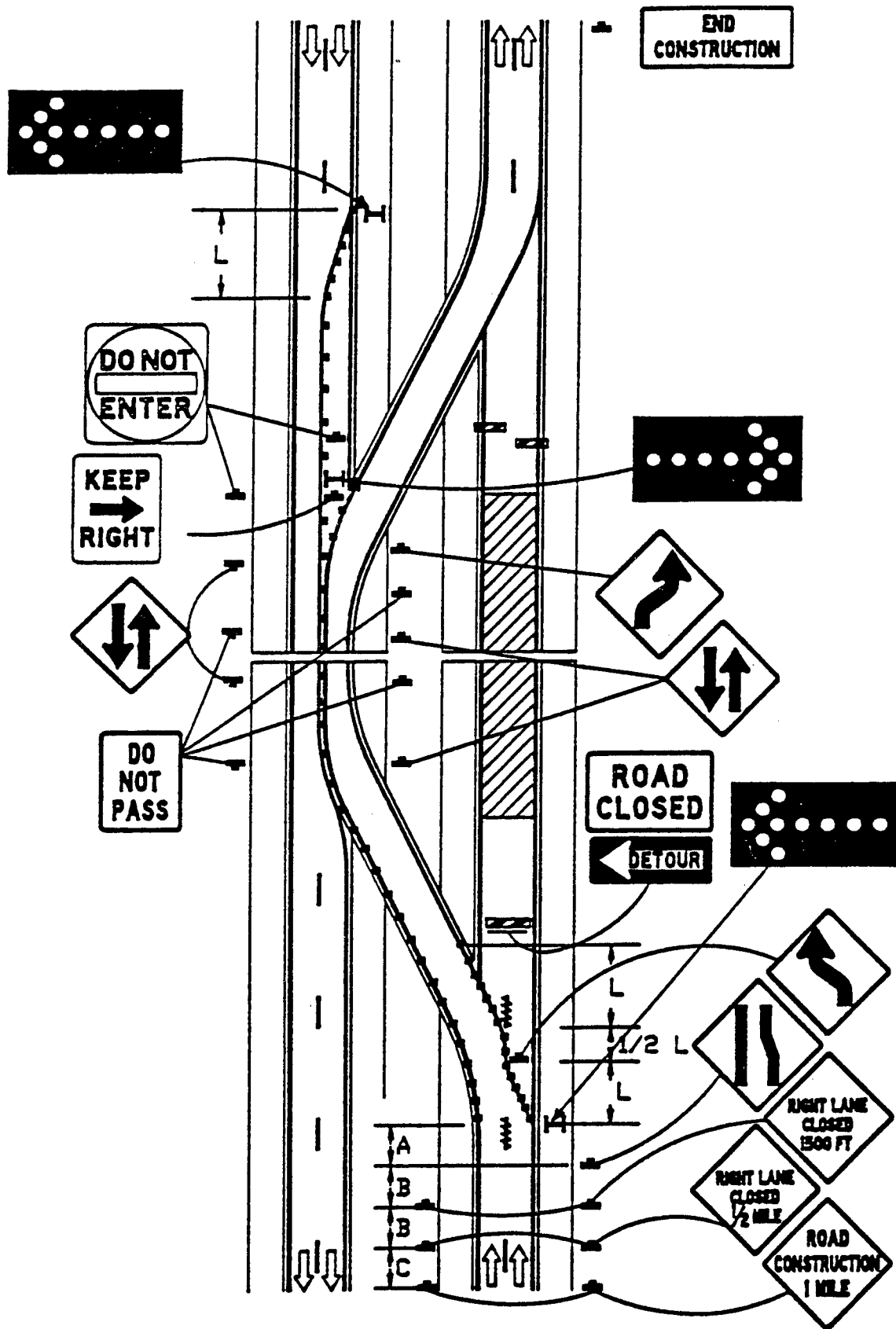
Figure 7 - Bypass two-lane two-way operation.
