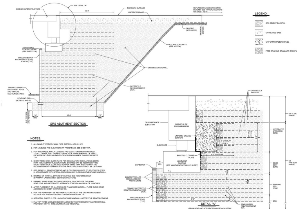
Figure 11. Diagram. Schematic of the eastbound and median abutments.
