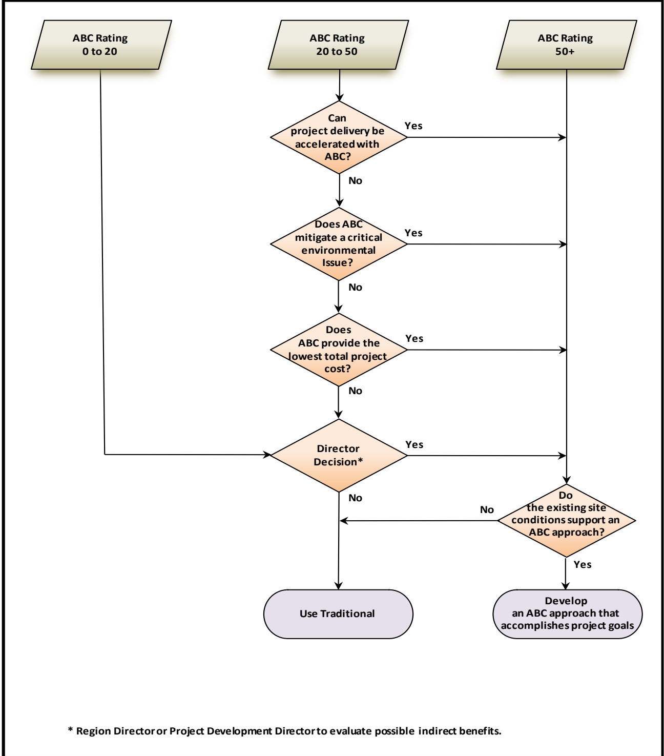
Figure 8. Chart. UDOT standard ABC decision flowchart (source: UDOT).
