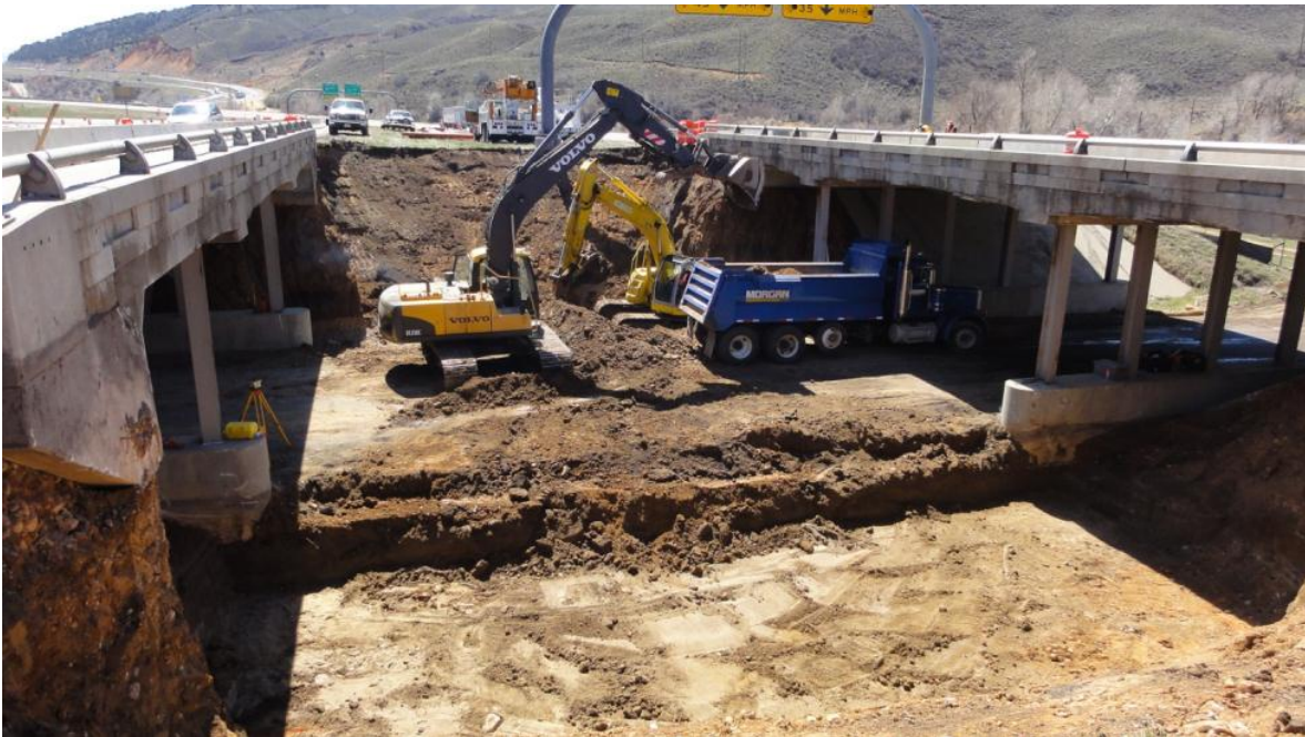
Figure 20. Photo. Roadway excavation for the median crossover bridge.
