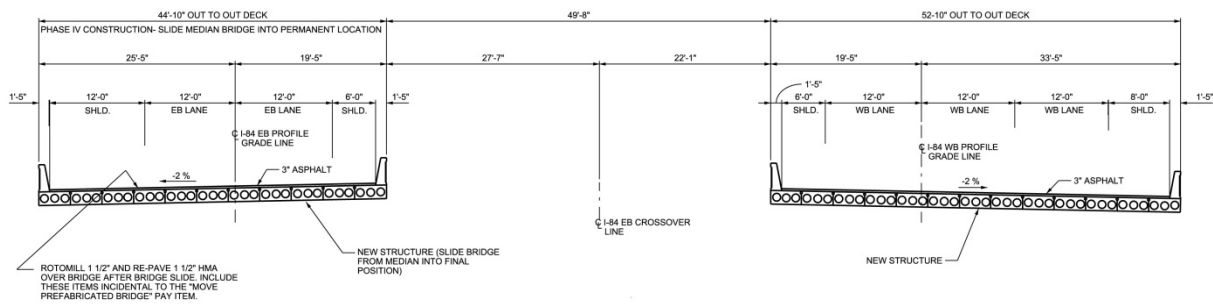
Figure 5. Diagram. Cross-section details of the new bridge (courtesy: UDOT).
