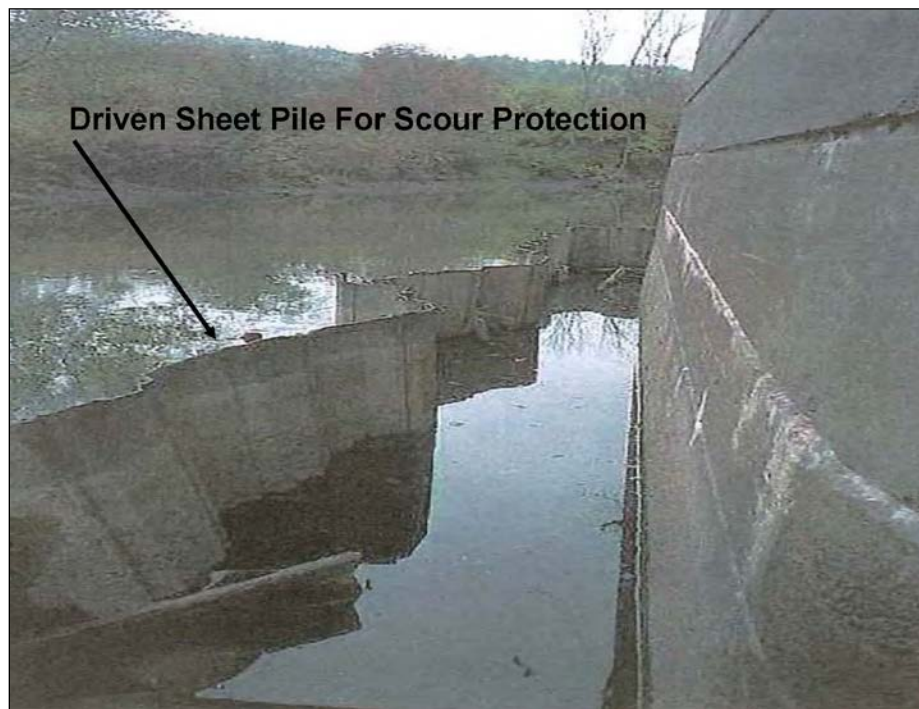
Figure 4. Scour protection at the existing structure.
