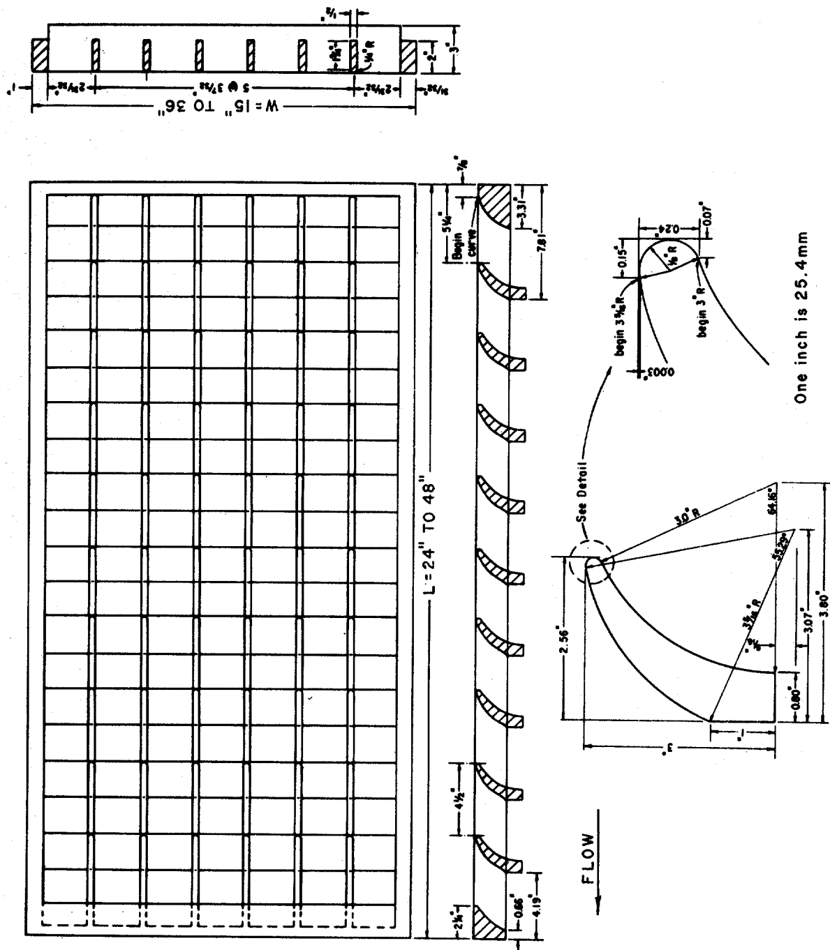
Figure 10. Curved vane grate.
