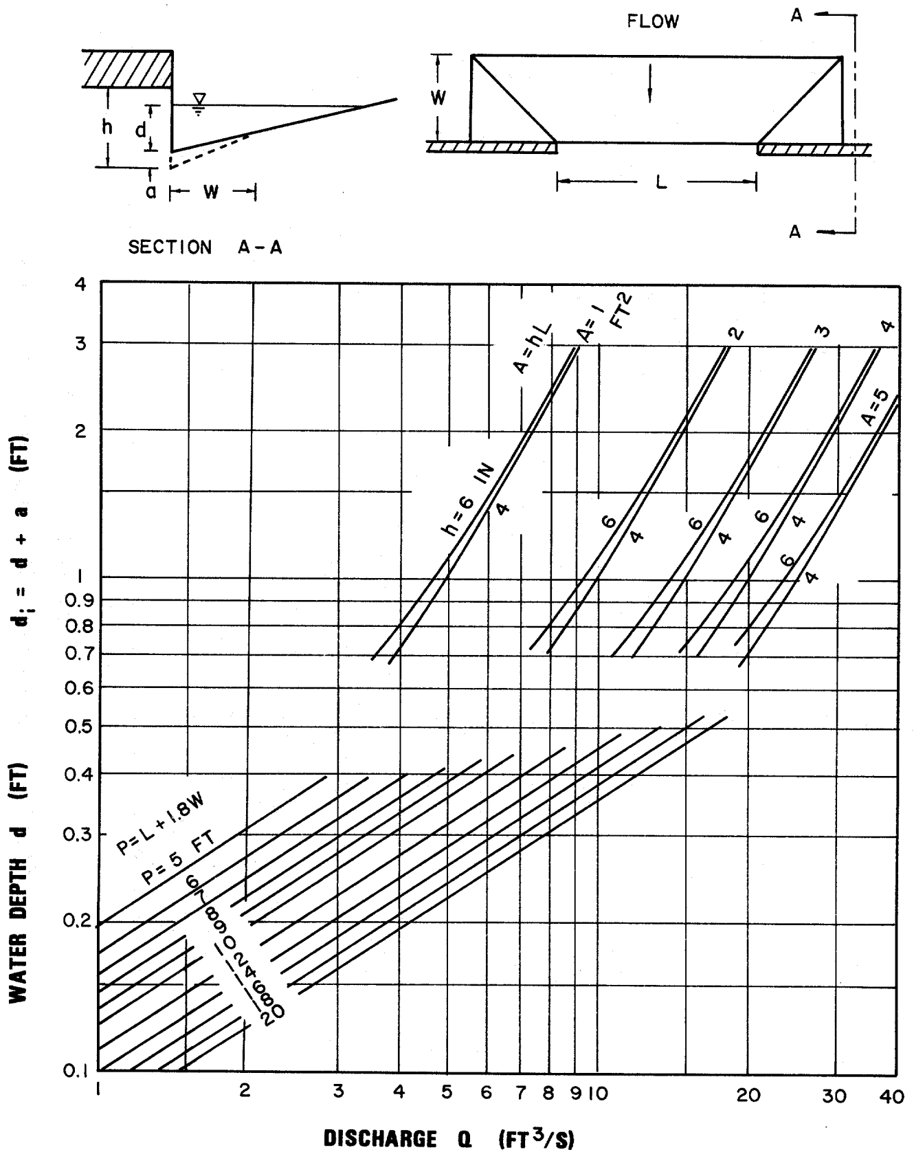
CHART 12. Depressed curb-opening inlet capacity in sump locations.
