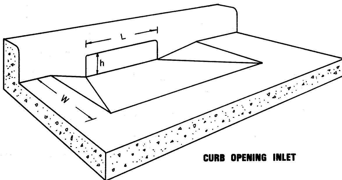
Figure 6. Perspective views of grate and curb-opening inlets.
