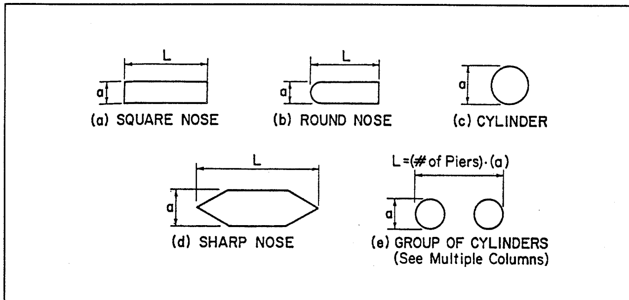
Figure 7. Common pier shapes.
