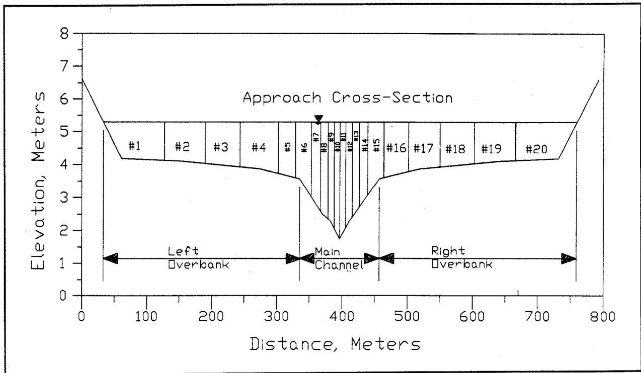
Figure 18. Equal conveyance tubes of approach section.
