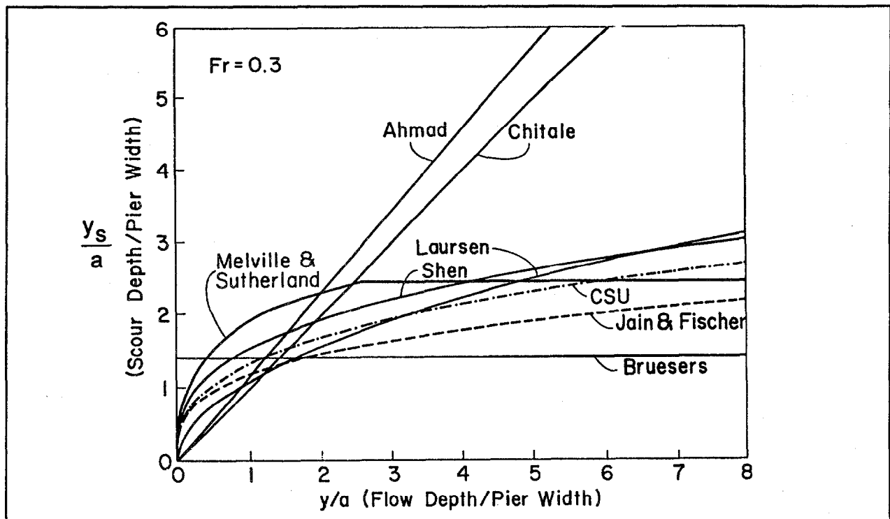
Figure 4. Comparison of scour equations for variable depth ratios ( y/a ) (after Jones). (44)
