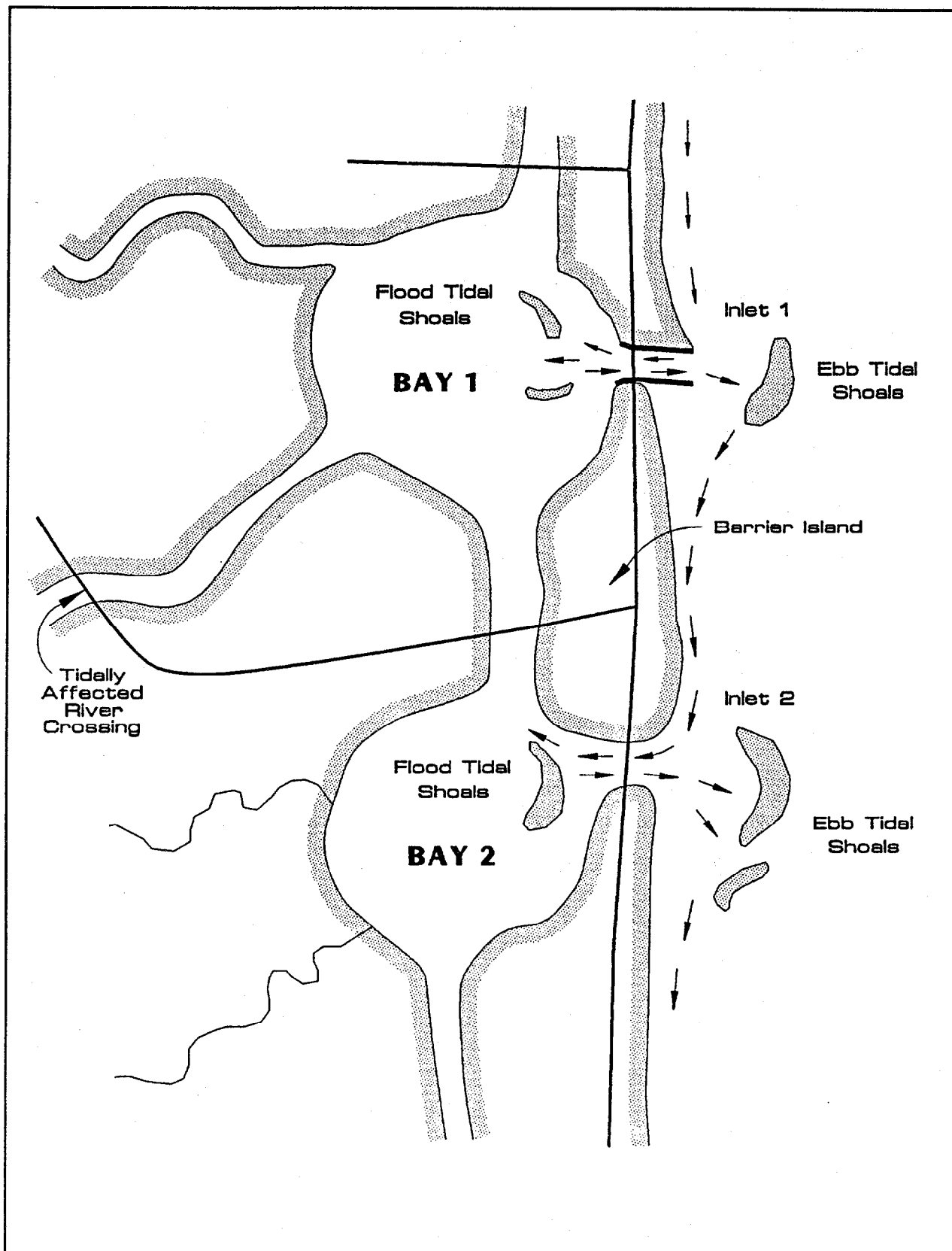
Figure 25. Sediment transport in tidal inlets (after Sheppard). (66)
