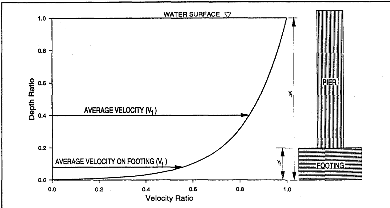
Figure 8. Definition sketch for velocity and depth on exposed footing.
