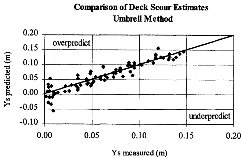
Figure 7. Predicted versus measured deck scour using Umbrell's equation for clear-water conditions.
