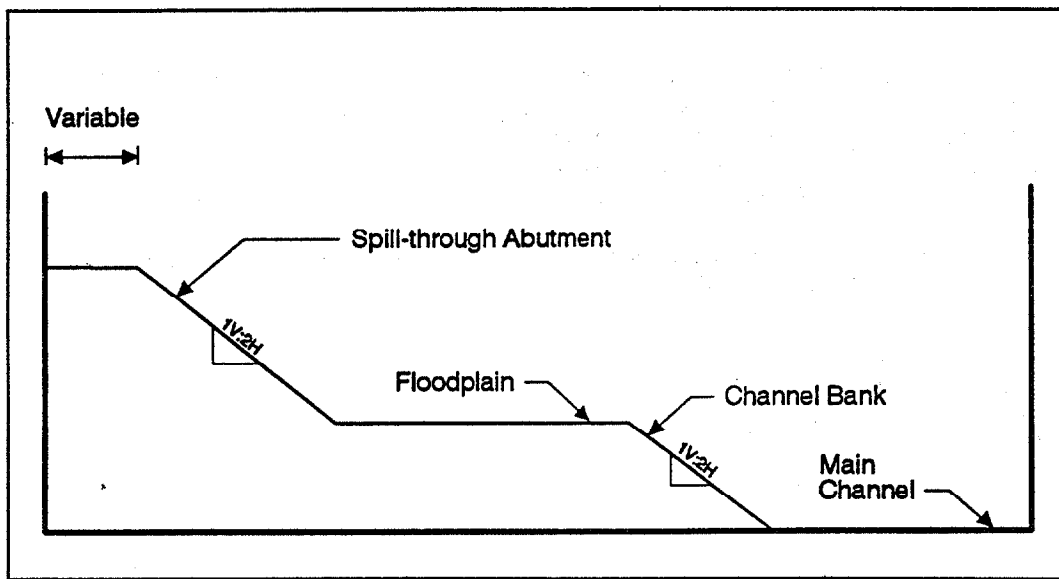
Figure 27. Section view of a typical setup of spill-through abutment on a floodplain with adjacent main channel. (81)
