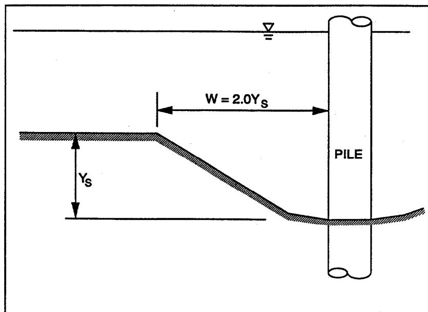
Figure 13. Topwidth of scour hole.
