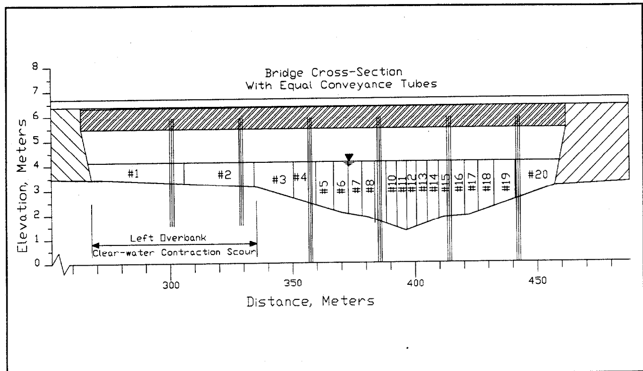
Figure 19. Equal conveyance tubes of bridge section.
