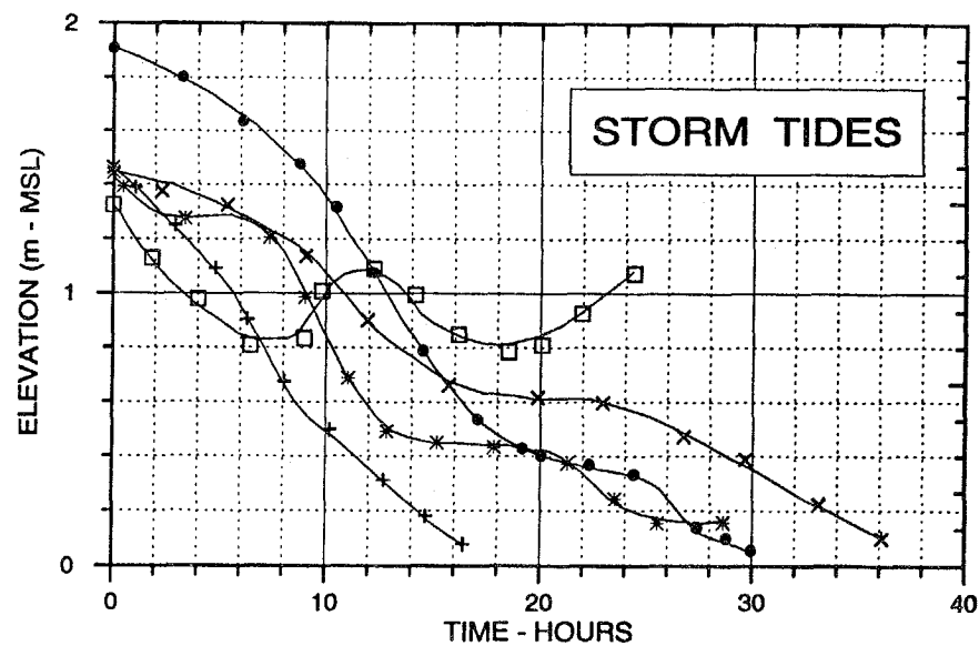
Figure 26. Tidal parameters for example problem 1.
