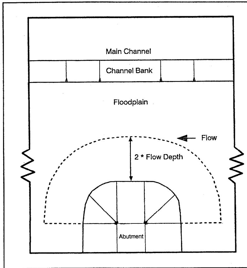
Figure 29. Plan view of the extension of rock riprap apron. (83)
