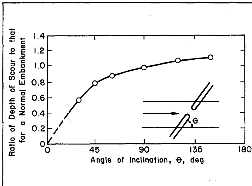
Figure 16. Adjustment of abutment scour estimate for skew.
