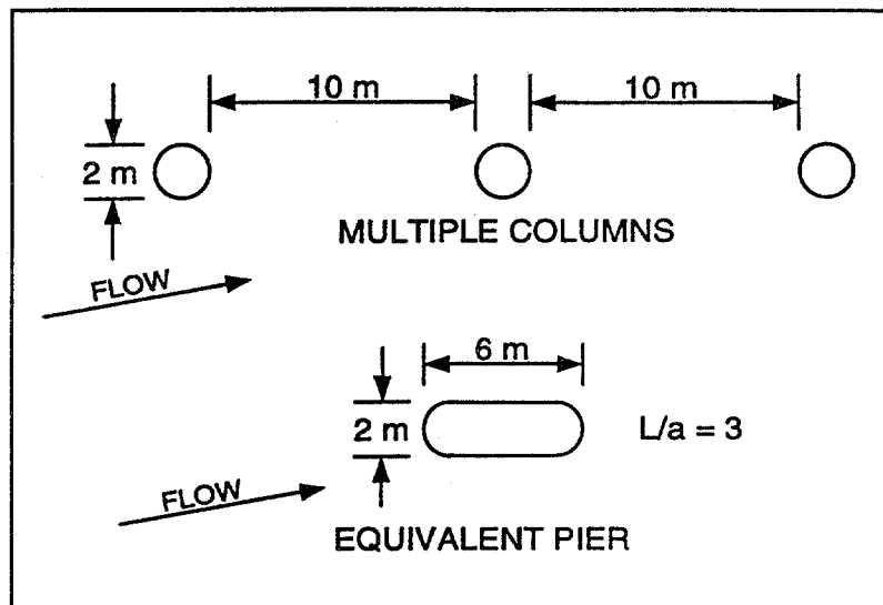
Figure 11. Multiple columns skewed to the flow.
