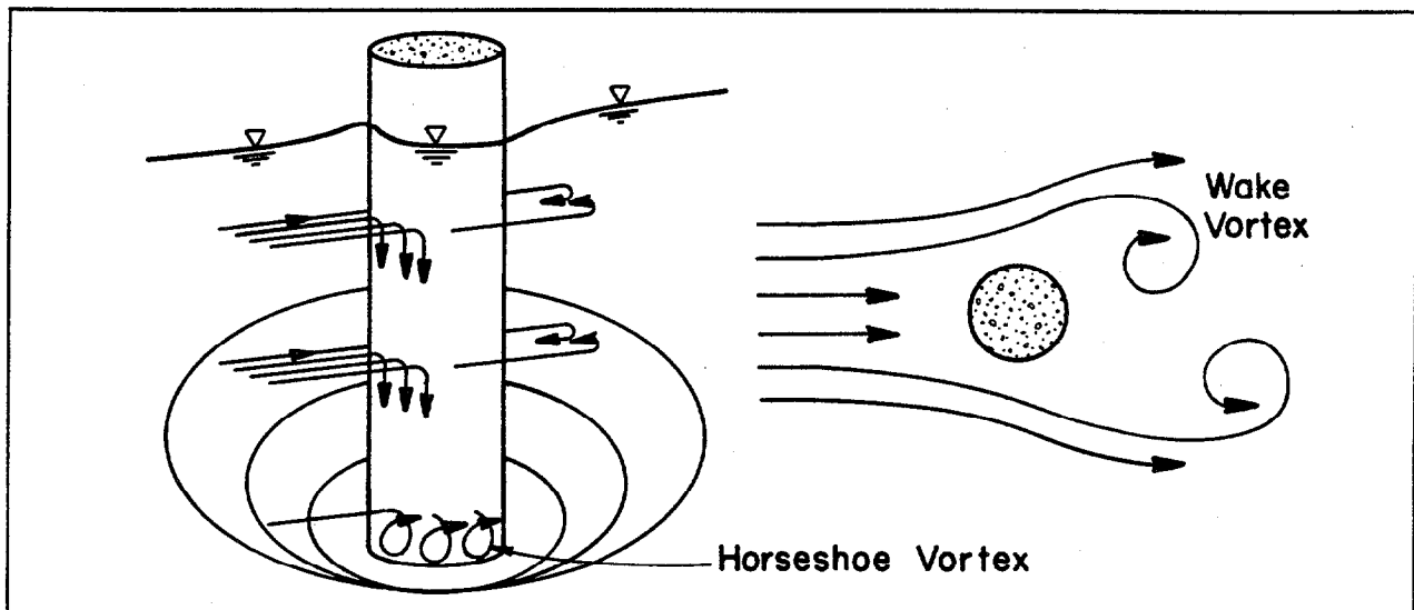
Figure 1. Schematic representation of scour at a cylindrical pier.
