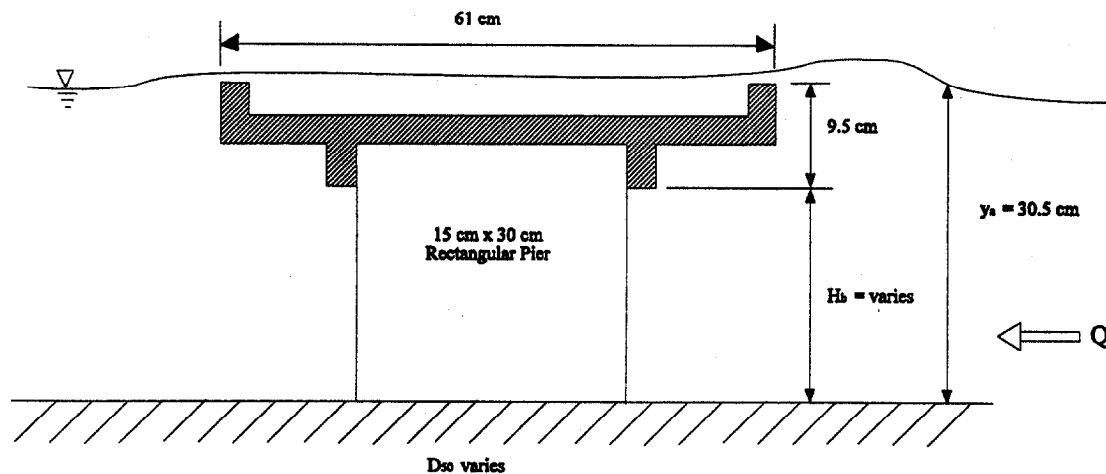
Figure 2. Federal Highway Administration test configuration.
