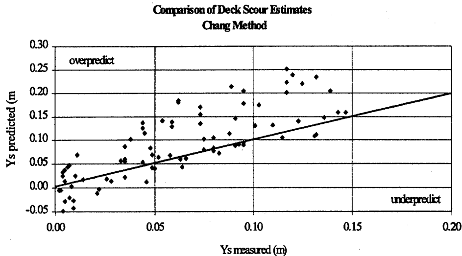
Figure 8. Predicted versus measured deck scour using Chang's correction coefficients.
