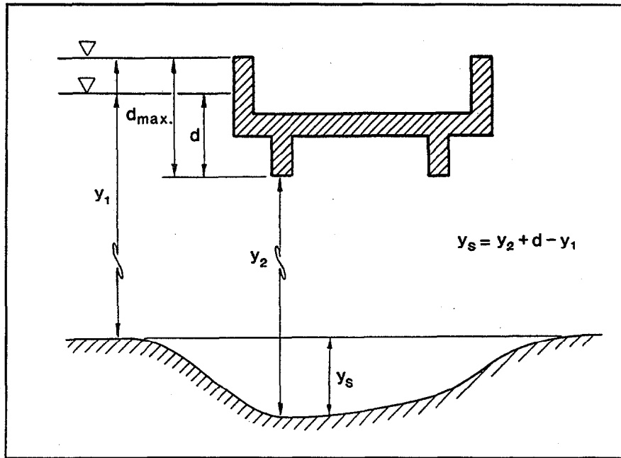
Figure 12. Definition sketch of vertical contraction scour resulting from pressure flow (see appendix B).
