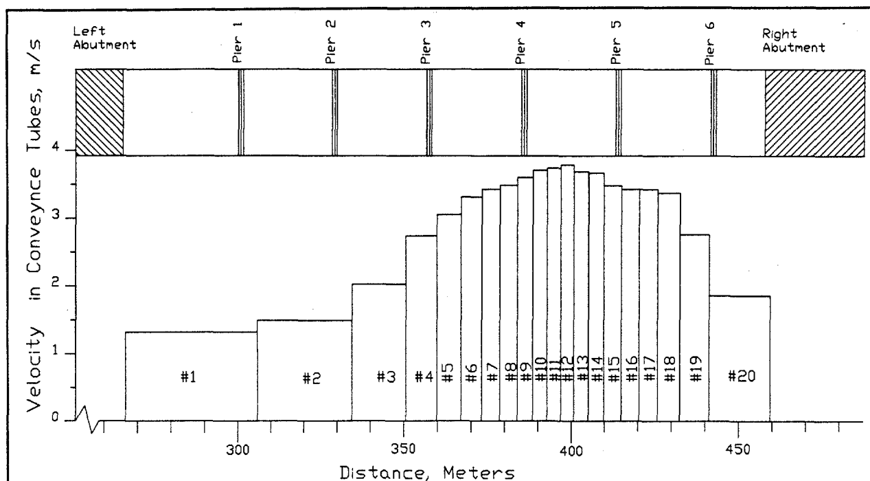
Figure 21. Velocity distribution at bridge crossing.
