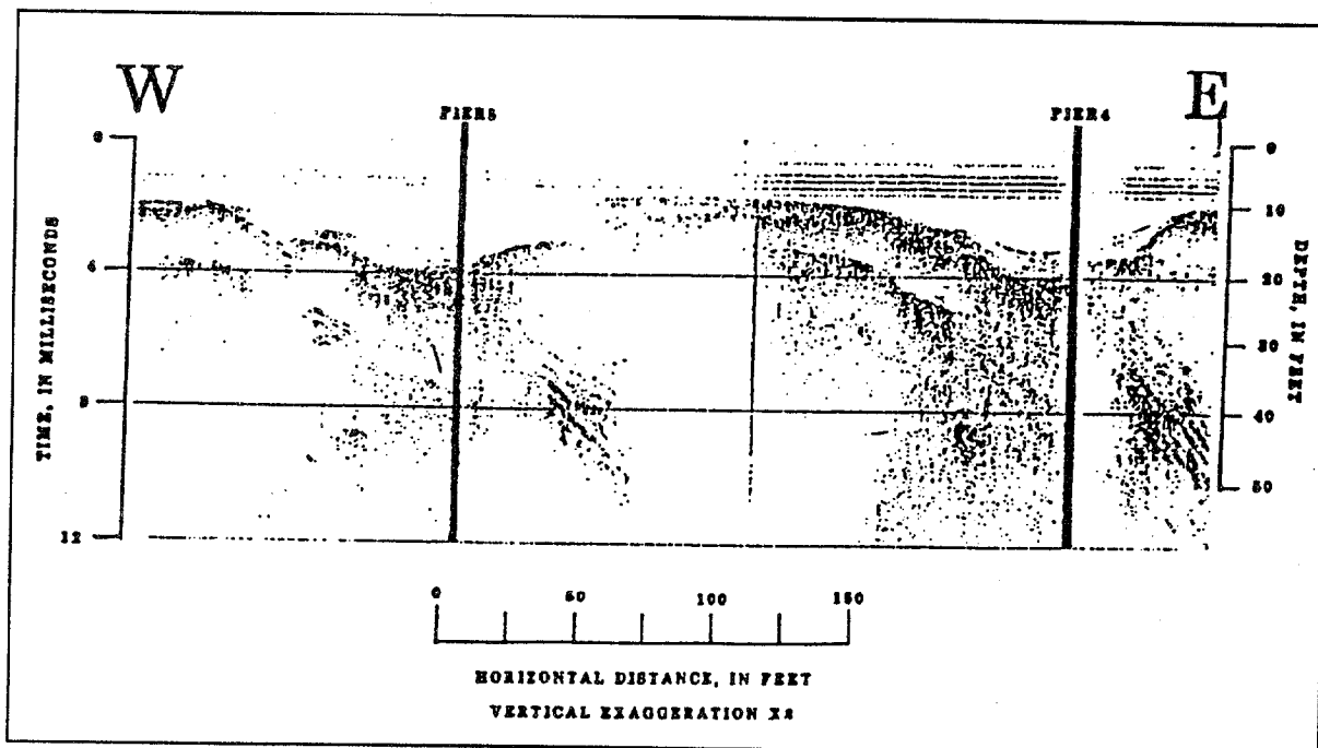
Figure F.6. Example of 14 KHz tuned transducer.
