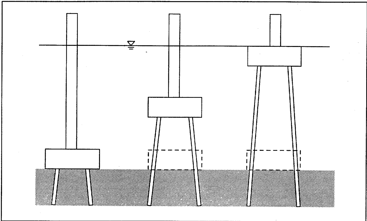
Figure 10. Pile cap placed at the streambed, in the flow, or at the water surface.
