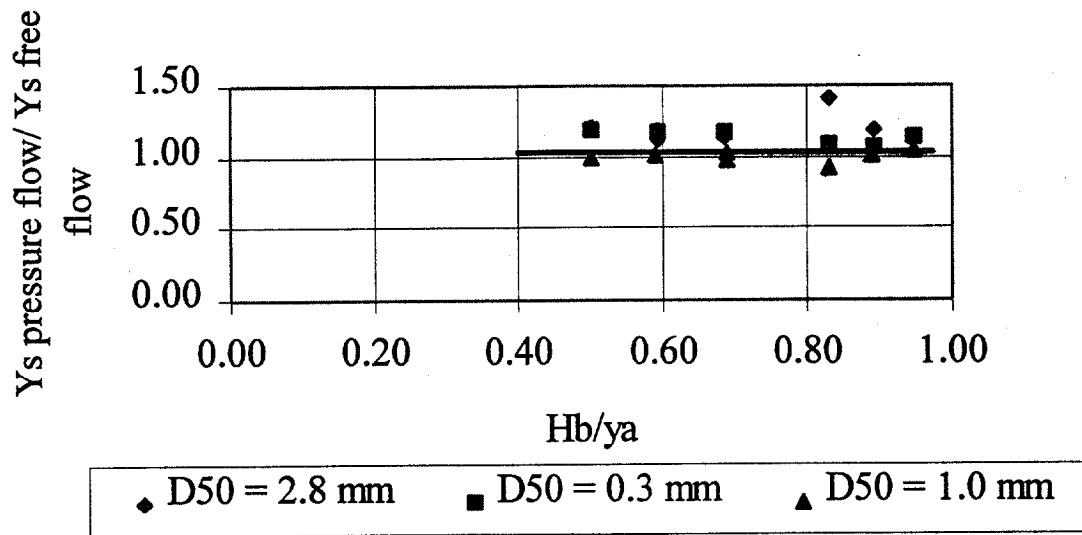
Figure 4. Pressure flow pier scour ratio, FHWA data.
