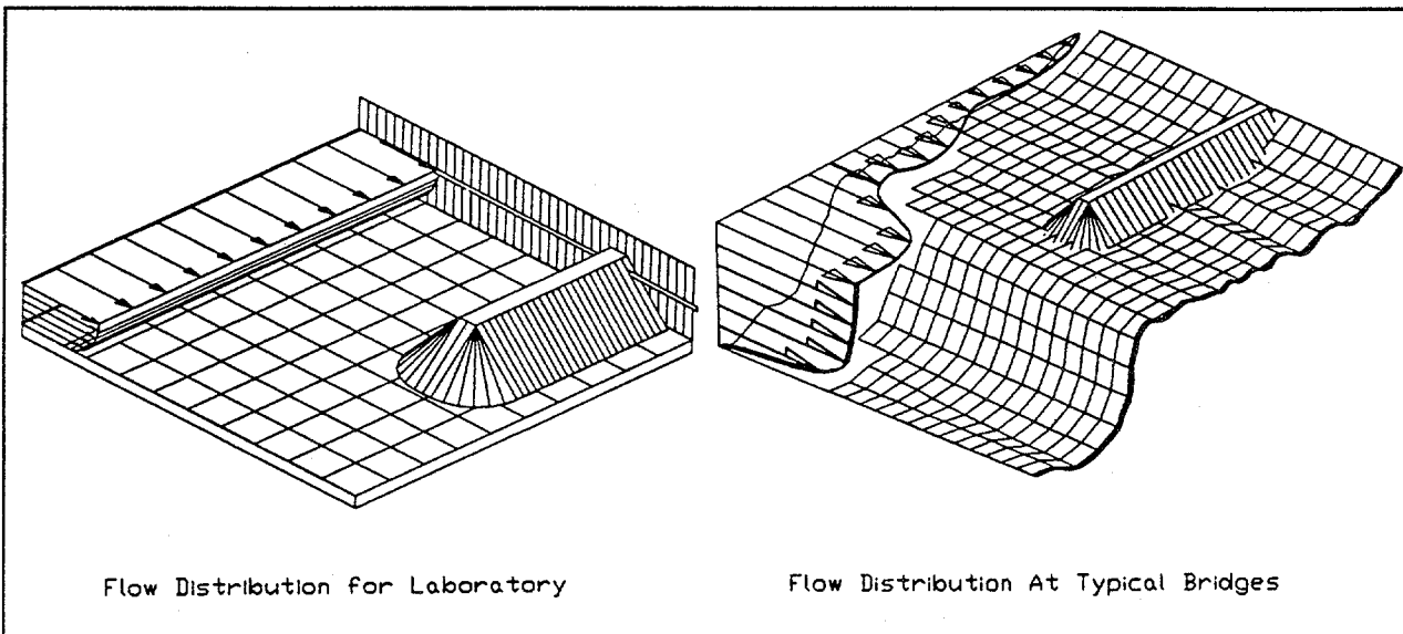
Figure 14. Comparison of laboratory flow characteristics to field flow conditions.
