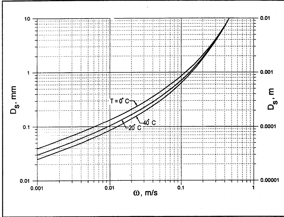
Figure 3. Fall velocity of sand-sized particles.
