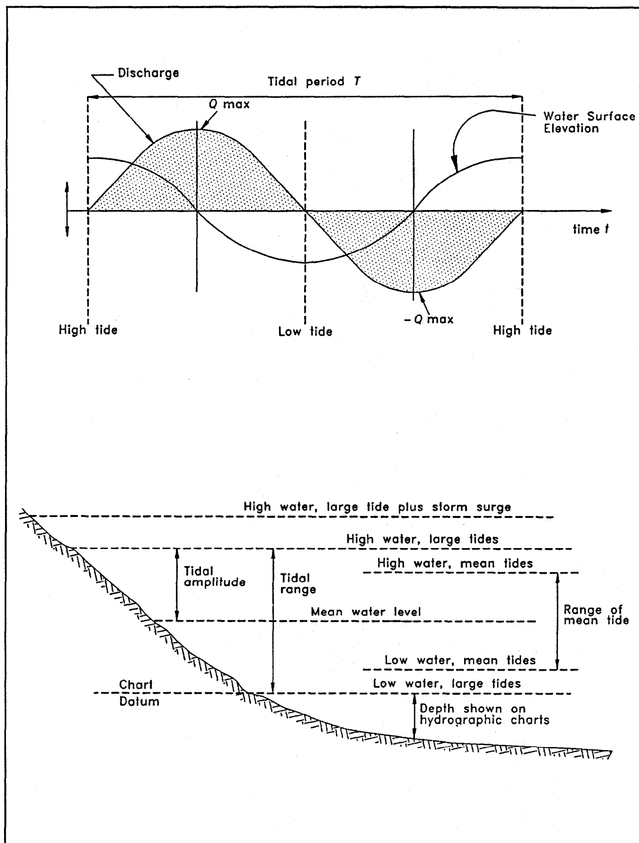
Figure 24. Principal tidal terms (after Neill). (63)
