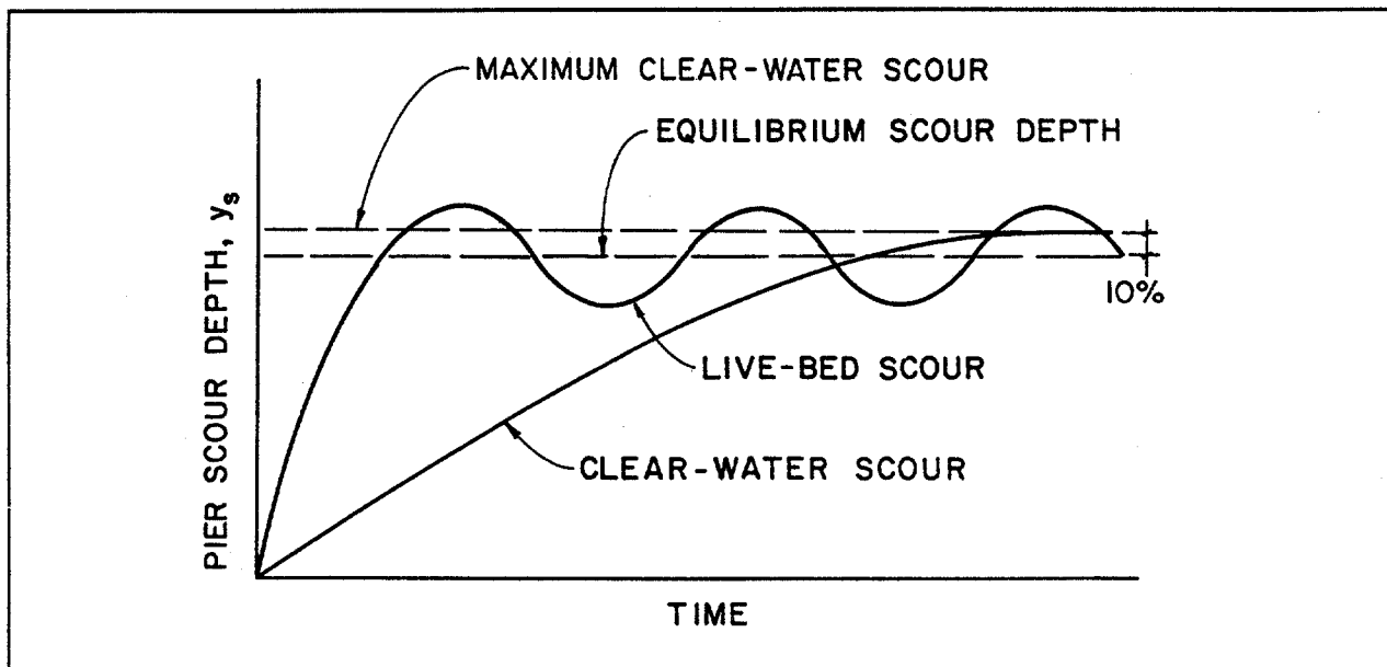
Figure 2. Illustrative pier scour depth in a sand-bed stream as a function of time. (not to scale)
