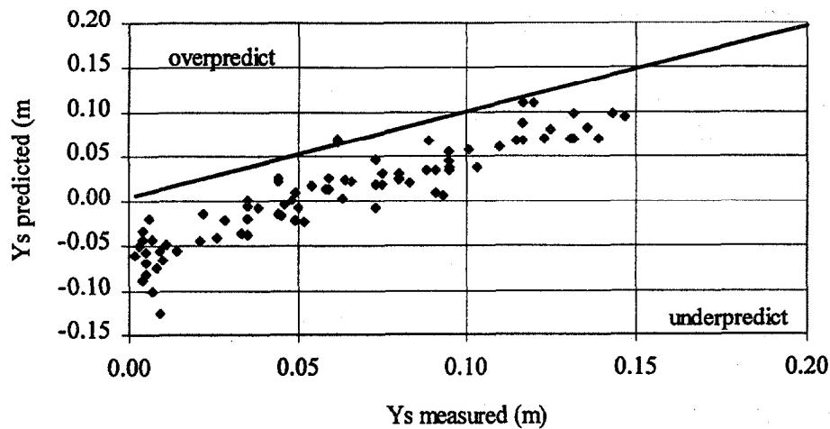
Figure 5. Comparison of deck scour estimates, simplified procedure.
