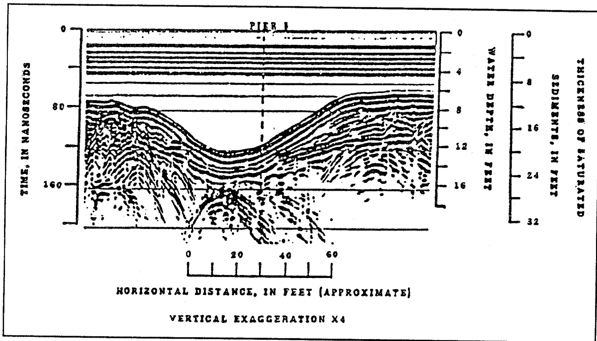
Figure F.5. Example of ground penetrating radar.
