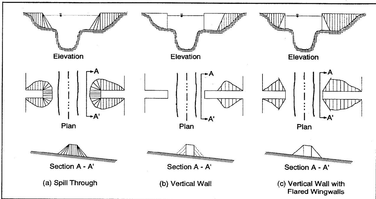
Figure 15. Abutment shape.
