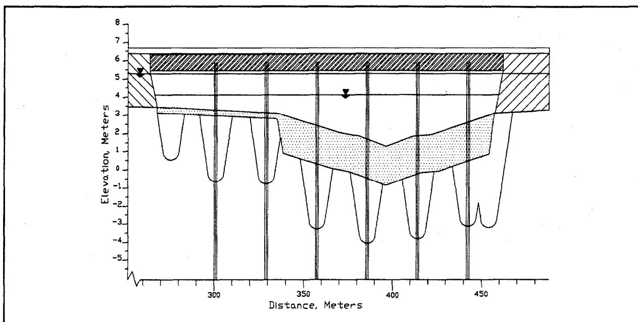
Figure 22. Plot of total scour for example problem.
