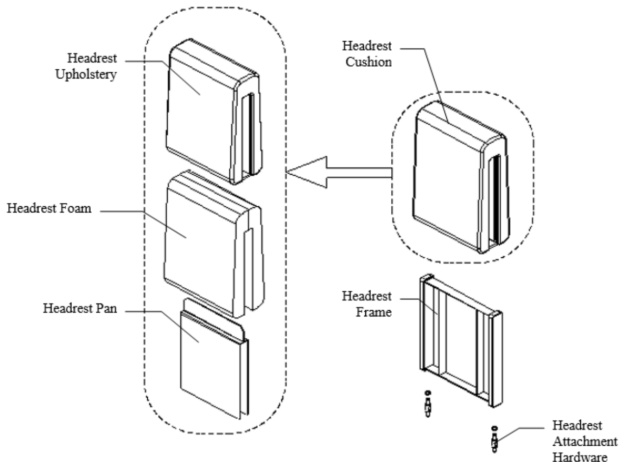
Figure 46. Headrest components
