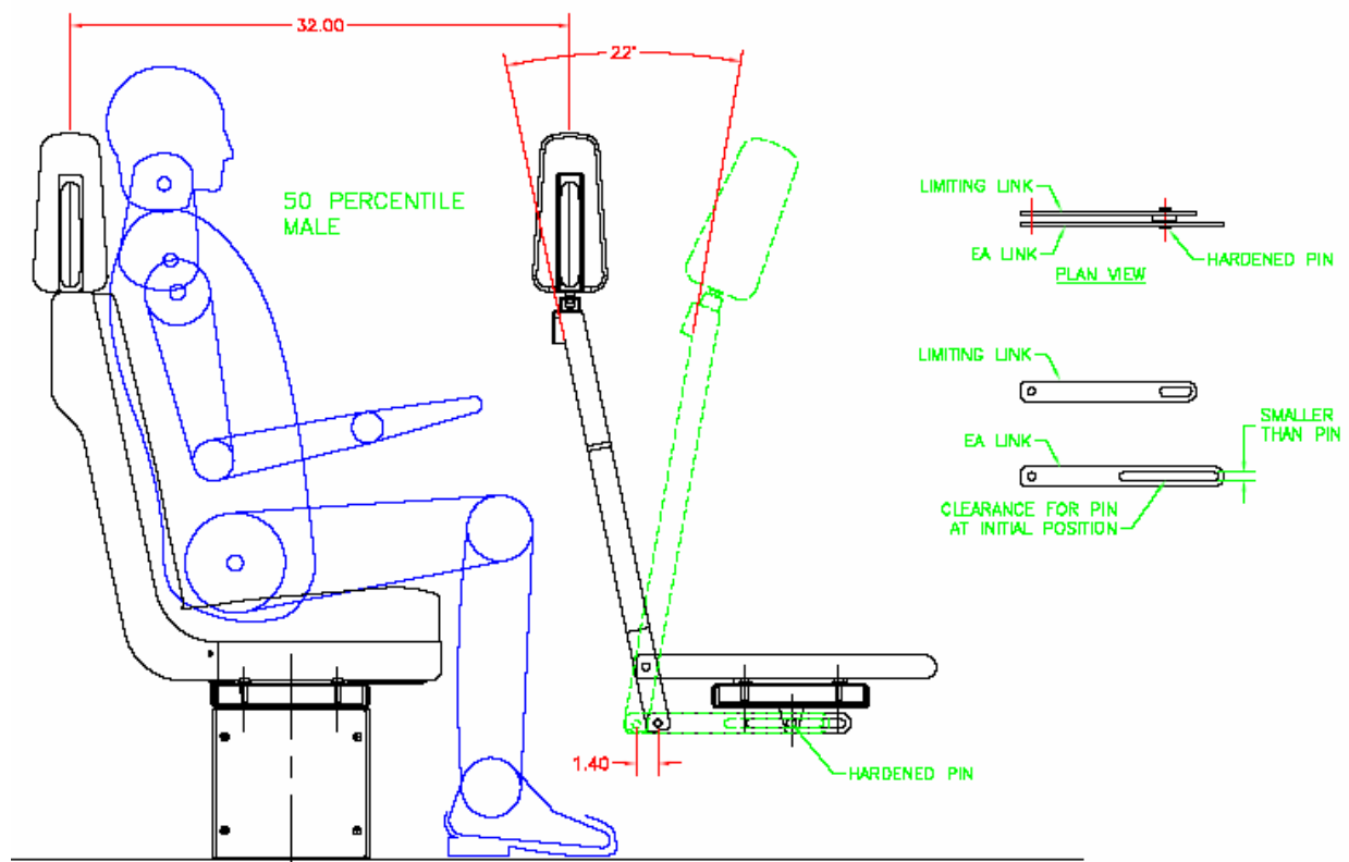
Figure 6. Example of an energy-absorbing mechanism placed below the seat pan
