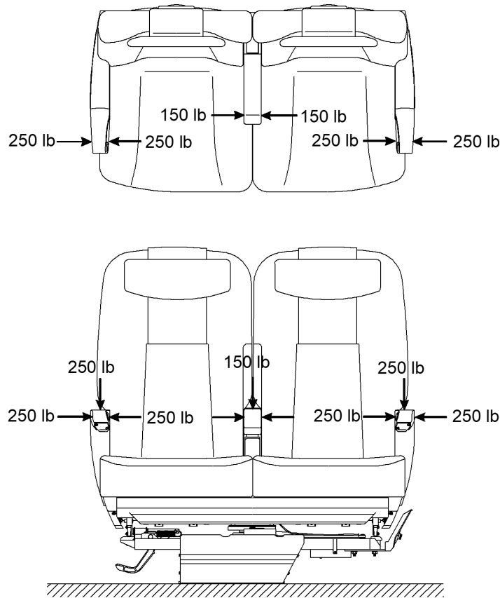
Figure A.5. Armrest strength test loading conditions
