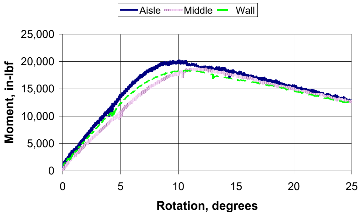
Figure 63. Moment vs. rotation behavior from the FF head load test
