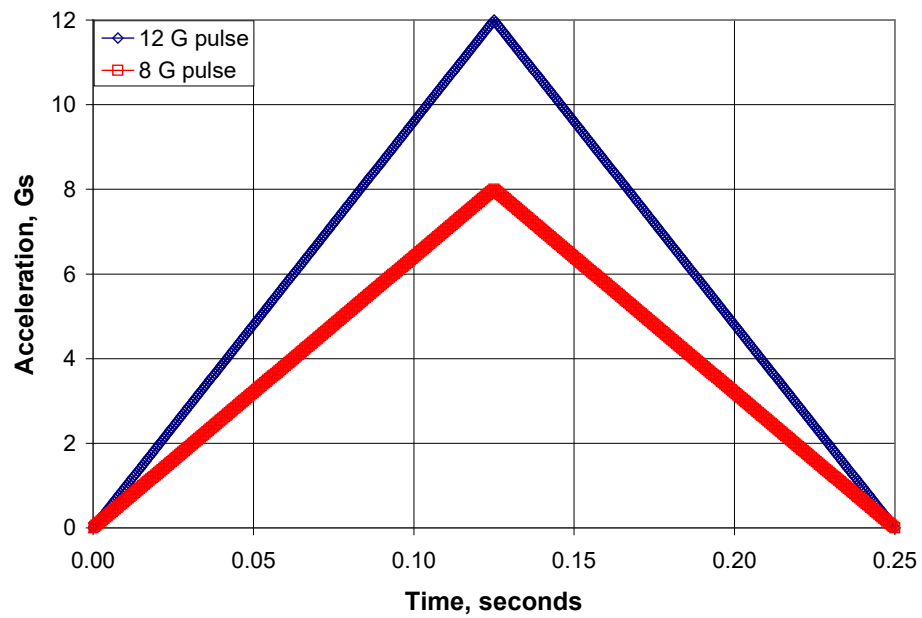
Figure 1. Crash pulses
