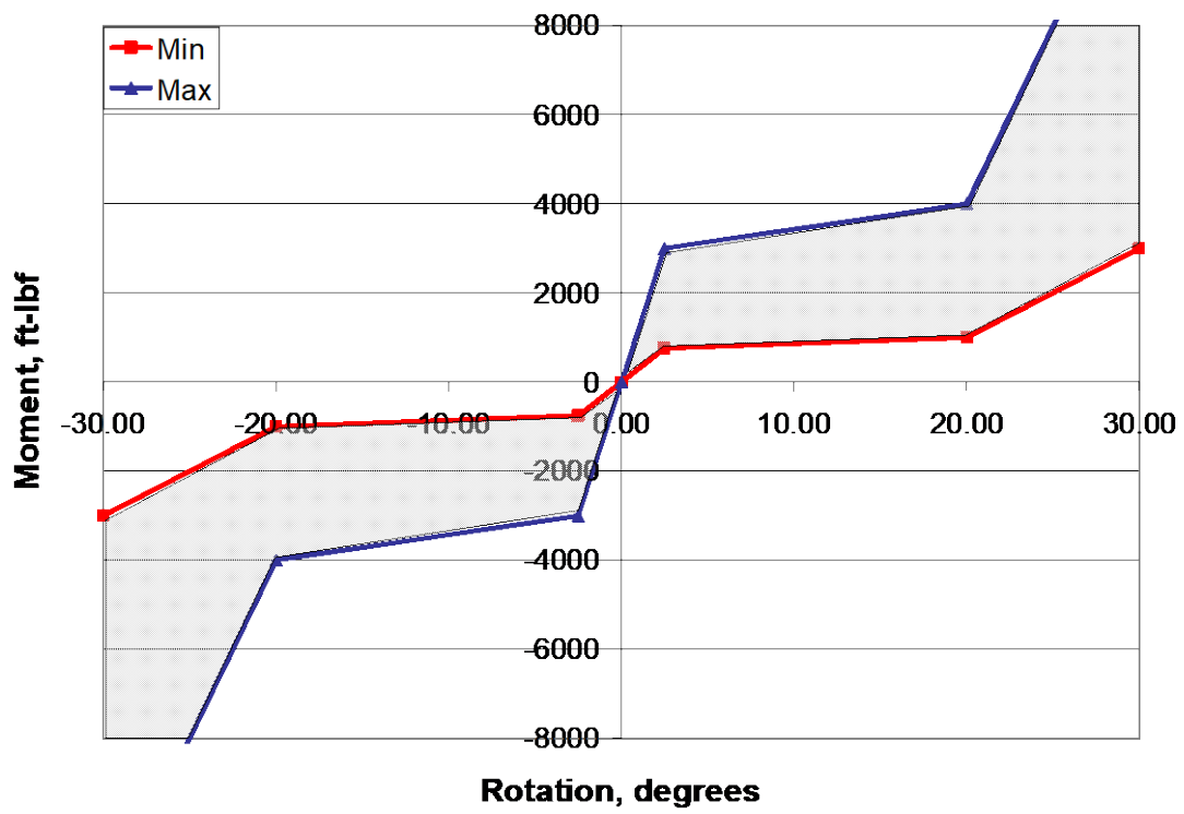
Figure 2. Limits for allowed moment vs. rotation characteristics of seat back
