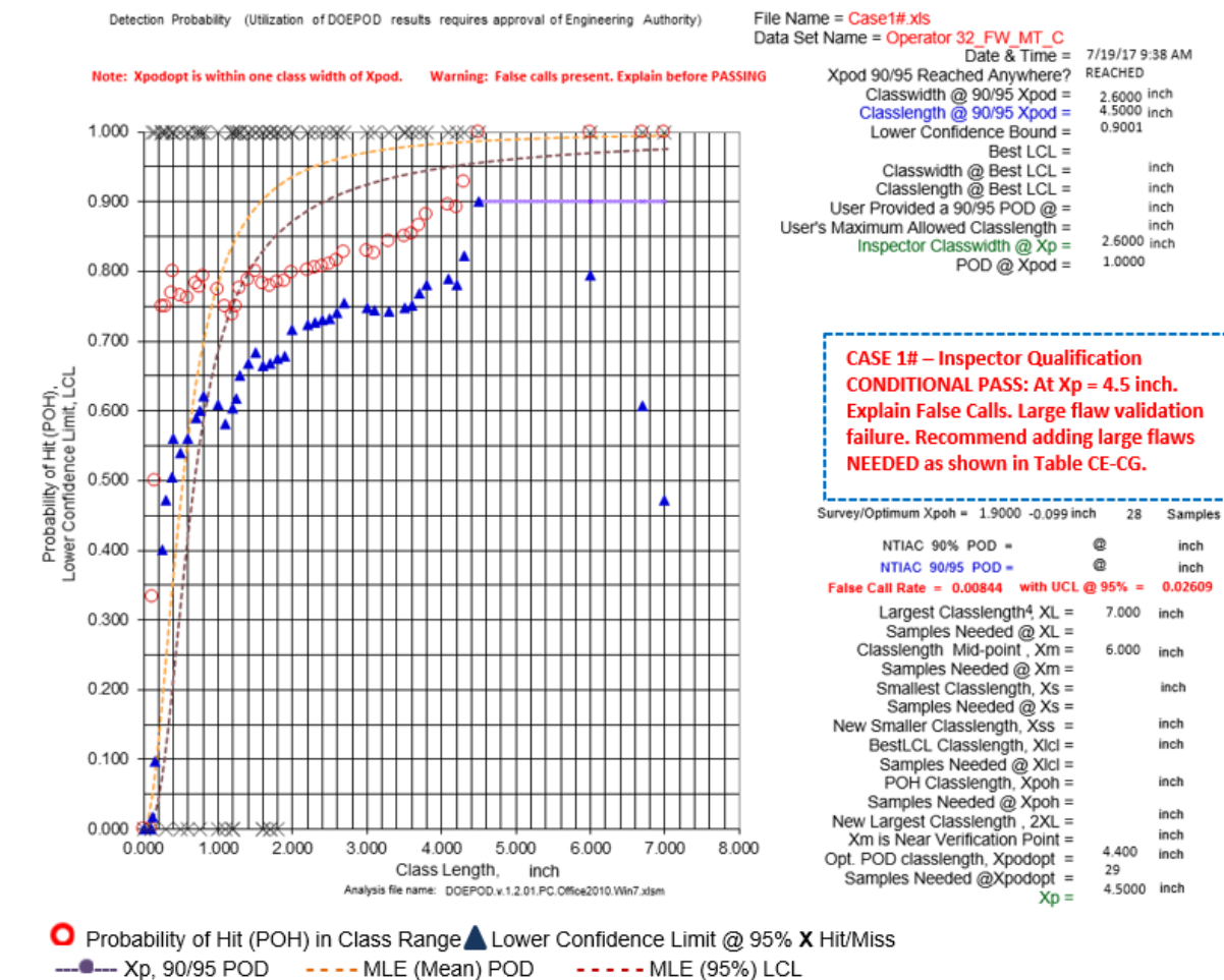
Figure 16. CASE 1# Example of DOEPOD Analysis for Operator 32 (MT with contrast)
