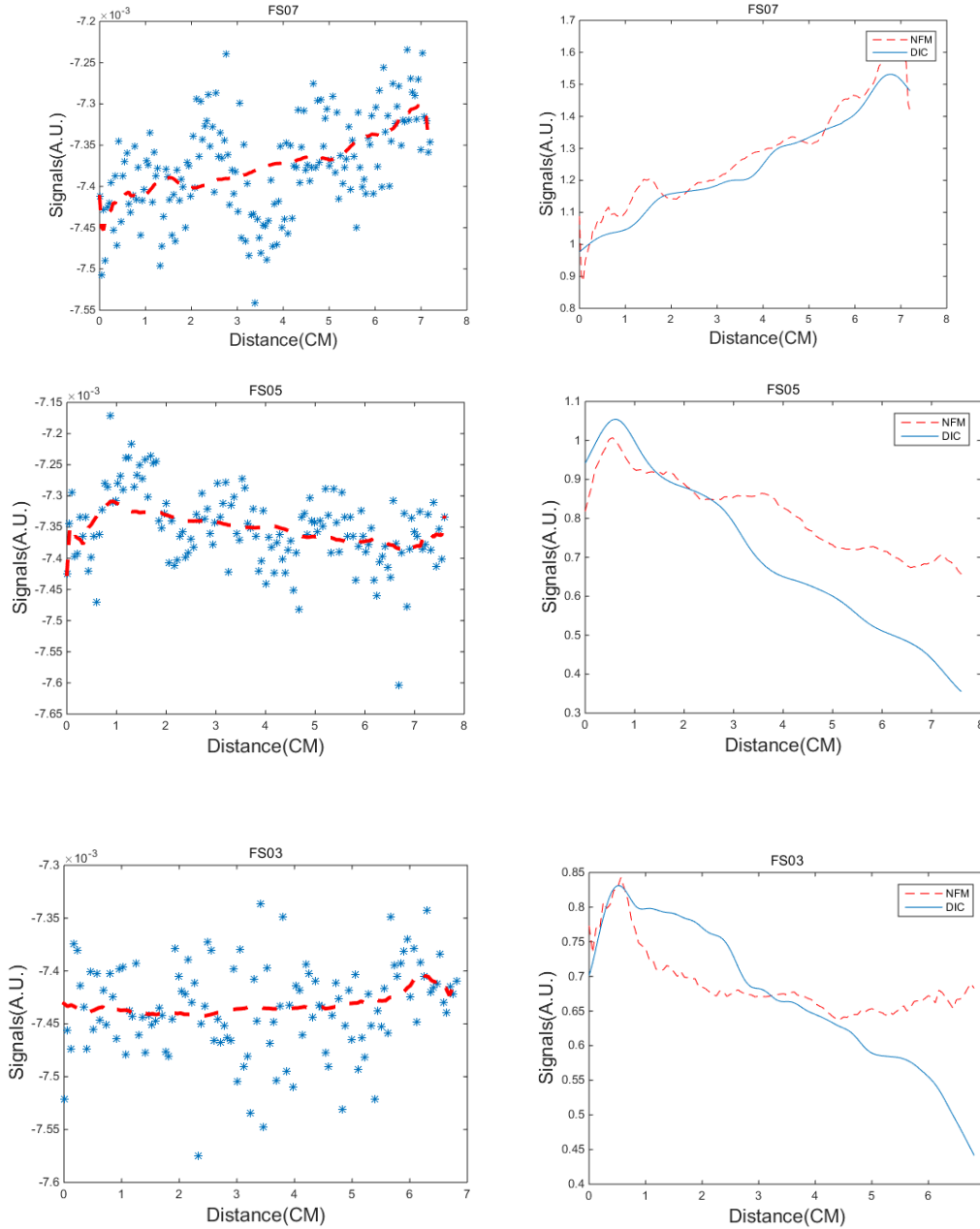
Figure 1-24 scanning results and correlation of the full specimens
