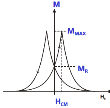
Figure 2-5 Barkhausen noise profile curve
