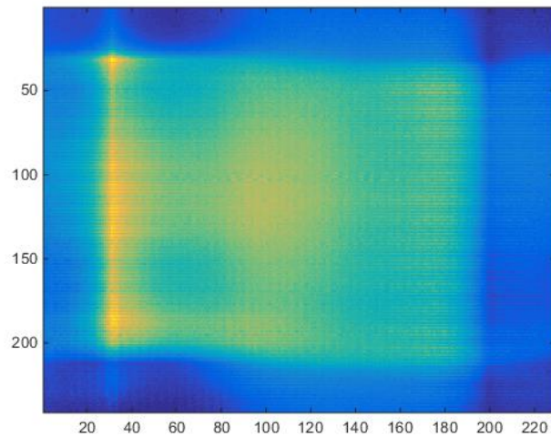
Figure 1-16 deblurred image
