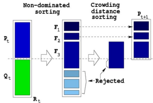
Figure 2-20 NSGAI algorithm
